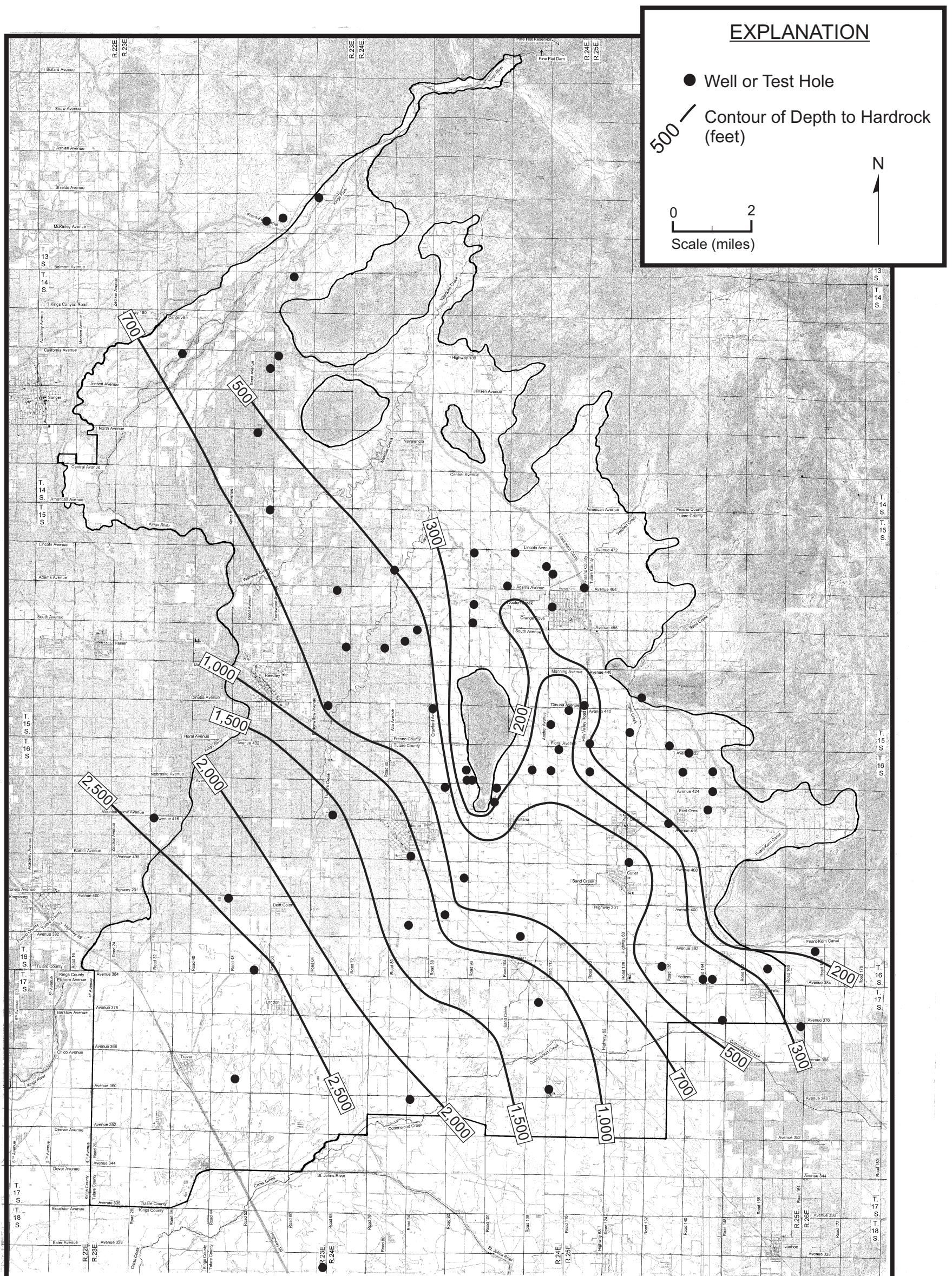
FIGURE 4 - DEFINABLE BOTTOM OF BASIN
