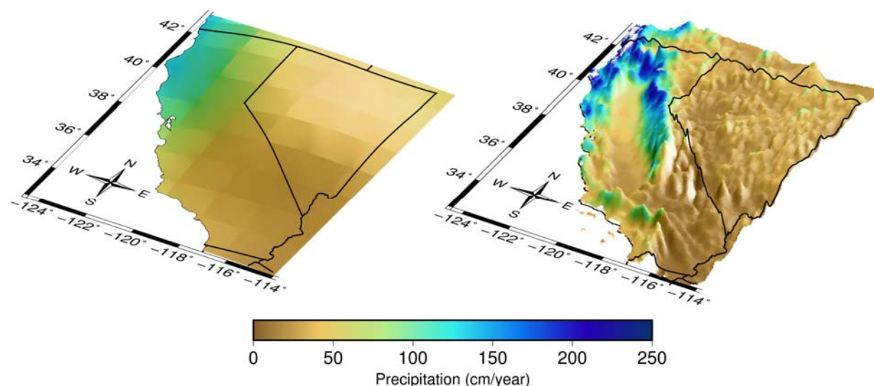
Figure 1. Annual precipitation in California and Nevada (cm; 250 cm is approximately 100 inches) in a global climate model with a resolution of approx. 160 km (100 miles; left), and after using a statistical model to account for the effects of topography at a 6 kilometer (3.6 mile) resolution (right). The global model only has a few grid cells over the entire state of California, so does not resolve the coastal mountain ranges, interior valley, or Sierra Nevada Mountains on the border with Nevada. The precipitation field in the right panel, by contrast, captures the wet conditions on the west slopes of the mountains, and the dry, rain shadow region to the east of the mountains. The vertical scale has been exaggerated for clarity, and by the same amount in both panels.
