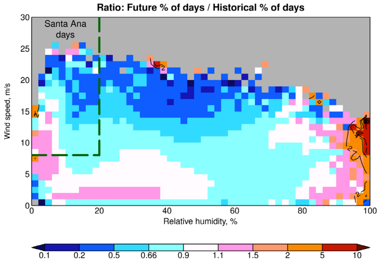
Figure 26. Ratio of the future incidence (% of days) to historical incidence of days in relative humidity-wind speed bins. The future period is 2070-2099, using RCP 8.5. The green box shows the Santa Ana day criterion used here: wind speed \geq 8 m/s, relative humidity \leq 20\% . Computed using the 8 of 10 California GCMs with the requisite data to calculate wind speed.
