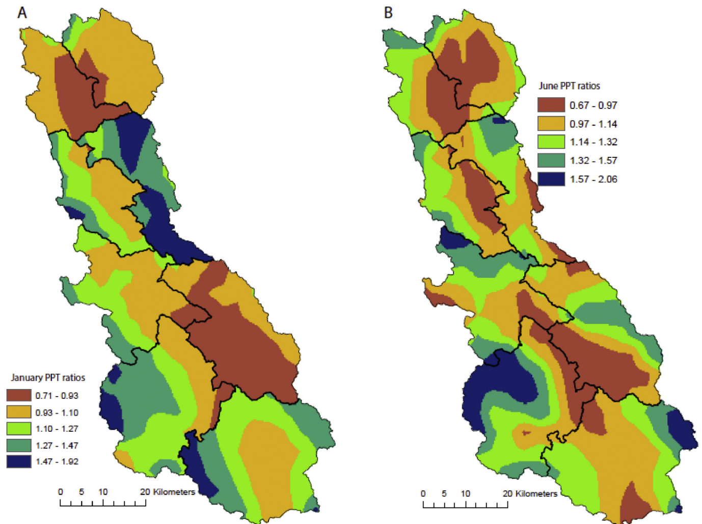
Fig. 10. Precipitation factors for A) January, and B) June calculated from monthly average PRISM values and daily precipitation values measured at climate stations located within the watershed. Nine precipitation stations and respective zones were used in this example. Precipitation factors are calculated for each month.
