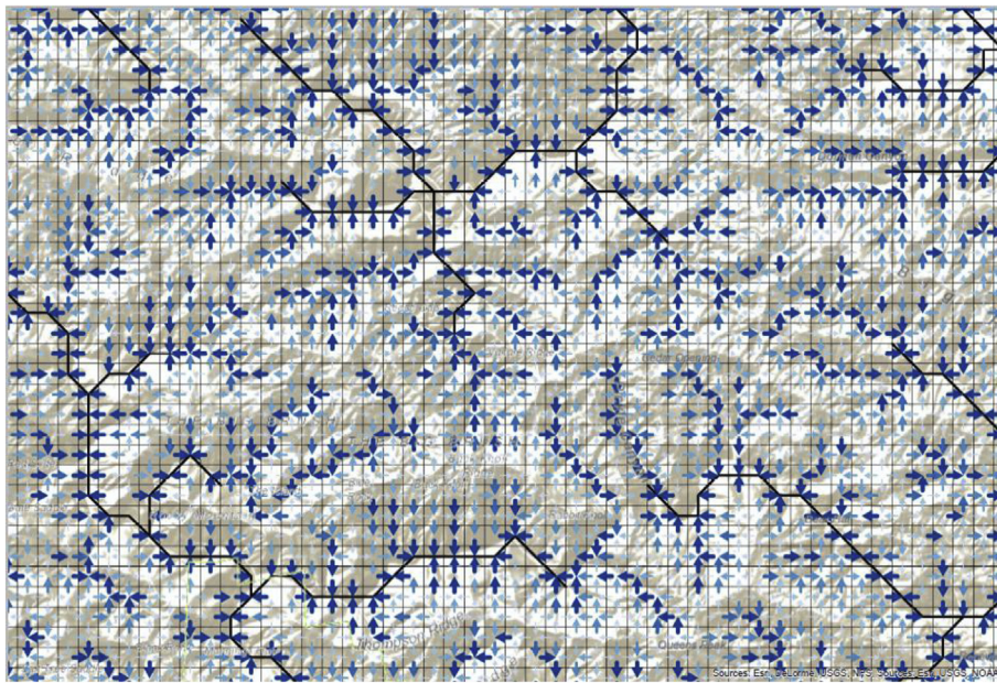
Fig. 7. Inset from Russian River model showing HRUs, streams, and cascading flow directions created by the Cascade Routing Tool (CRT). Cascade parameters generated by CRT are used for distributed overland flow and shallow subsurface flow routing in GSFLOW (Henson et al., 2013). Darker colored arrows indicate greater drainage area accumulation.
