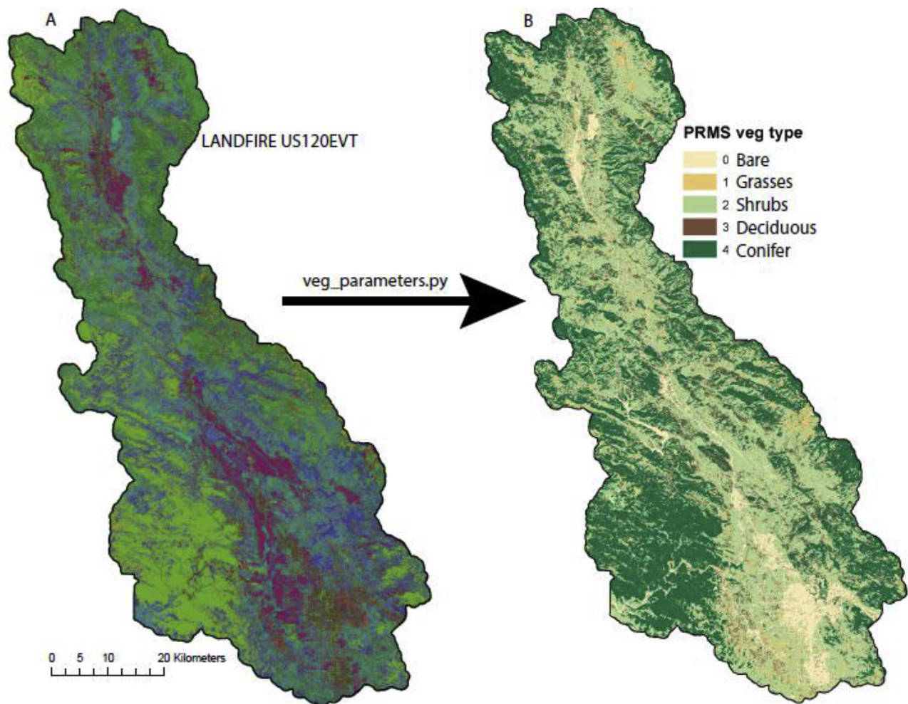
Fig. 8. Map showing vegetation type remapped from: A) LANDFIRE existing vegetation type (US120EVT), and to B) PRMS values. Vegetation type is just one of the several vegetation based parameters that veg_parameters.py converts to PRMS values for each HRU.
