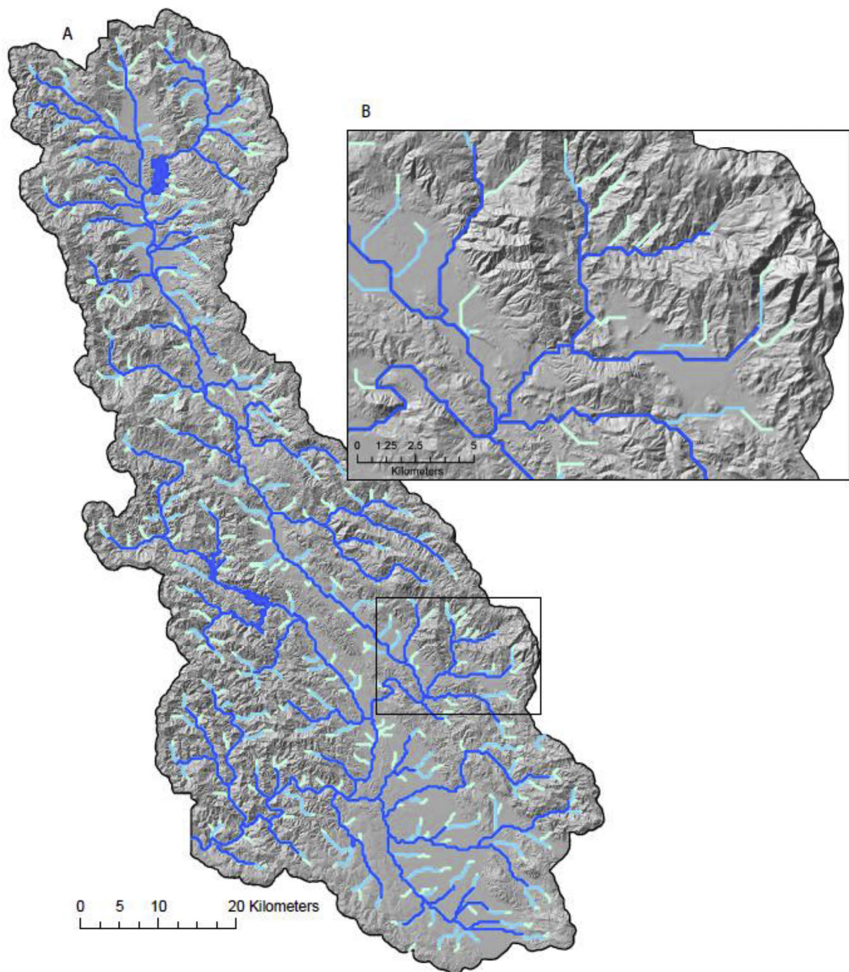
Fig. 4. Stream networks generated with different flow accumulation and flow length threshold settings; A) Russian River watershed, and B) inset of a sub-basin showing different stream resolutions. The darkest blue lines (streams_100_10) show a network with a flow accumulation threshold of 100 and flow length threshold of 10. HRUs with flow accumulation and flow lengths smaller than the specified threshold will not contain streams. The lighter blue lines show the levels of detail that can be obtained by decreasing the flow accumulation and stream length thresholds (streams_50_5 and streams_30_3, respectively). These thresholds are site specific and depend on the resolution and purpose of the model. (For interpretation of the references to color in this figure legend, the reader is referred to the Web version of this article.)
