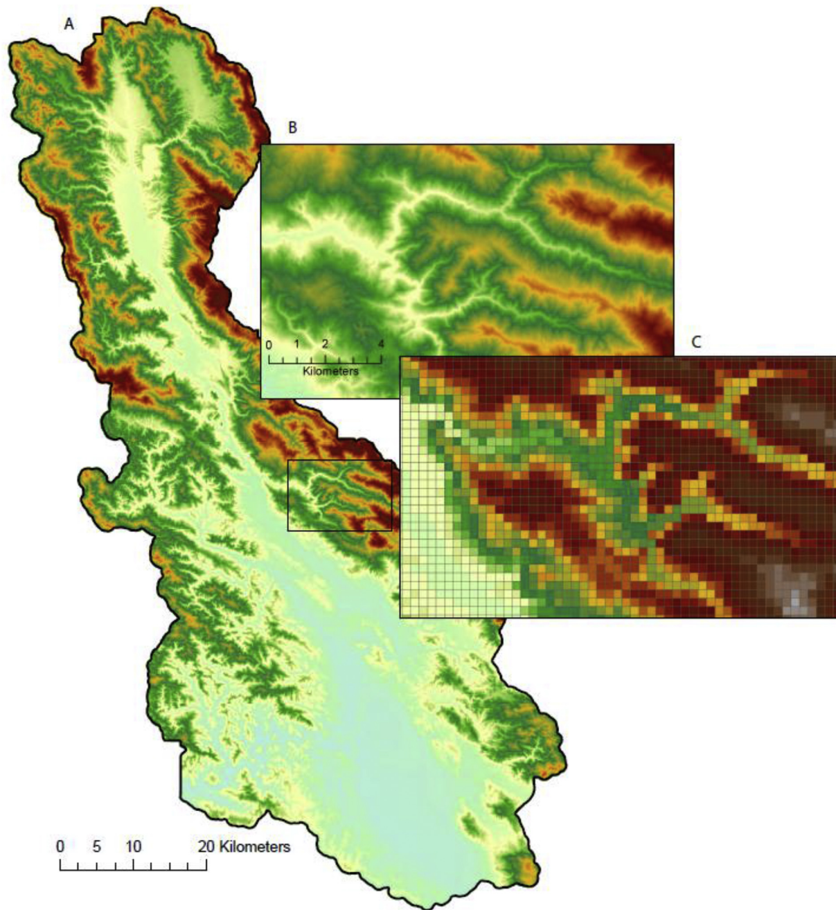
Fig. 3. Maps showing: A) Original 10 m DEM, clipped to the Russian River watershed, B) inset at the original DEM scale, and C) inset of the 300 m DEM re-sampled for the model grid.
