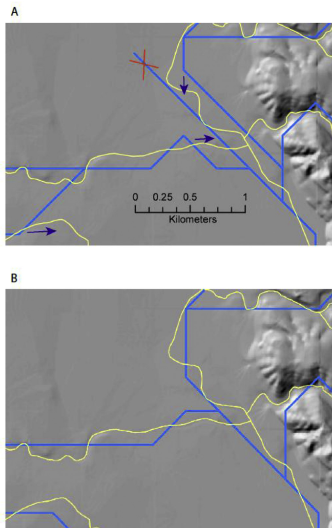
Fig. 5. Gsflow-Arcpy provides the user with the option to make manual adjustments to the DEM_ADJ values in the HRU parameter shapefile attribute table to guide the streams in certain areas, such as flat regions or drainages that are very close to each other, potentially causing a segment to ‘jump’ drainages: A) an erroneous segment (marked with a red X), and the directions (blue arrows) of the desired stream paths; and B) the resulting flow paths after re-running dem_2_streams.py with the adjusted elevations. The amount of manual adjustments is completely up to the user, as some may choose to use the CRT fill values and move on, while others may want to fine tune their stream network beyond the capability of the scripts. (For interpretation of the references to color in this figure legend, the reader is referred to the Web version of this article.)
