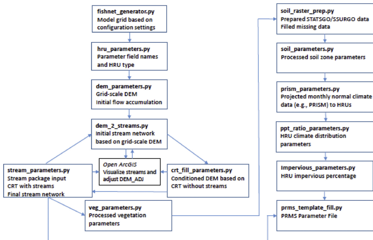
Fig. 1. Diagram illustrating the process flow for Gsflow-Arcpy and the 13 Python scripts that carry out the automated procedure for developing GSFLOW input datasets. The Cascade Routing Tool (CRT; Henson et al., 2013) is used by Gsflow-Arcpy.
