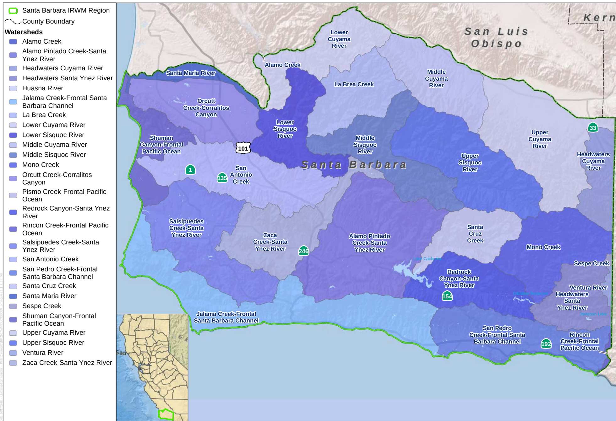
FIGURE 2.7 Watersheds
