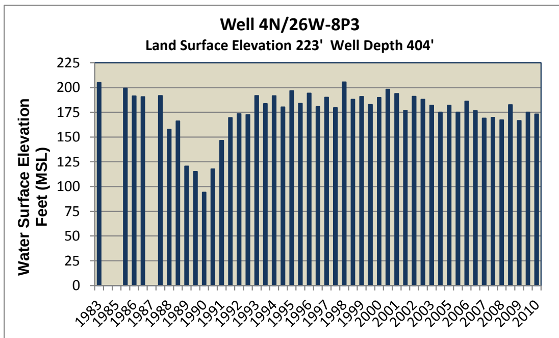
Figure 17: Hydrograph for State Well 4N/26W-8P3
