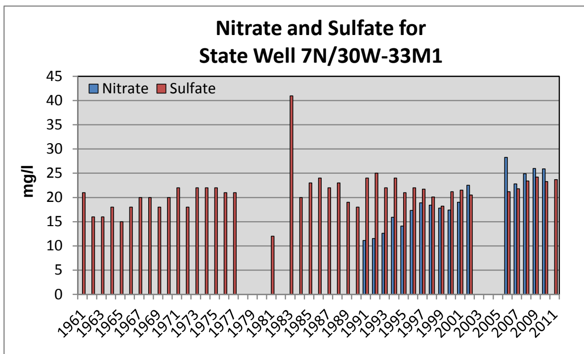
Figure 30: Nitrate and Sulfate for State Well 7N/30W-33M1
