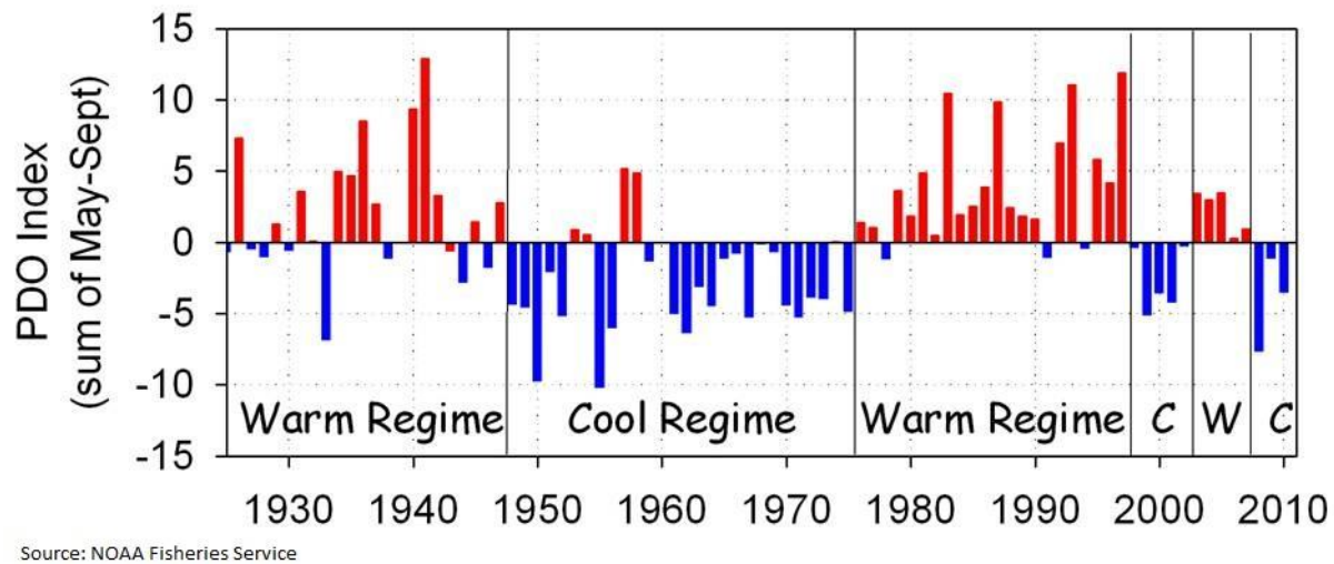
Figure 10: Historic PDO Index
