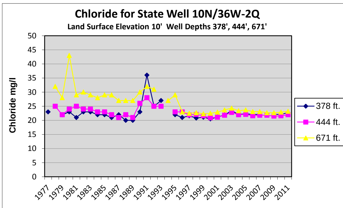
Figure 45: Chloride Concentration for State Wells 10N/36-2Q
