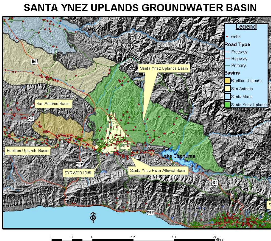
Figure 26: Santa Ynez Uplands Groundwater Basin
