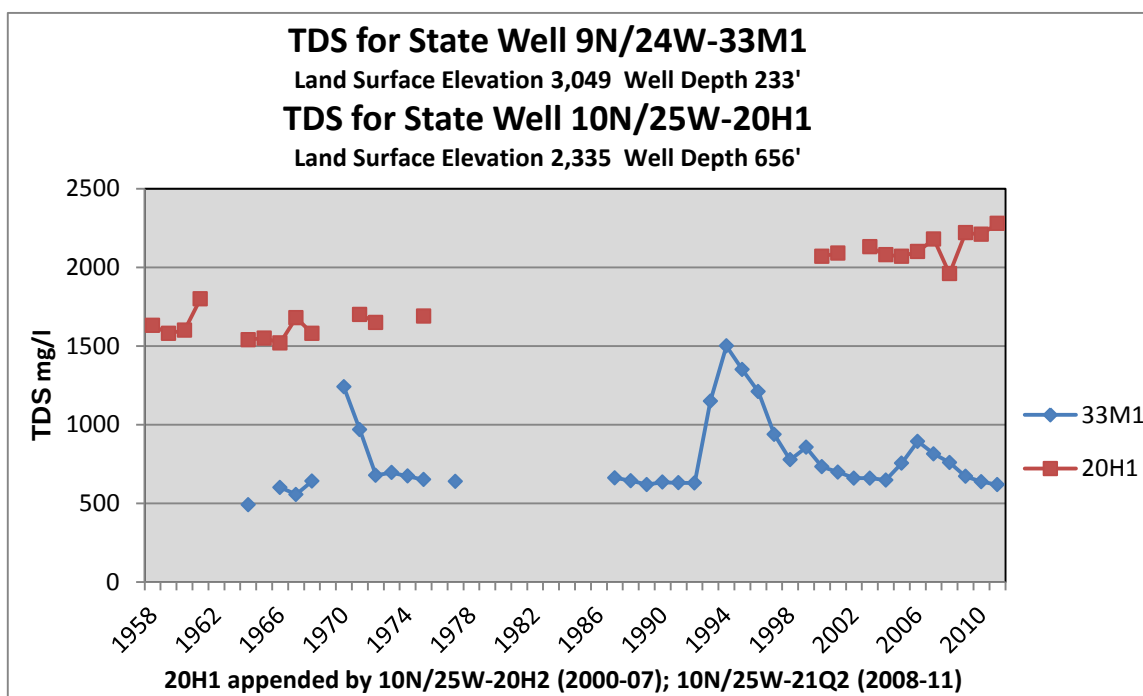
Figure 50: TDS for State Wells 9N/24W-33M1 and 10N/25W-20H1
