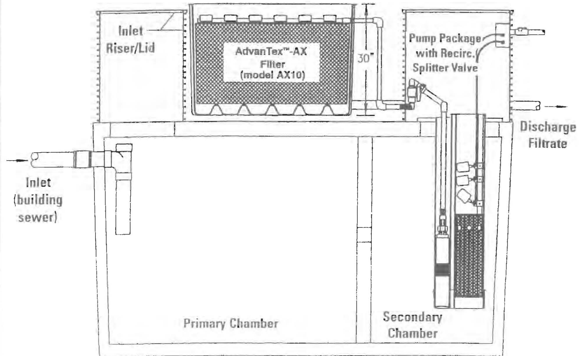
TEXTILE FILTER
