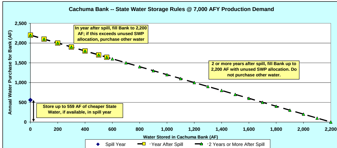
Figure 7. Rule curve for purchase of water for Cachuma Bank at production demand level of 7,000 AFY.
