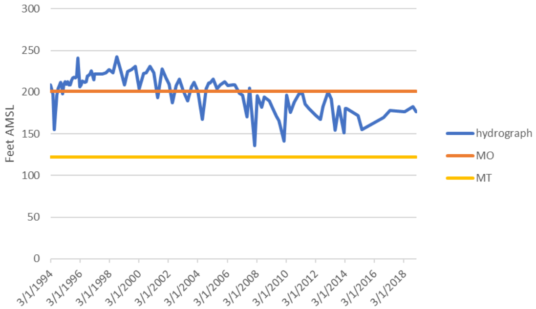
Figure 5-11f. DMW 07 Hydrographs [1993 – 2018], MO, and MT
