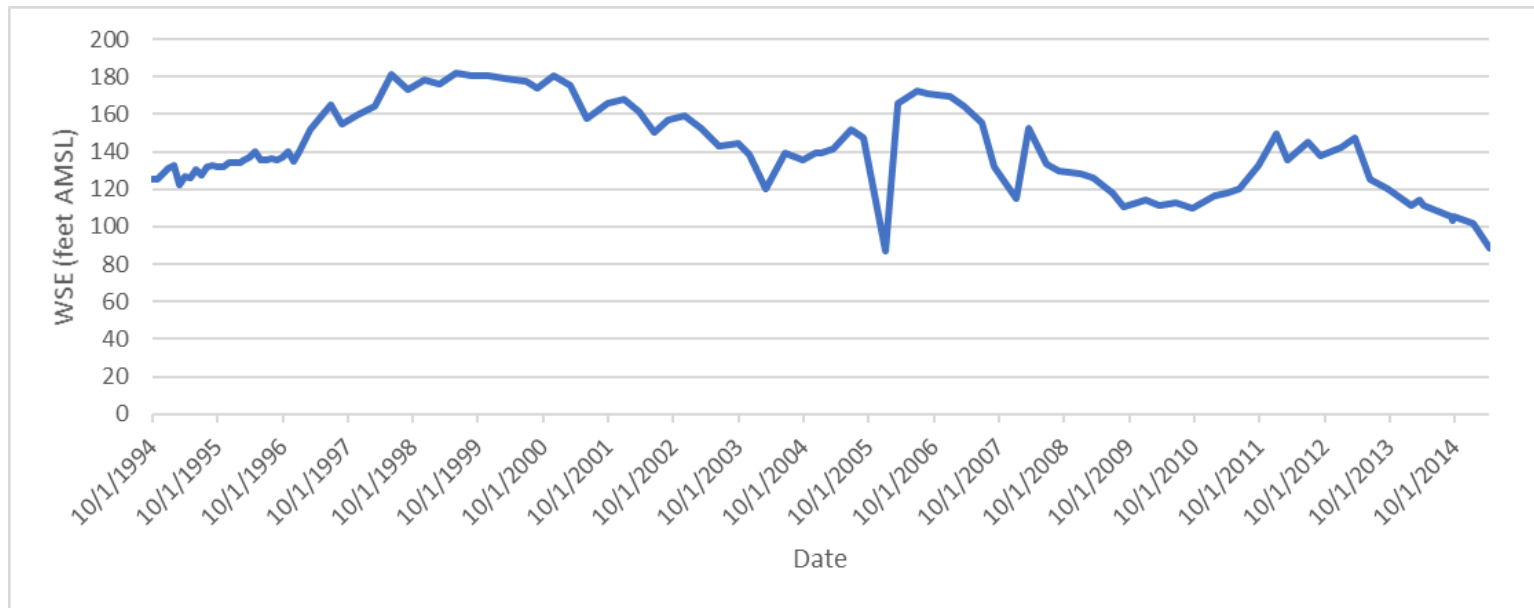
Figure 2-26k. DMW12b Hydrograph
