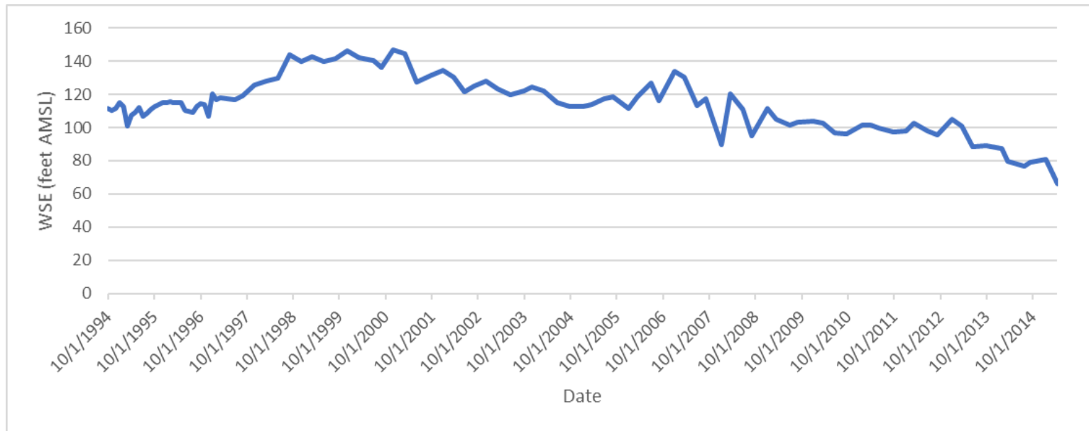
Figure 2-26i. DMW10b Hydrograph
