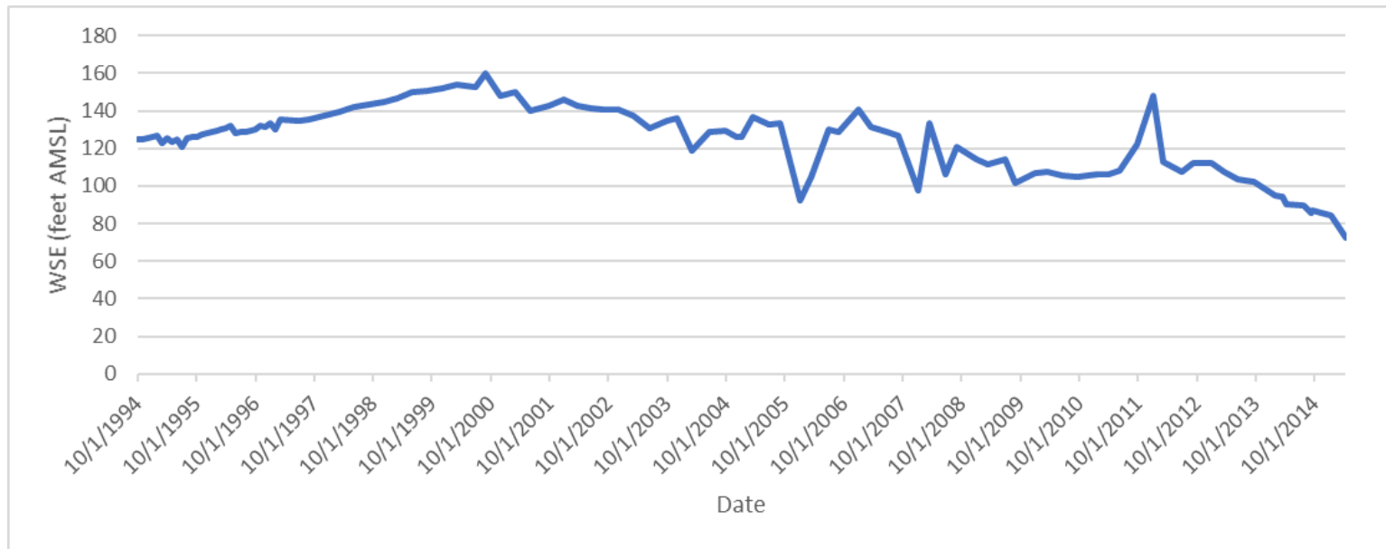
Figure 2-26j. DMW12a Hydrograph
