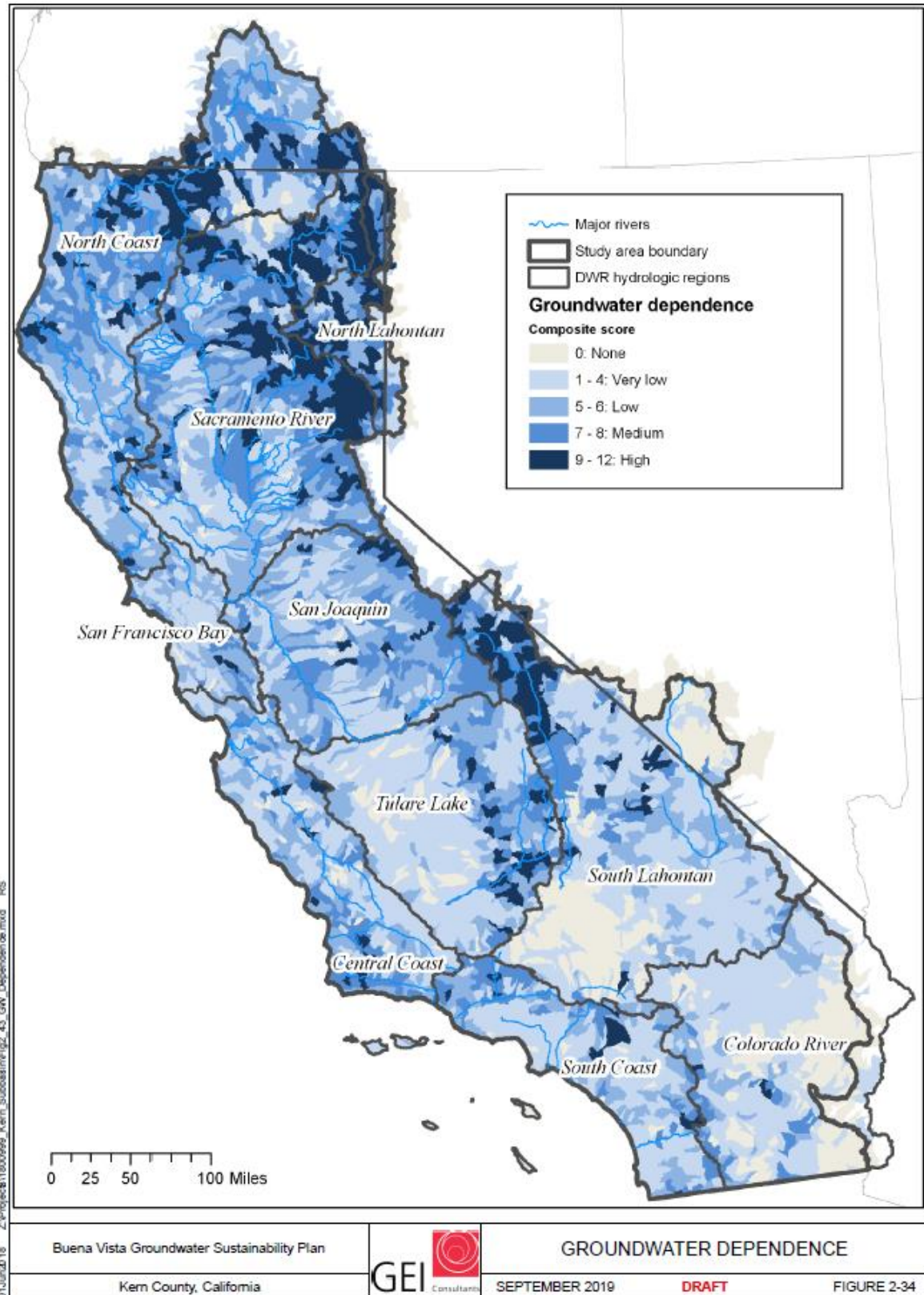
Figure 2-34. Groundwater Dependence
