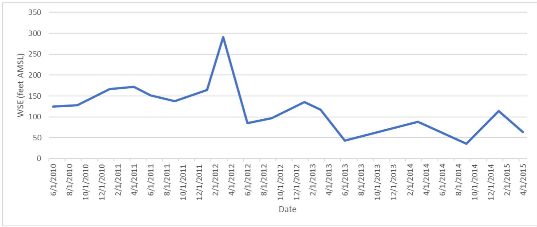
Figure 5-20. Hydrograph of Well MO2
