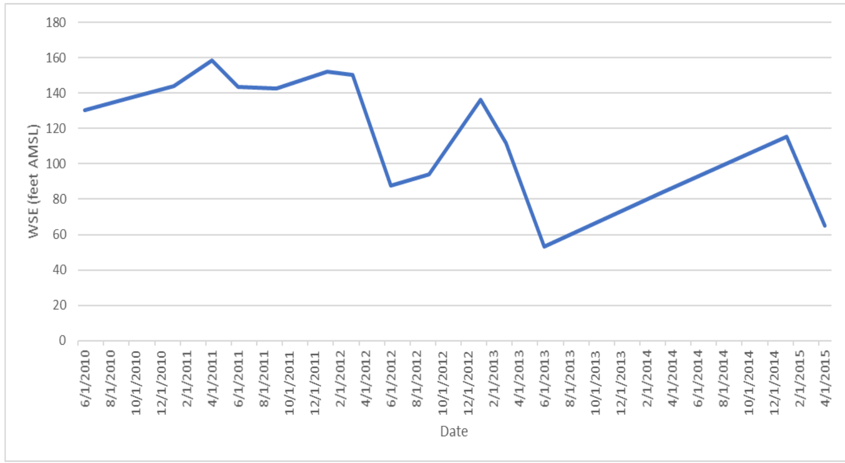
Figure 5-19. Hydrograph of Well MO1
