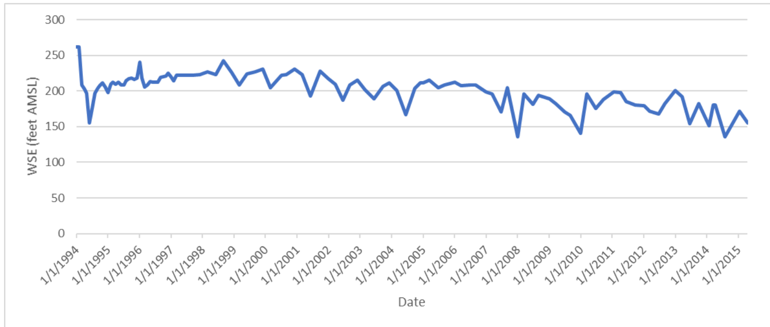
Figure 2-26f. DMW07 Hydrograph
