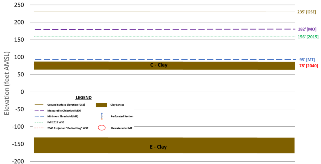
Figure 5-10b. Minimum Threshold and Measurable Objective Setting for DMW 02
