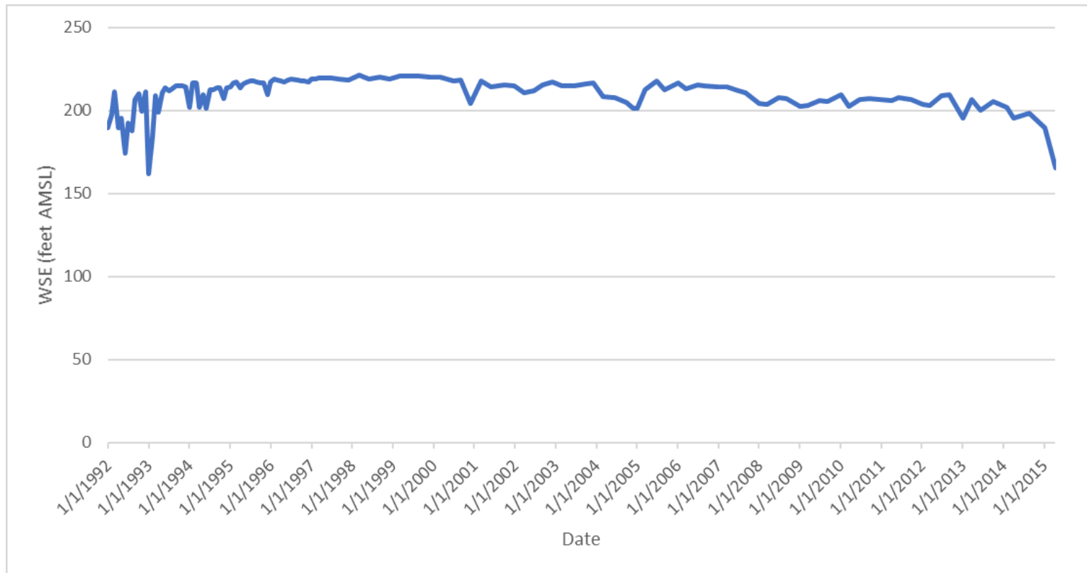
Figure 2-26a. DMW01 Hydrograph
