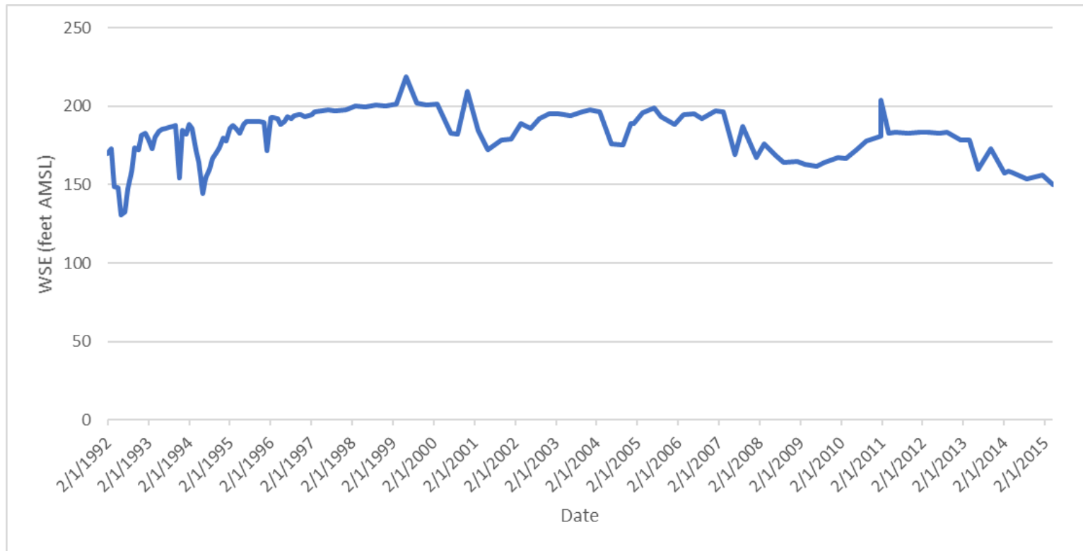
Figure 2-26b. DMW02 Hydrograph
