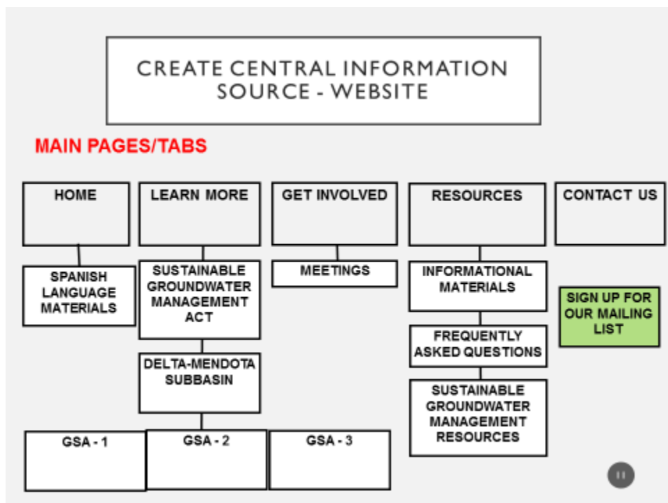
Figure 10. Website Structure
