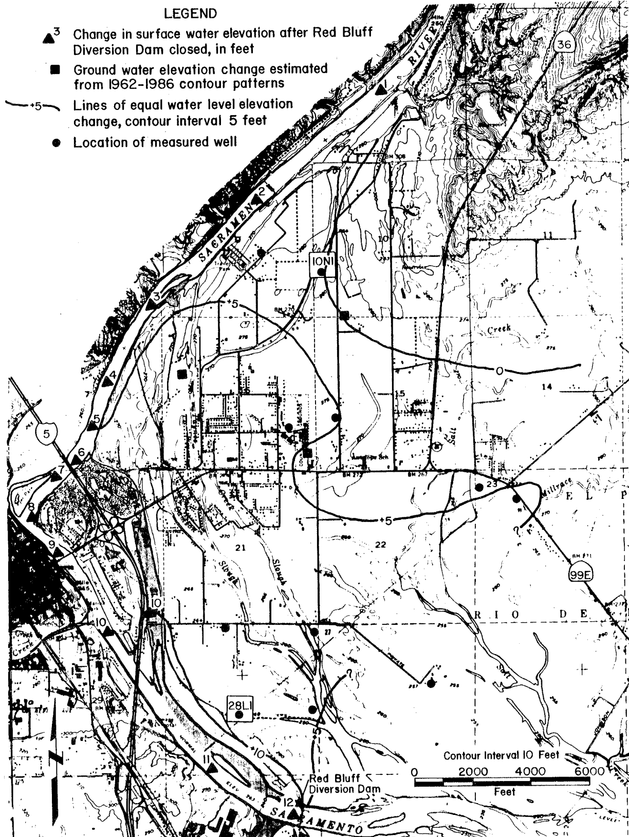
Antelope Ground Water Study Change in Water Level Elevation Spring 1962 to 1986
