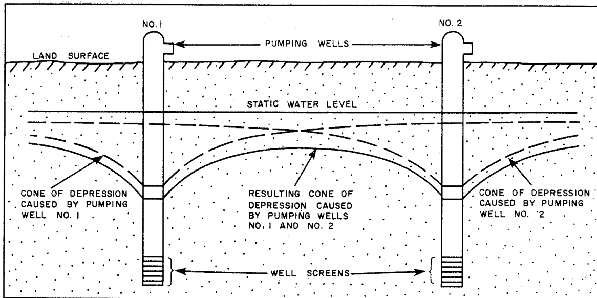
Figure 9 Effects of interference between two pumping wells.
