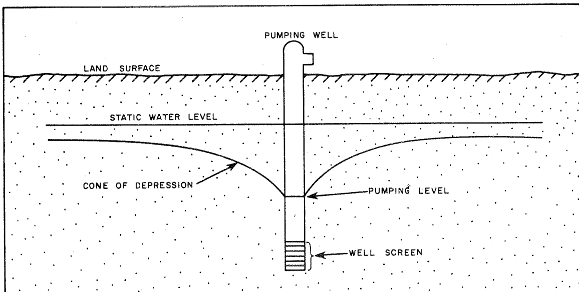
Figure 8 Cone of depression caused by pumping wells.
