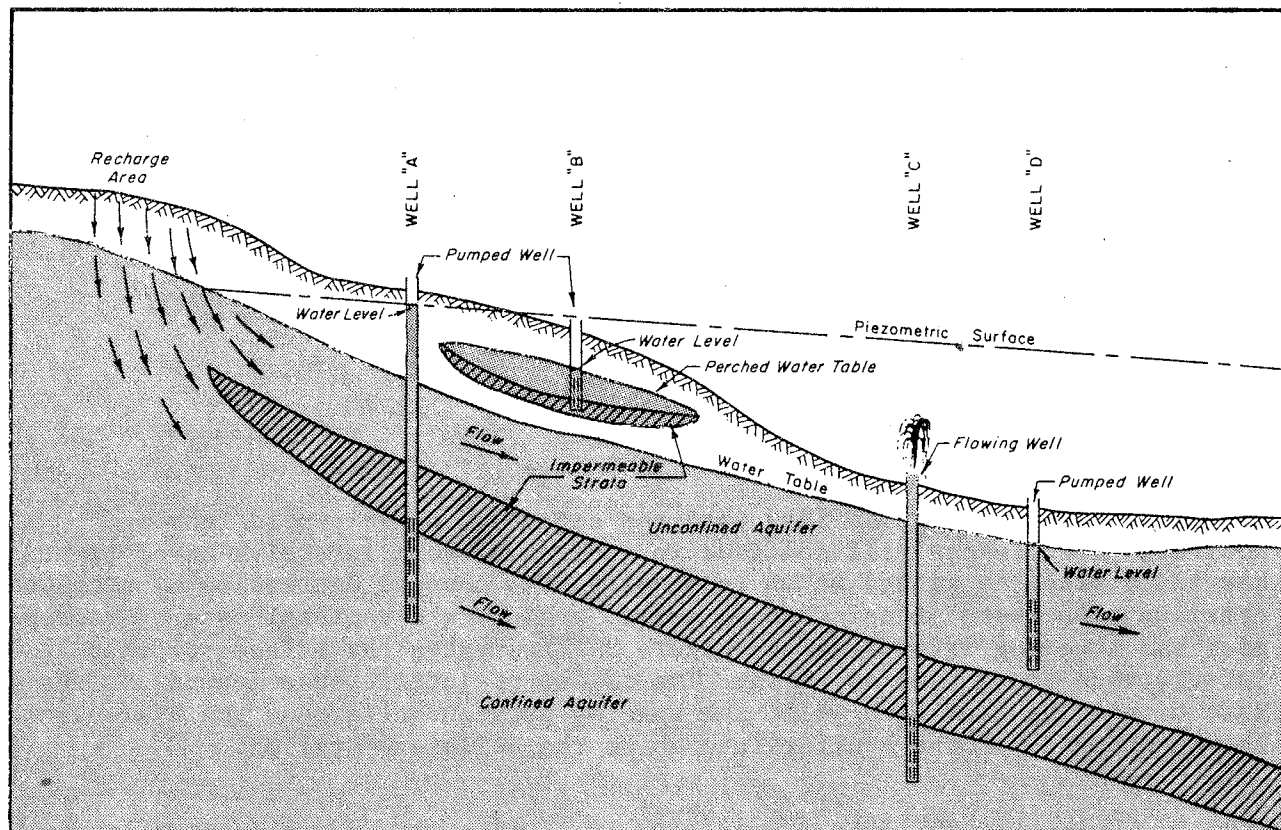
Figure 7 Unconfined and Confined Ground Water.
