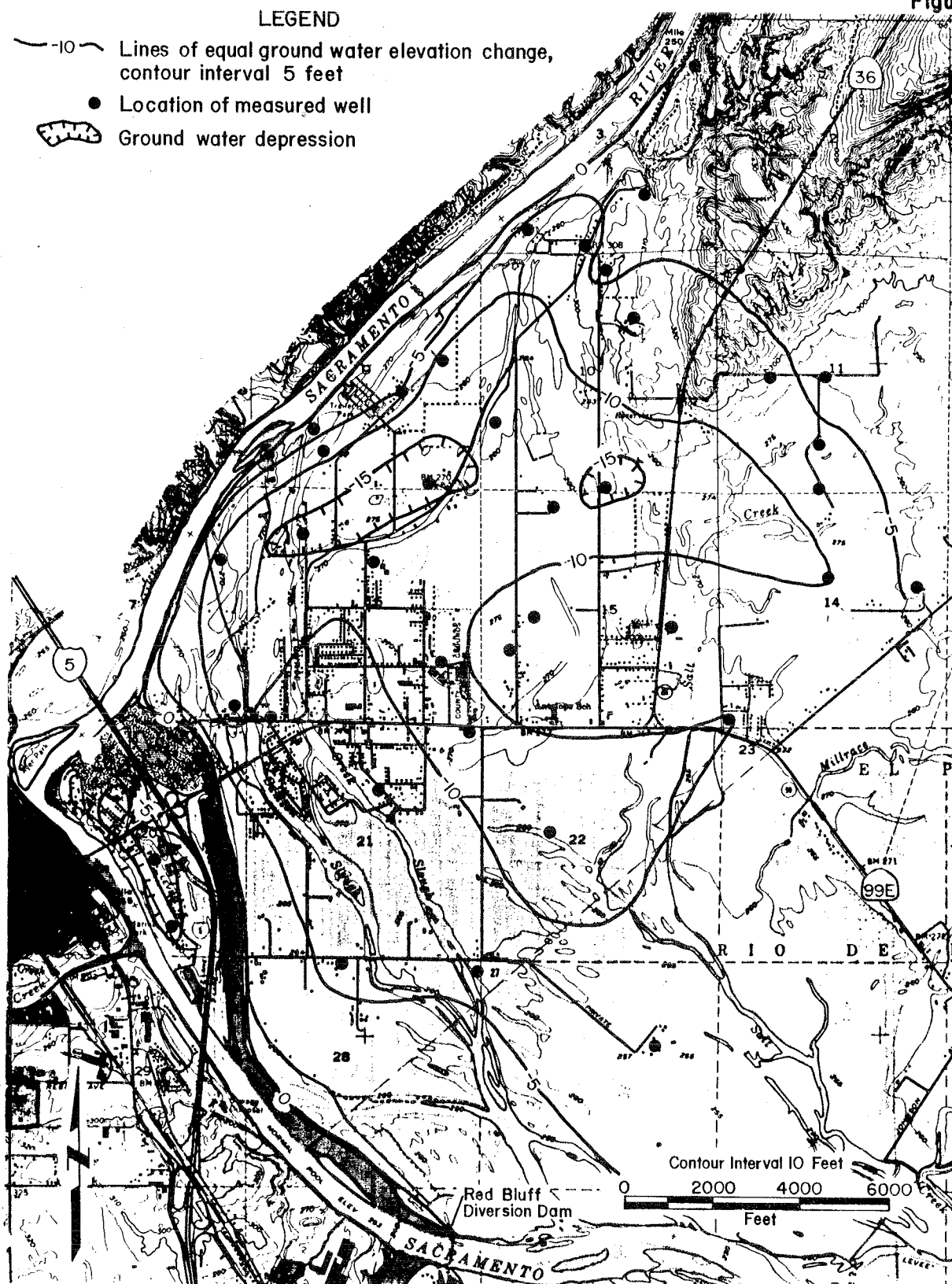
Antelope Ground Water Study Change in Water Level Elevation, Spring to Fall 1986
