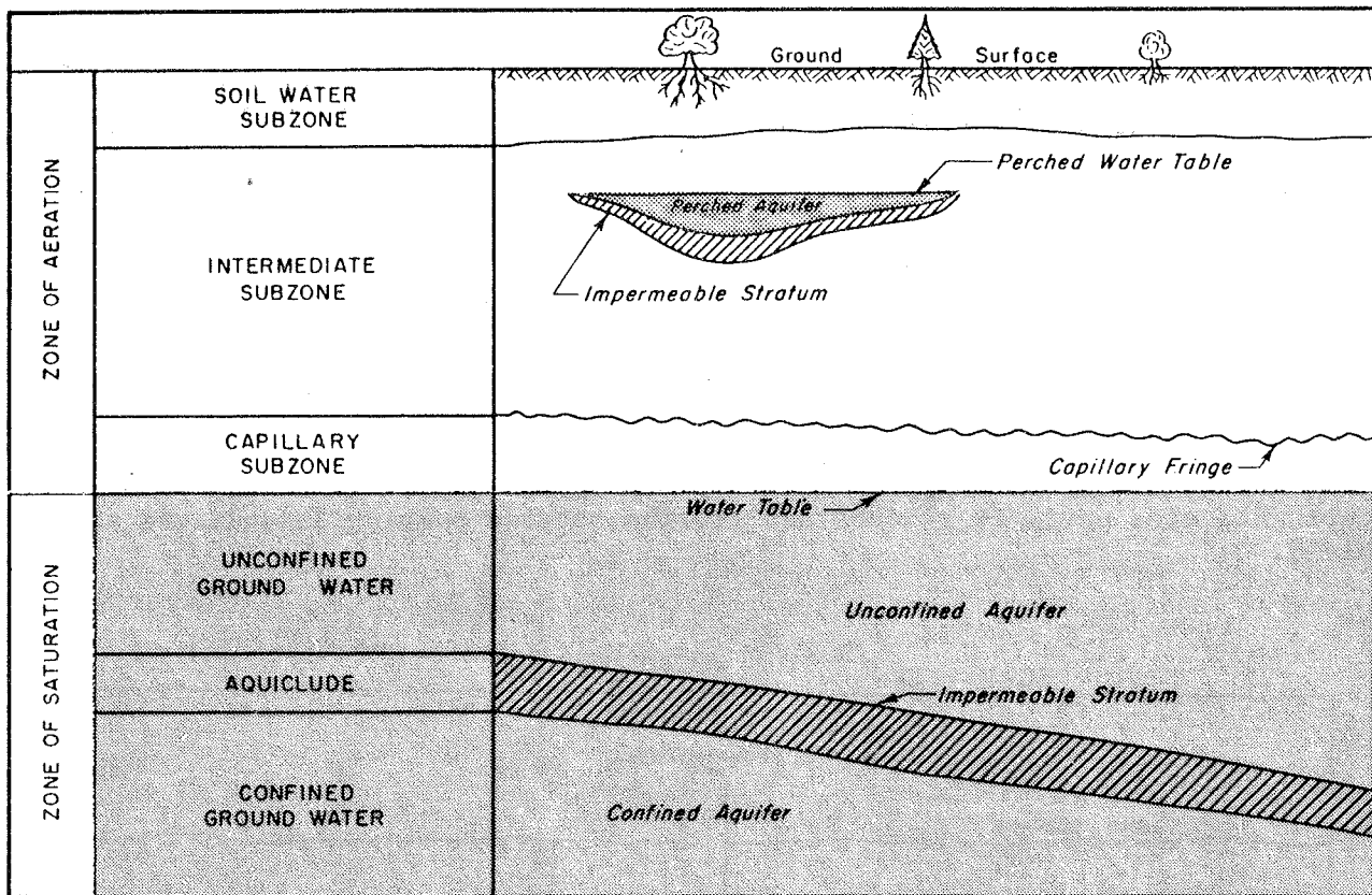
Figure 6 Occurrences of Ground Water.
