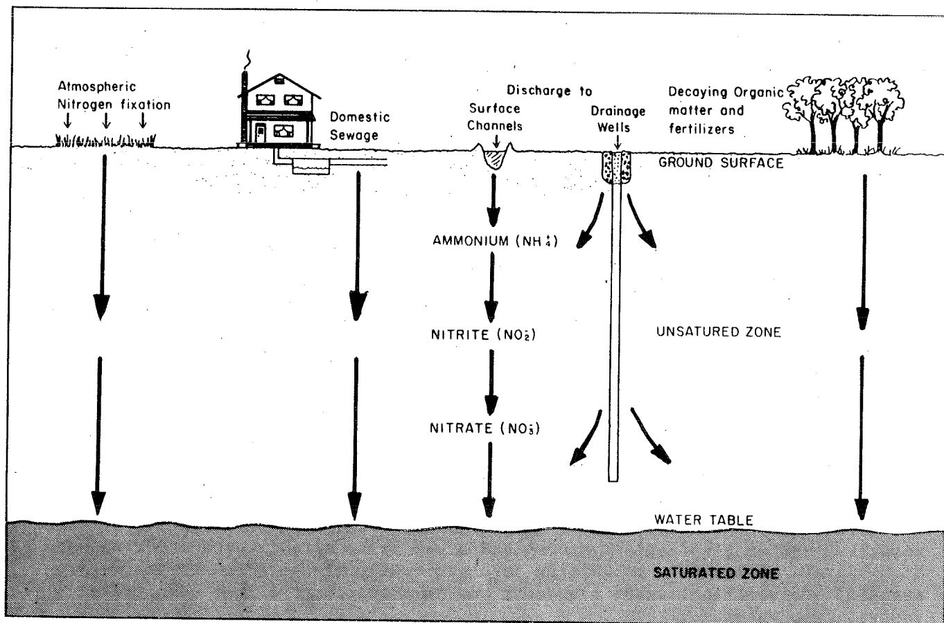
Figure 22 Nitrate sources to ground water.
