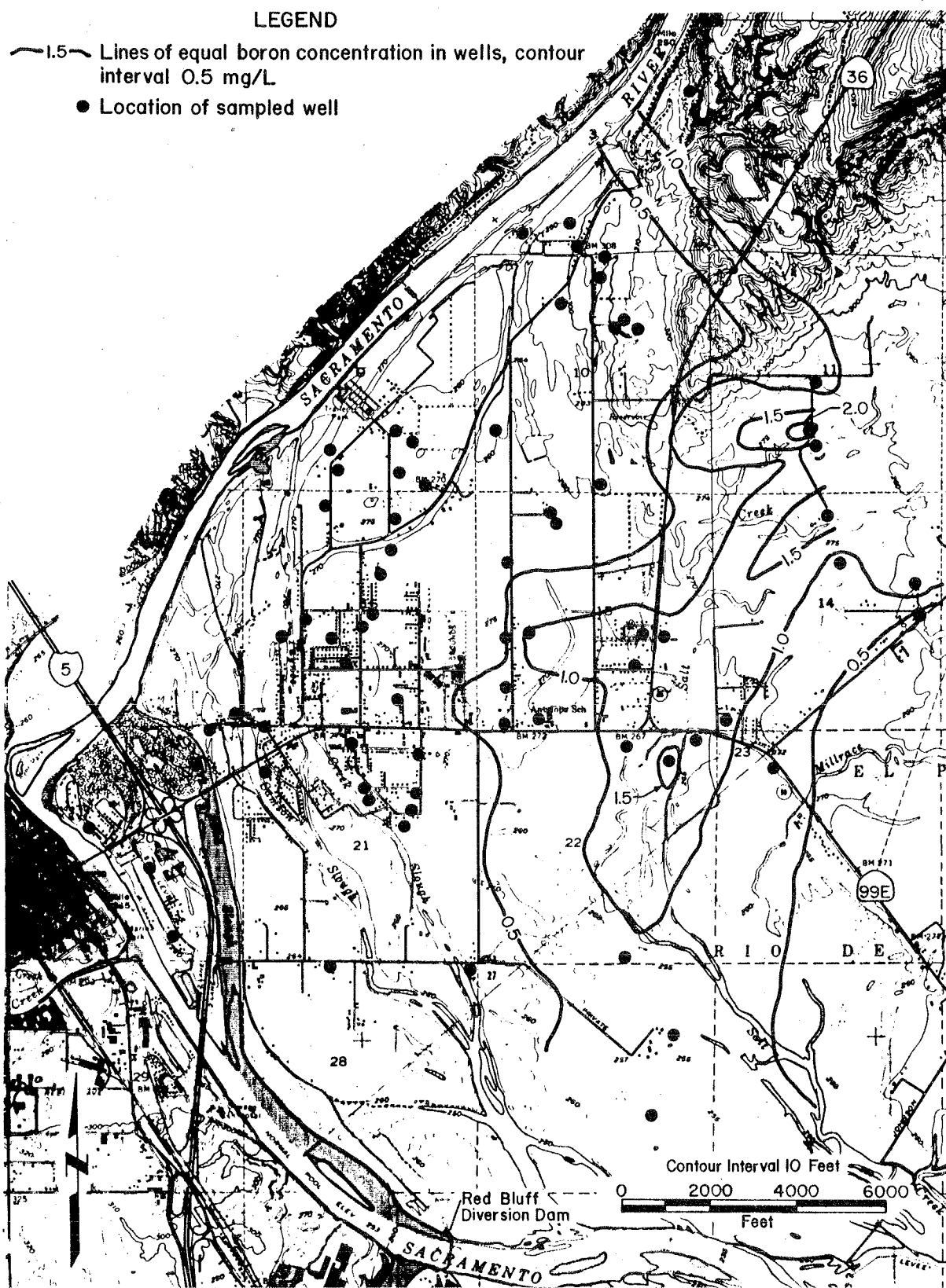
Antelope Ground Water Study Distribution of Boron
