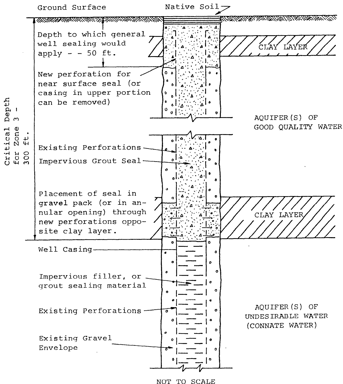
FIGURE 4. TYPICAL SEALING FEATURES OF DESTROYED WELLS FOR ZONE 3 (for gravel packed wells)
