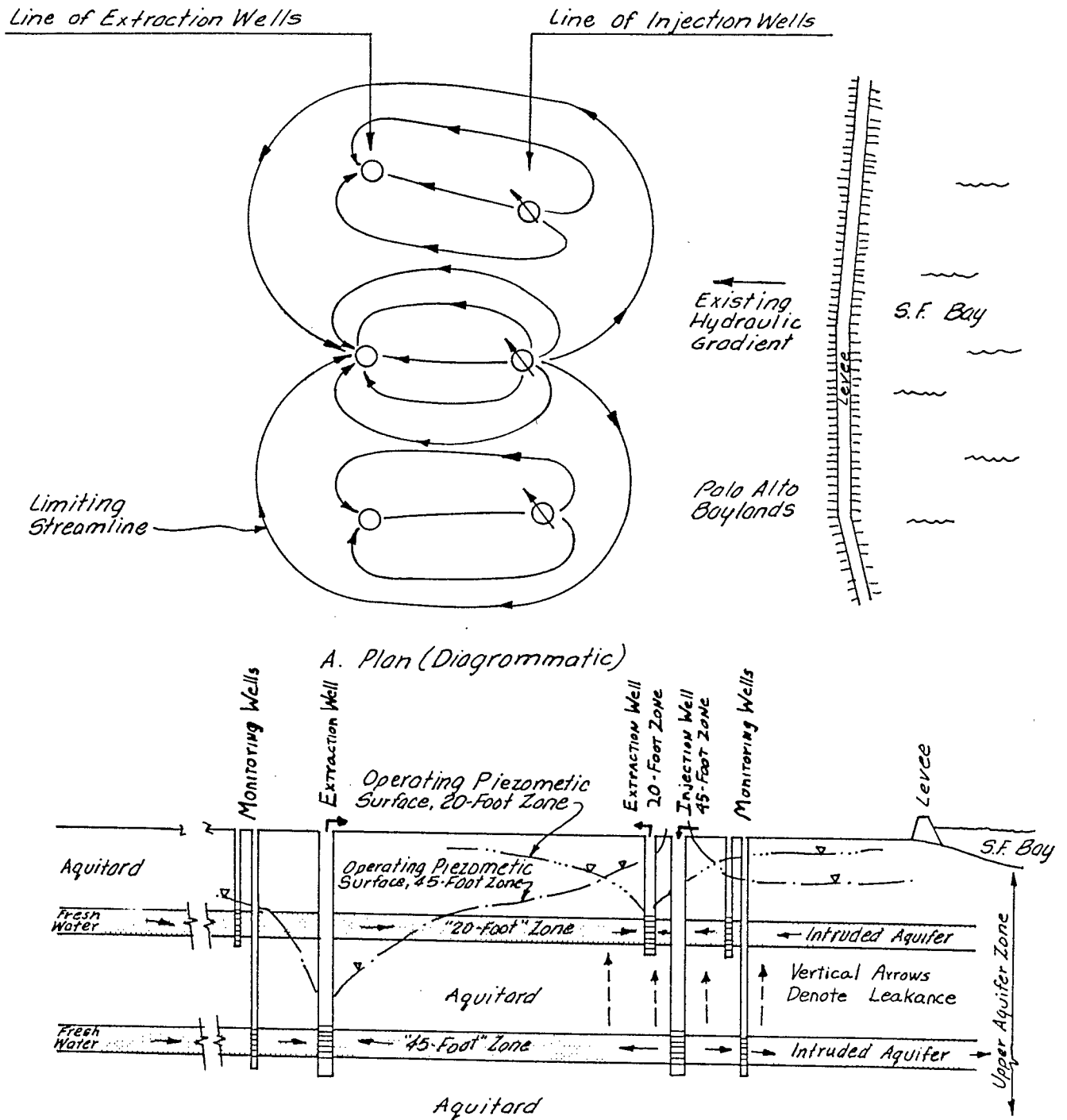
B. Profile (diagrammatic, enlarged from general scale of plan)
