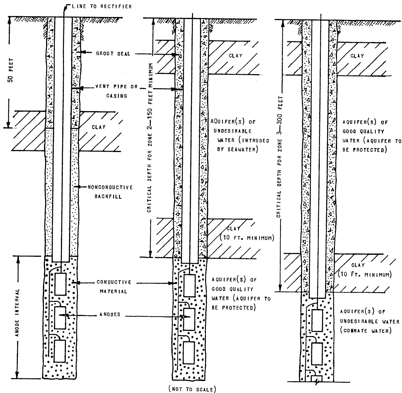
A. GENERAL REQUIREMENT, ZONE 1.
