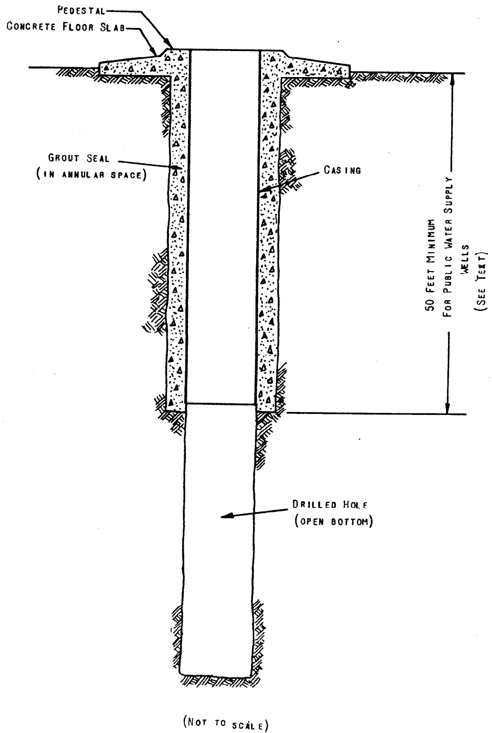
FIGURE 5. EXAMPLE OF SEALING UPPER ANNULAR SPACE WELL IN BEDROCK FORMATION
