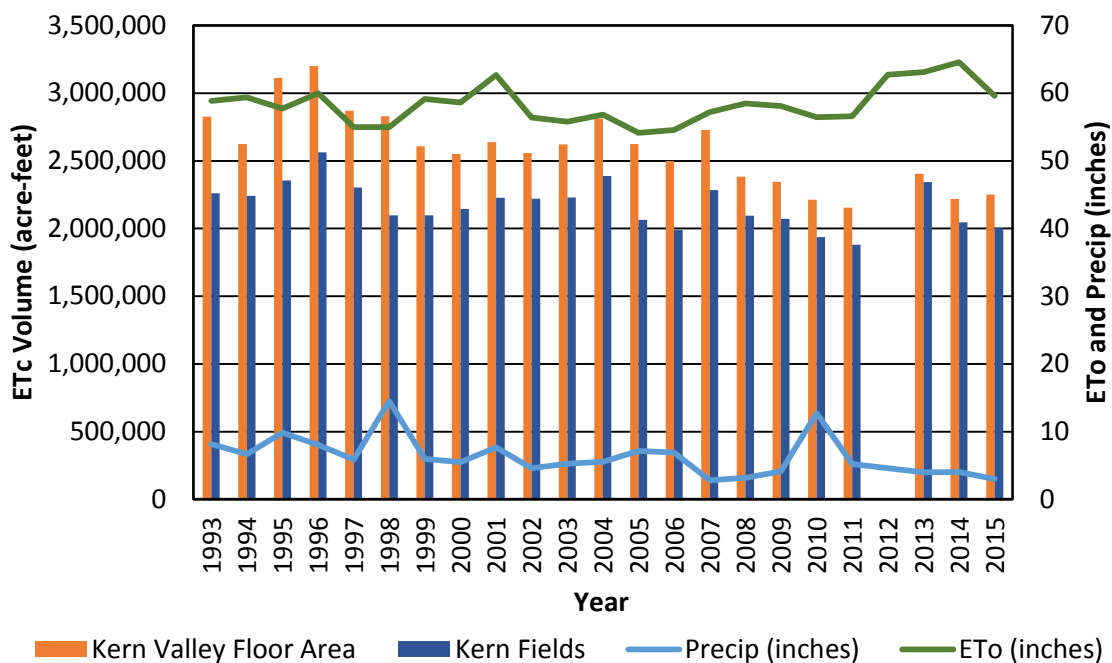
Figure 10. Annual volume of ET_c for the Kern County Valley floor and within fields in Kern County. Grass reference ET_o and precipitation depths are shown for each year as a reference.
