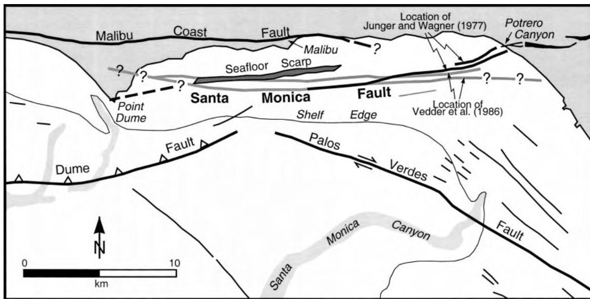
Figure 4. Map of active surficial faults along the Malibu Coast. Note differing locations for offshore Santa Monica fault shown by Junger and Wagner (1977) and Vedder et al. (1986), as well as 10-m-high, south-facing submarine scarp south of Malibu. Thick lines denote faults discussed in the text. Thinner lines show other faults that exhibit either Holocene or Pleistocene activity. Stipple denotes submarine canyons. Data are compiled from Junger and Wagner (1977) and Vedder et al. (1986).
