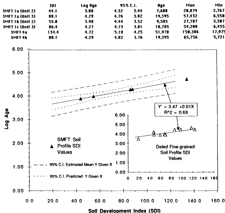
Figure A1. Soil development index (SDI) parameters for soil profiles in Santa Monica fault trenches. Soil profile locations as in Table A1. Regression method is from Rockwell et al. (1990).
