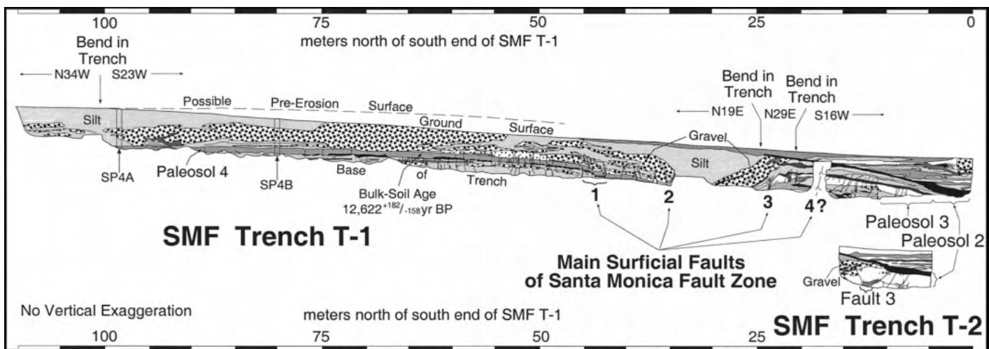
Figure 6. Logs of trenches T-1 and T-2. Note south-dipping sequence onlapped by late Holocene Sepulveda fan strata near south ends of trenches and major disruption of prominent gravel bed by faults 2 and 3. Pre-erosion surface is based on extrapolation of paleosol 4 surface to ground surface southward from 100 m north. No vertical exaggeration.
