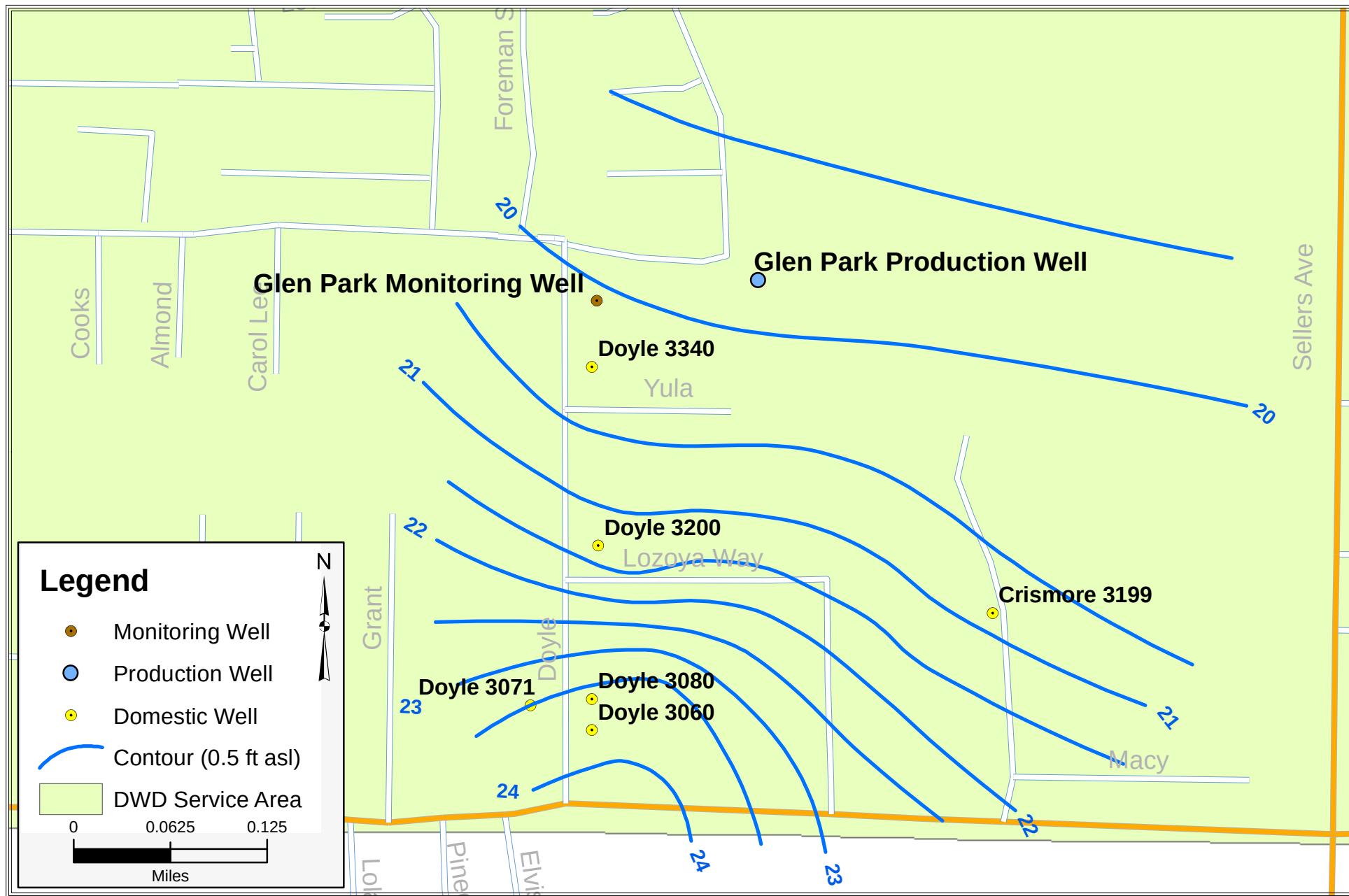
Figure 16B Shallow Groundwater Elevation Contours, Fall 2010 Vicinity of Glen Park Production Well
