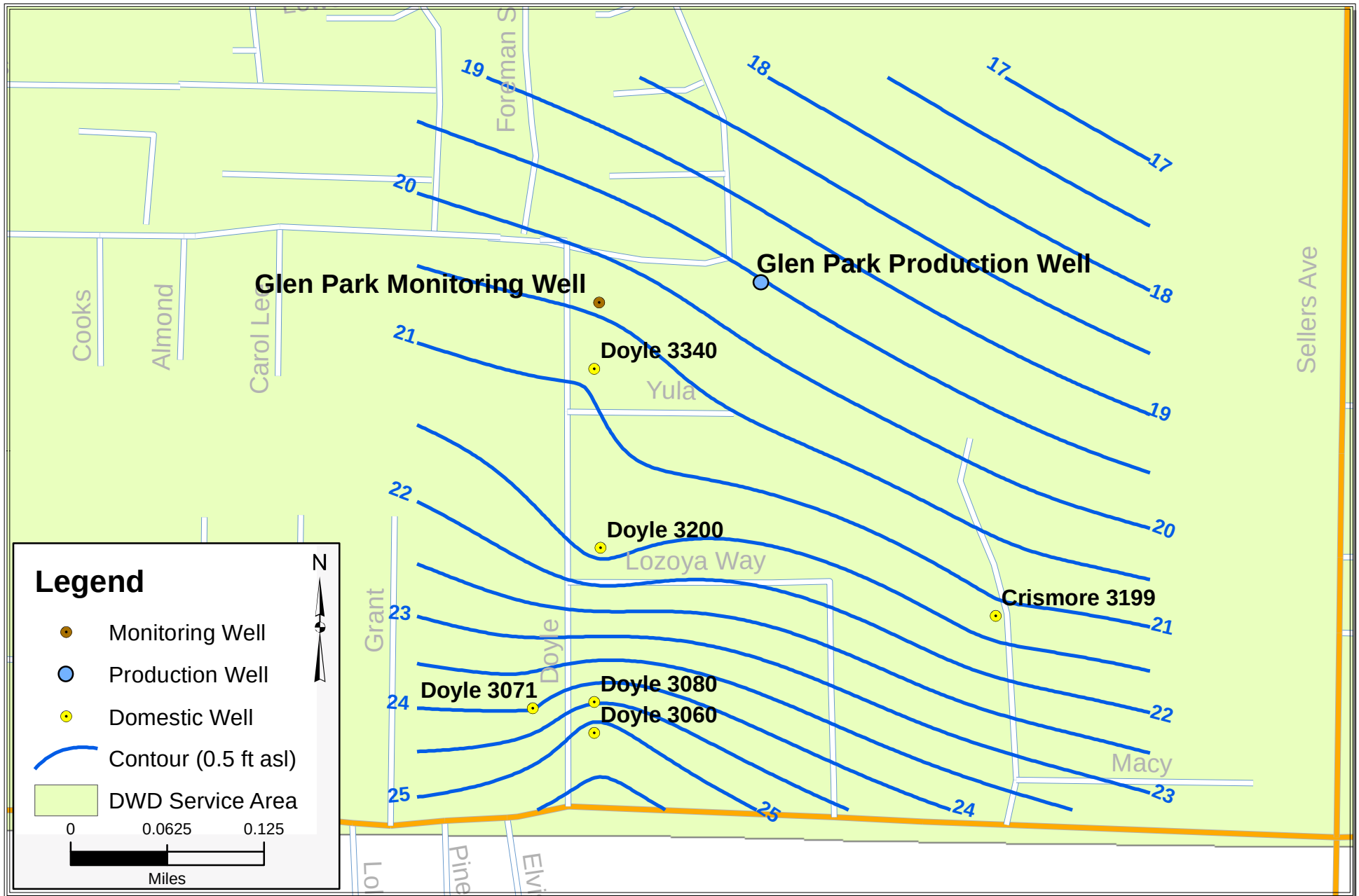
Figure 15A Shallow Groundwater Elevation Contours, Spring 2009 Vicinity of Glen Park Production Well
