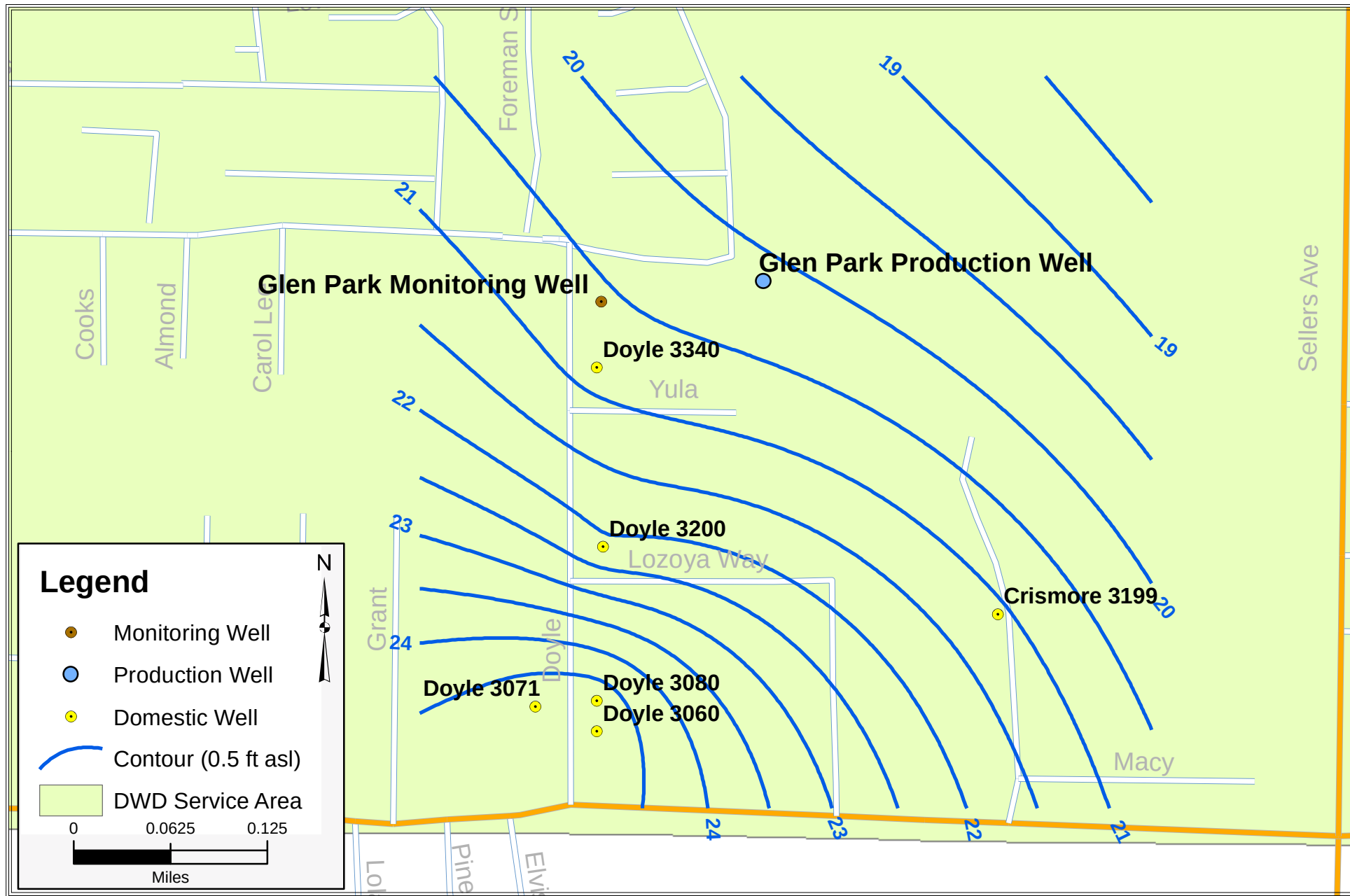
Figure 15B Shallow Groundwater Elevation Contours, Fall 2009 Vicinity of Glen Park Production Well
