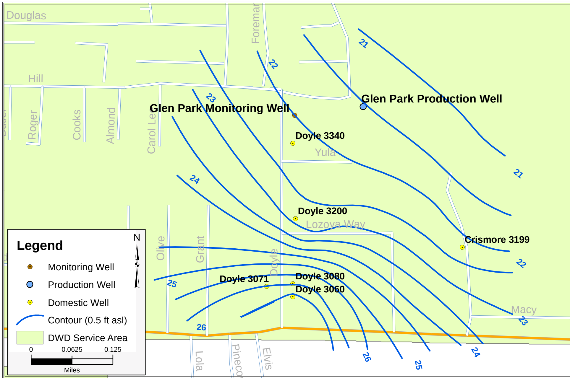
Figure 16A Shallow Groundwater Elevation Contours, Spring 2010 Vicinity of Glen Park Production Well
