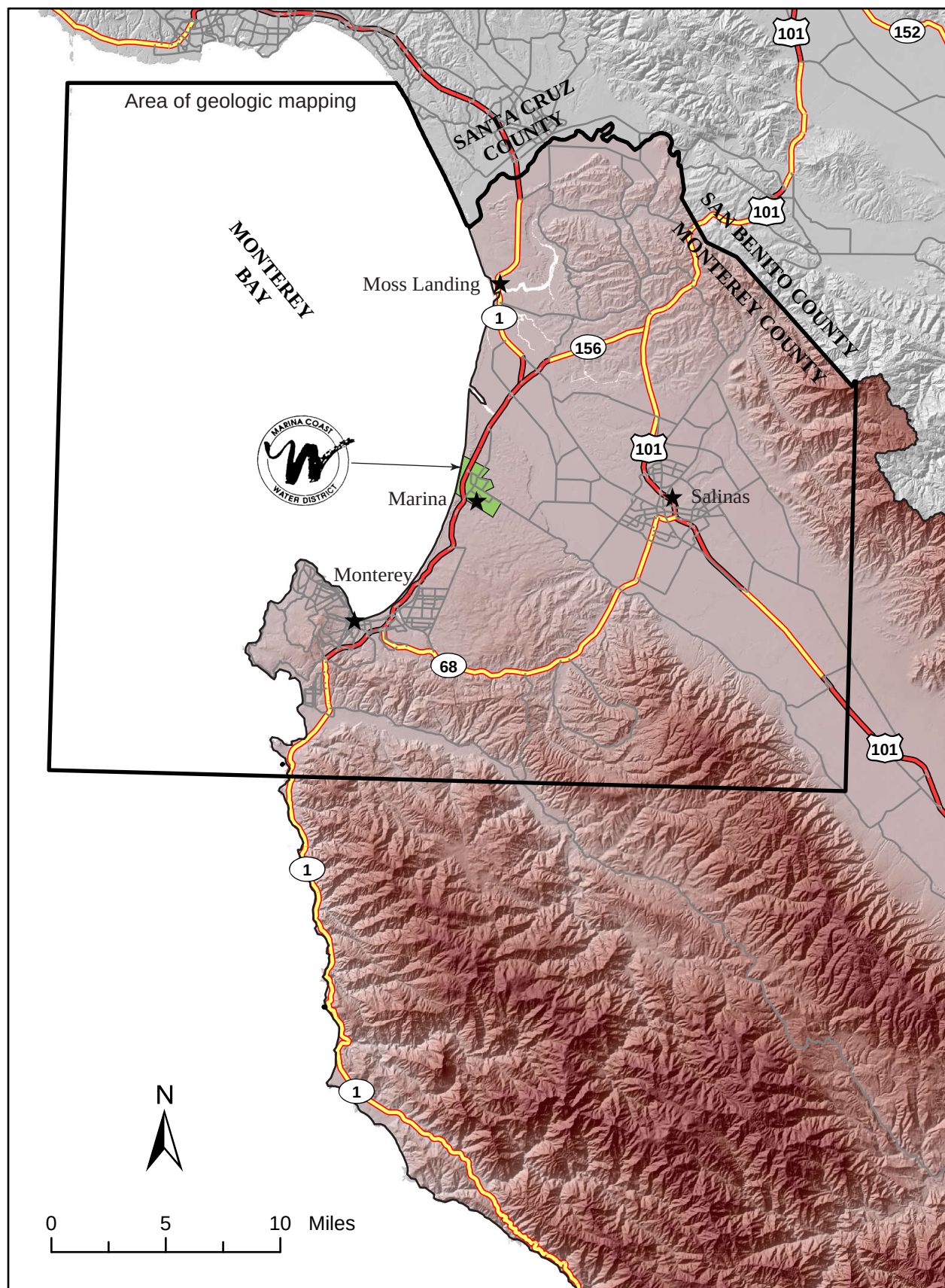
Figure 1. Vicinity map showing Marina Coast Water District and area of geologic mapping
