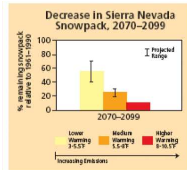
Figure 6-1: Projected Snowpack Changes in the Sierra Nevada
