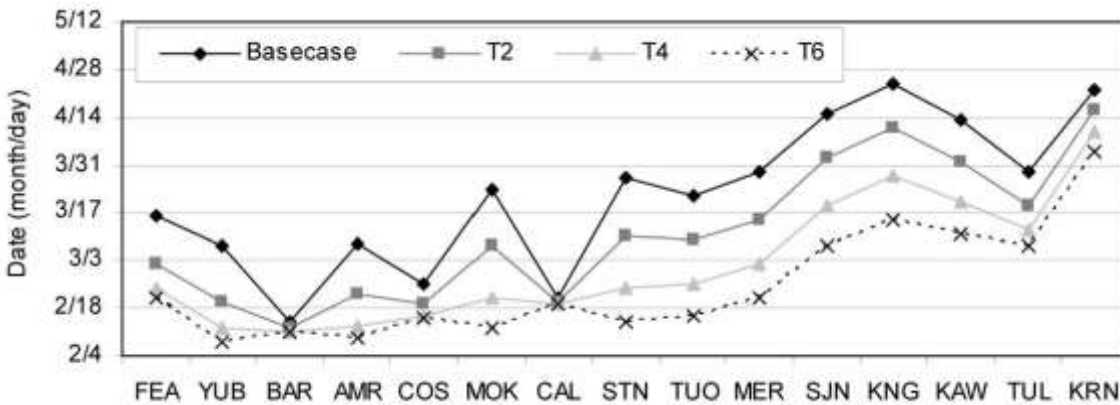
Figure 6-3: Average Annual Centroid Timing by Watershed
