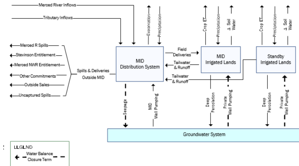
Figure 5.1 Flow Path and Components of Water Balance
