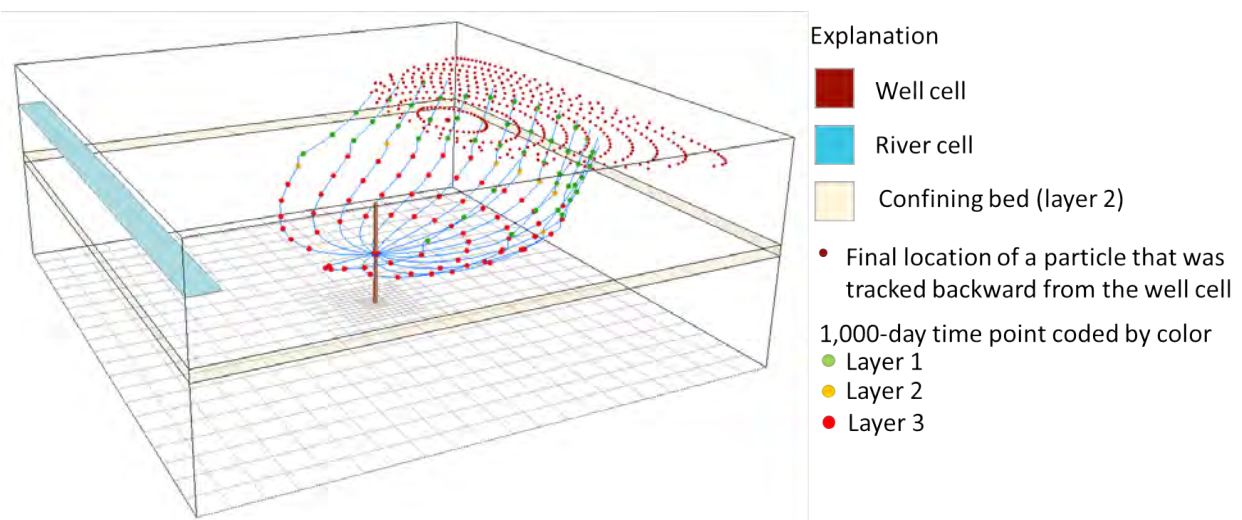
Figure 30. Three-dimensional view of particle-tracking results for MODPATH simulations 2A and 2B.
