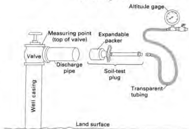
Components used to measure water pressure of flowing wells
