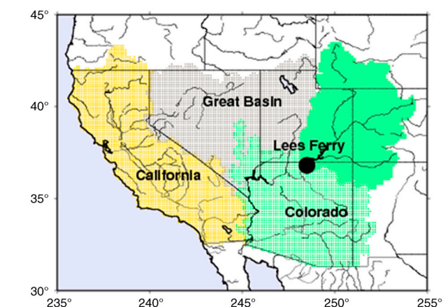
Fig. 1. The study area consists of three regions: California, Great Basin, and Colorado River Basin. Together these are called the “Southwest.”
