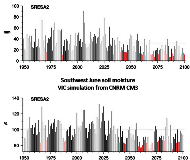
Fig. 4. Southwest region April first snow water equivalent (mm) (Upper) and June soil moisture (% of 1951–1999 average annual values) (Lower) from VIC simulation of the CNRM CM3 GCM for 1950 to 2100. Climate change period (2000–2100) from scenarios SRES A2. Extremely dry years are indicated by red bars that mark years when April 1 SWE or June soil moisture is lower than the 10th percentile of the historical (1951–1999) period (18.0 mm).
