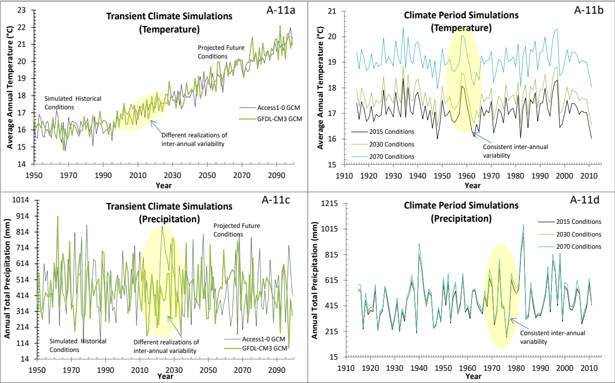
Figure A-11. Transient and Climate Period Simulations of Temperature and Precipitation
