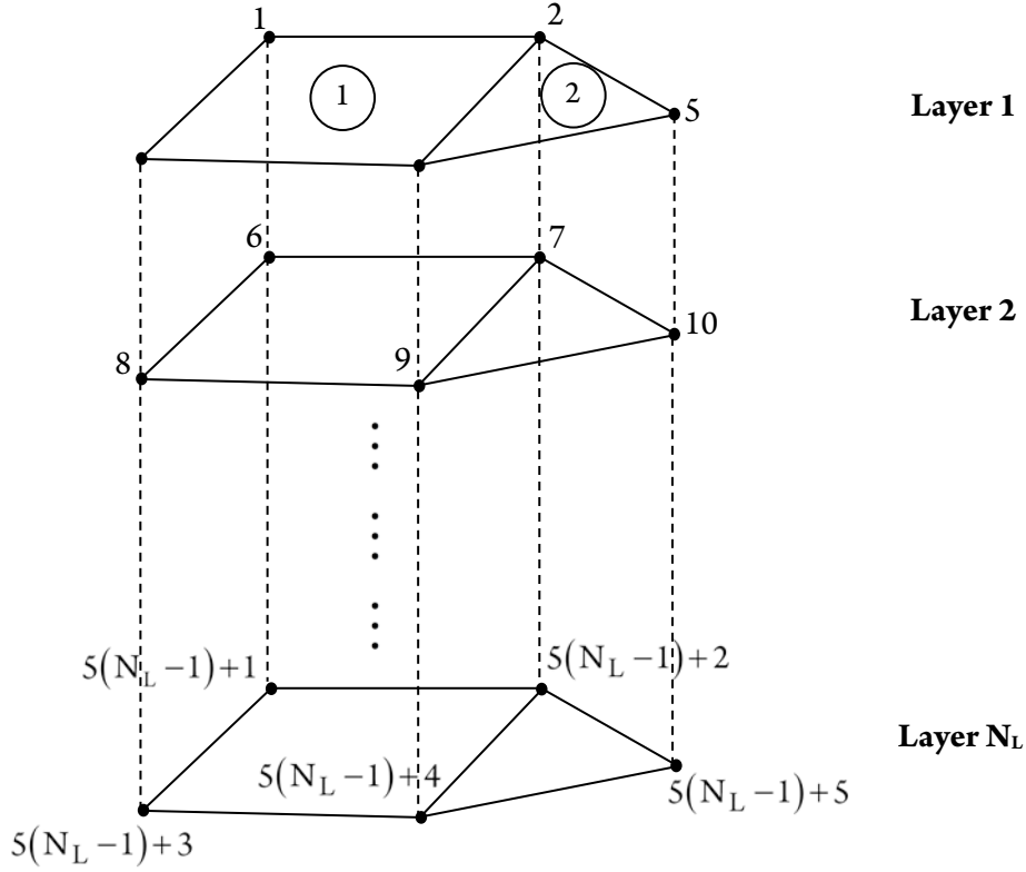
Figure 3.1 Node numbering convention used in IWFM for an aquifer system with N_L layers and N=5 nodes in each layer
