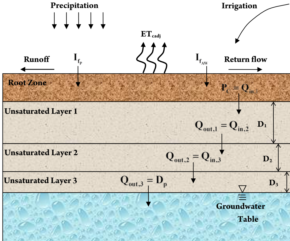
Figure 2.10 Schematic representation of flow through the root zone and the unsaturated zone
