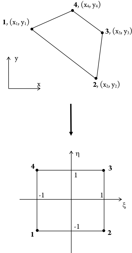
Figure 3.3 Transformation of a quadrilateral element from (x, y) space to (\xi, \eta) space
