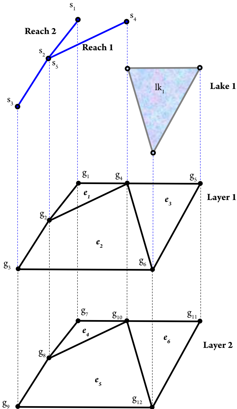
Figure 3.6 Hypothetical model domain
