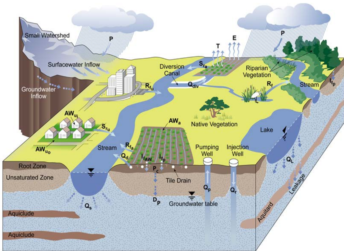
Figure 1.1 Hydrologic processes modeled in IWFM
