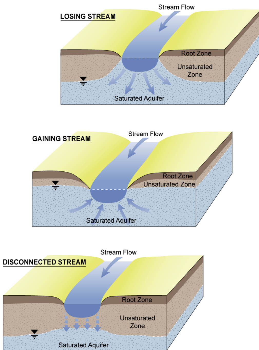
Figure 2.6 Stream-groundwater interaction scenarios
