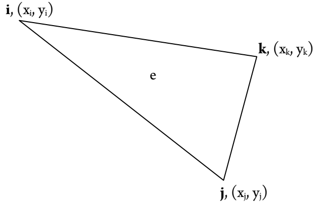
Figure 3.2 A representative triangular element
