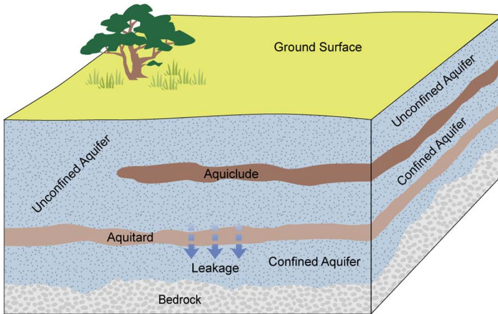
Figure 2.1 Multi-layer aquifer system
