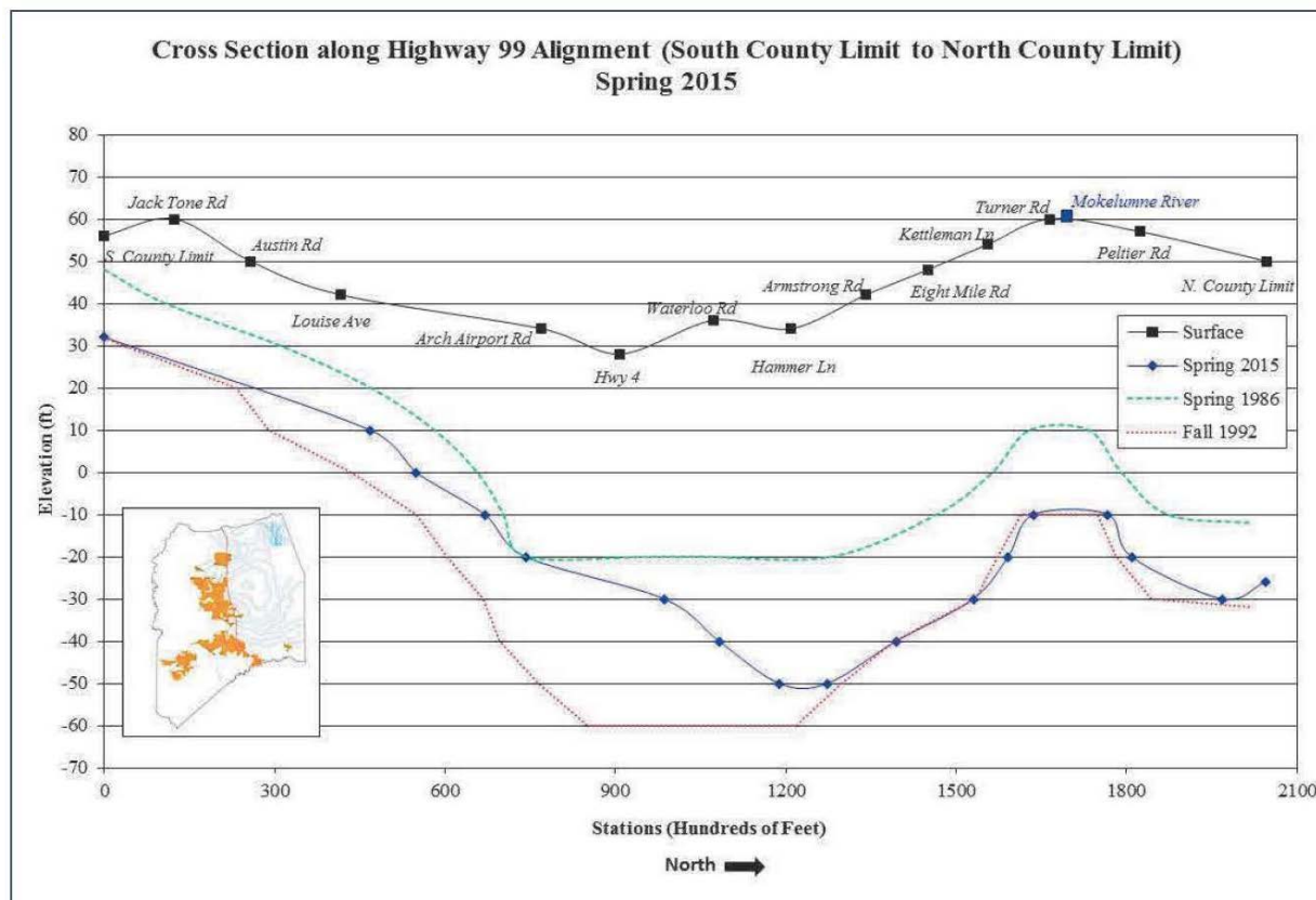
Figure 5-3. Highway 99 Cross Section Groundwater Levels
