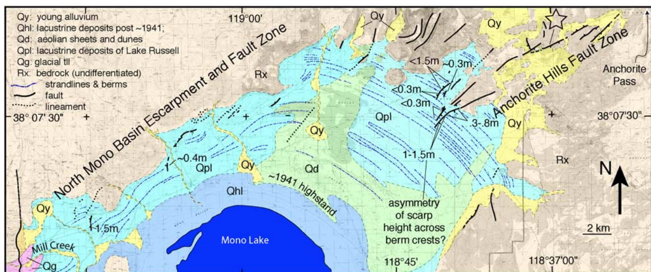
Figure 6. Map showing Anchorite Hills fault zone and scarps along the North Mono Basin escarpment. Scarp heights are annotated. Location of Gilbert et al. 's [1968] ~300 m left-lateral offset of 2.5 Ma bedrock is marked by star.
