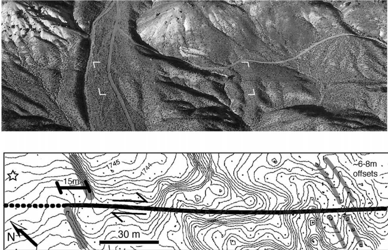
Figure 20. Photo and 0.5 m contour interval map of (shaded) right-lateral offsets of channels, channel margins, and ridgelines along the northern section of the Benton Springs fault. Extent of contour map is shown by white brackets in photo. Coordinates (UTM NAD27 CONUS) of point marked by star are E396102 N4274096. Figure location is also shown in Figure 19.
