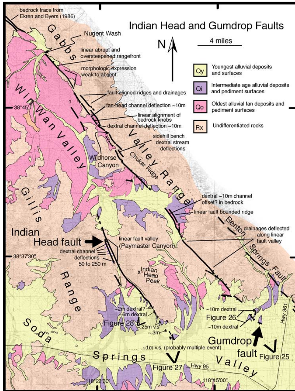
Figure 24. Traces of Indian Head and Gumdrops faults. Features indicative of lateral offset and ongoing fault activity are annotated. Perspectives of photo in Figures 25, 27, and 28 are shown by open ended V shapes. Units Qy, Qi, and Qo are Quaternary surfaces of relatively increasing age. Unit Rx is undifferentiated bedrock. See text for further discussion. See Figure 19 for detail of Benton Springs Fault.
