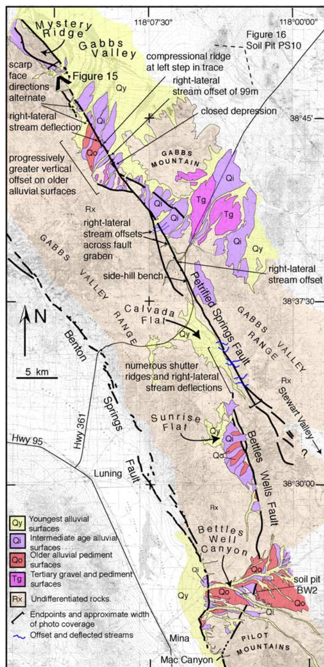
Figure 14. Petrified Springs fault trace. The fault trace (bold lines) is annotated to mark features indicative of lateral offset and ongoing fault activity. Location of map in Figure 16 and soil pit PS10 are also labeled. Perspective of photo in Figure 15 is shown by bold open ended V shape. Units Qy, Qi, and Qo are Quaternary surfaces of relatively increasing age. Units Tg and Rx encompass Tertiary gravels and undifferentiated bedrock, respectively. See text for further discussion. Details of Benton Springs fault are shown in Figure 19.
