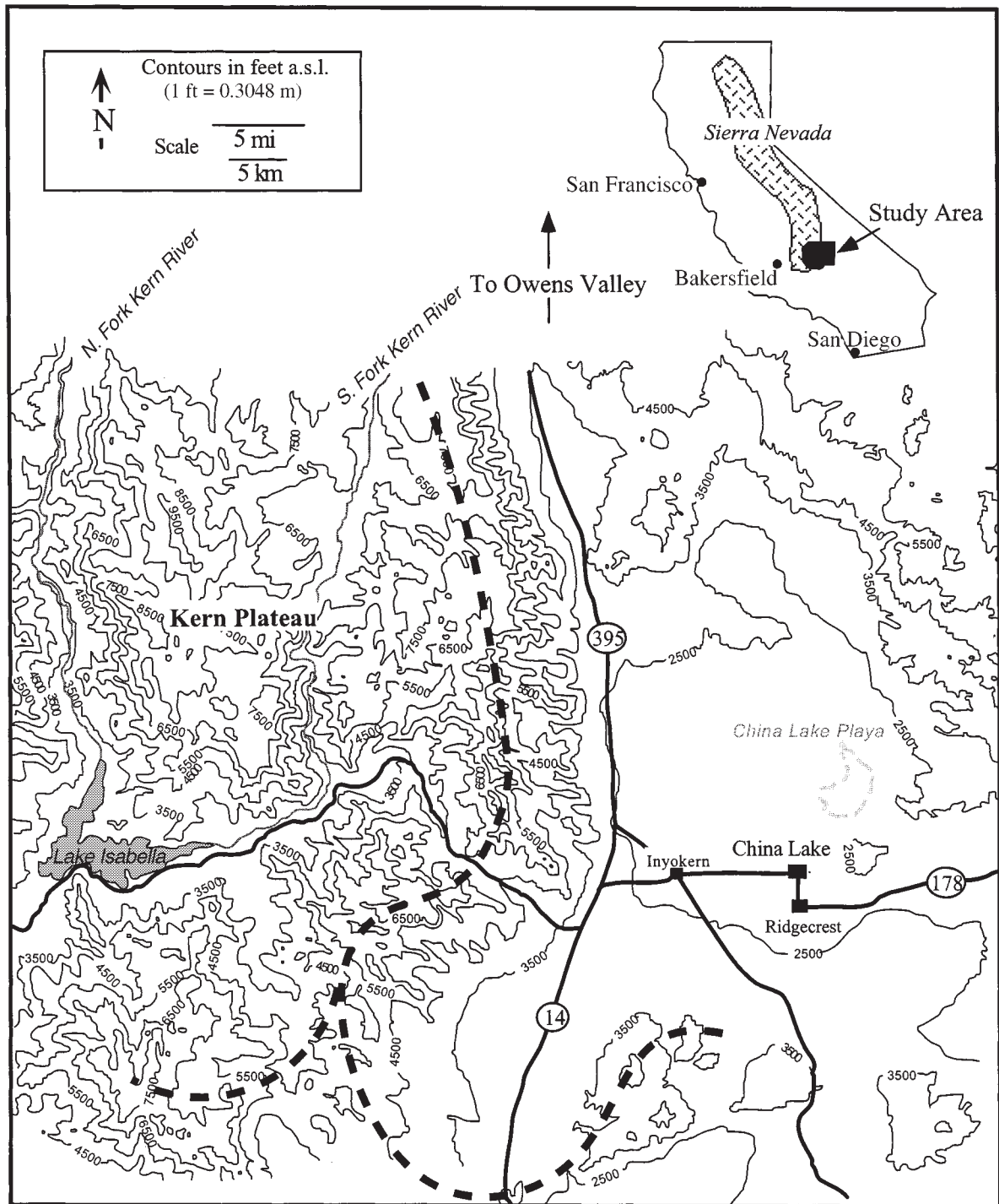
Figure 1. Topographic map of the Indian Wells Valley and Kern Plateau area encompassing lat 35°20'N to 36°10'N and long 117°20'W to 118°45'W. Note location of Lake Isabella in the west and the outline of the topographic drainage (heavy dashed line) for orientation. Modified from U.S. Geological Survey (1981).
