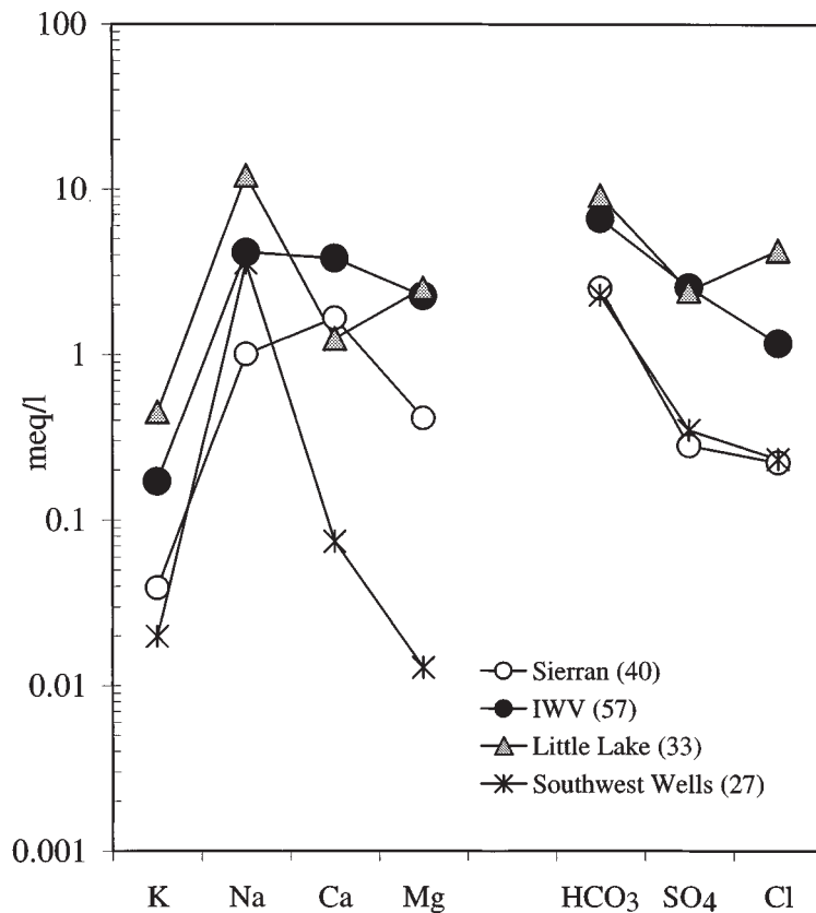
Figure 7. Schoeller diagram of the four hydrochemical facies (Sierran, Indian Wells Valley, Little Lake, and Southwest Wells) found in the study area. Mean values are plotted, other statistical data for each facies are listed in Table 2.
