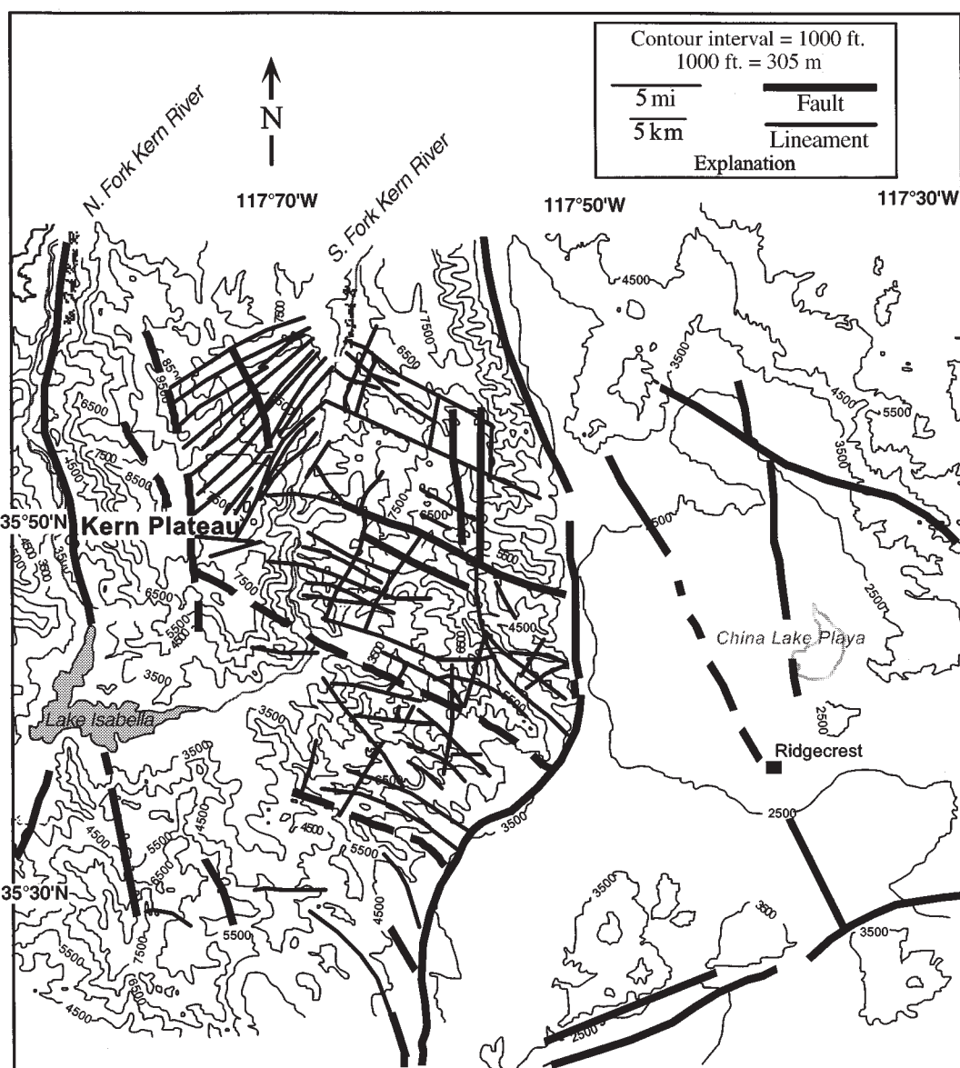
Figure 12. Map view of selected faults and lineaments in the study area. Modified from Ostidick (1997) and Figure 1 (this study).
