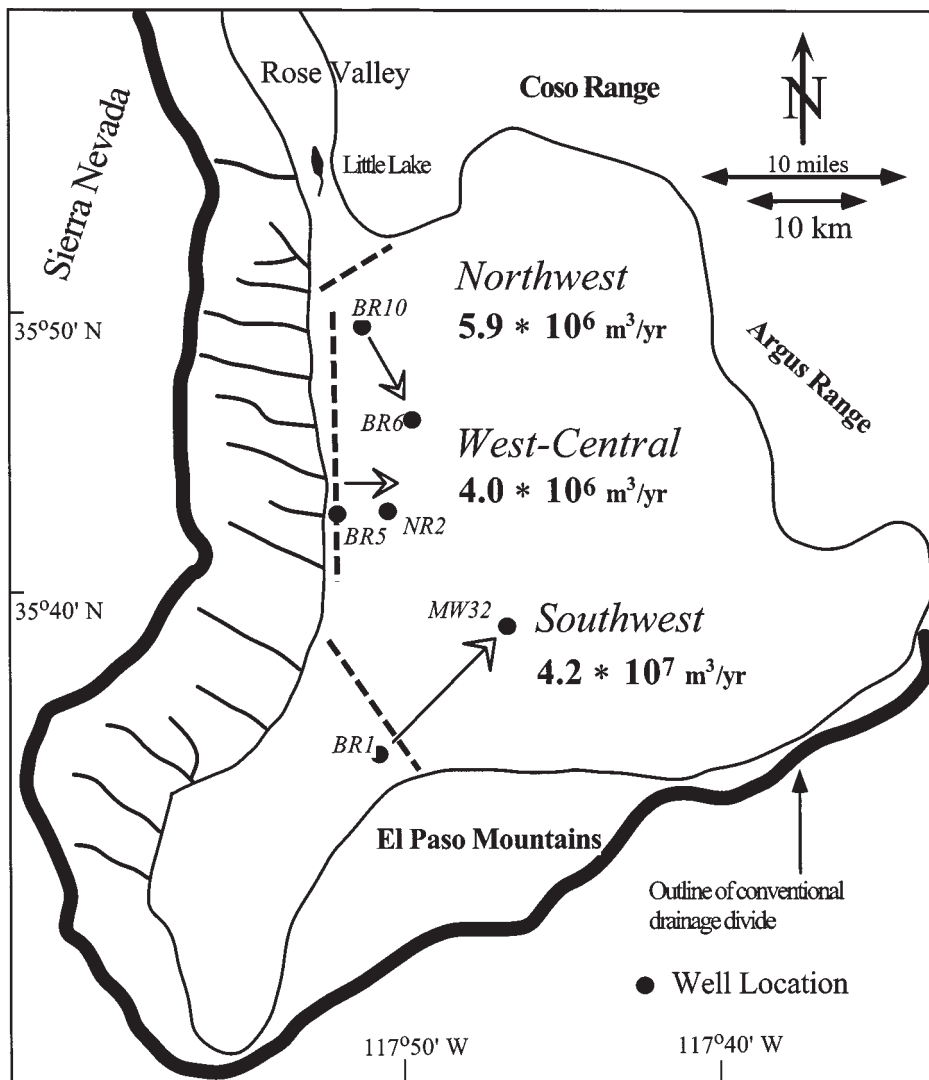
Figure 5. Results of the aquifer flux calculations using Darcy's Law. Data used in the calculations are listed in Table 1. The locations of the wells used to estimate the potentiometric gradient are shown with arrows to indicate the direction of flow. The heavy dashed lines indicate the cross-sectional area used to calculate the flux.
