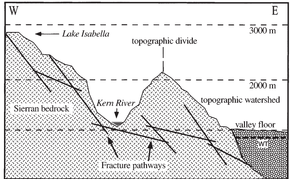
Figure 13. Conceptual model of fracture flow from the Kern Plateau into the Indian Wells Valley (not to scale). Flow crosses the local phreatic divide (Kern River) to discharge into the alluvial aquifer. WT—water table.
