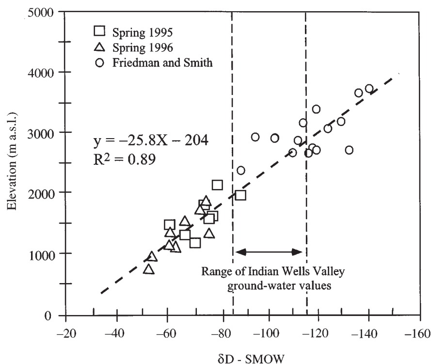
Figure 10. Plot of hydrogen isotope ratios ( \delta D ) (SMOW, standard mean ocean water) versus elevation for the study area. Dashed line shows the linear regression for the data (equation shown). The data are from the rain gauge samples and published values (Friedman and Smith, 1972).
