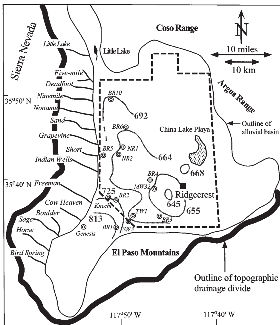
Figure 2. Schematic map view of Indian Wells Valley shows the locations of the canyons and wells (italics). Multipiezometer wells have the BR or NR prefix. The heavy dashed line shows the area included in prior models (Bloyd and Robson, 1971; Berenbrock and Martin, 1991). The potentiometric contours (in meters above sea level) are the heavy gray lines taken from 1991 head measurements (Kern County Water Agency, 1992). Note the irregular contour interval.
