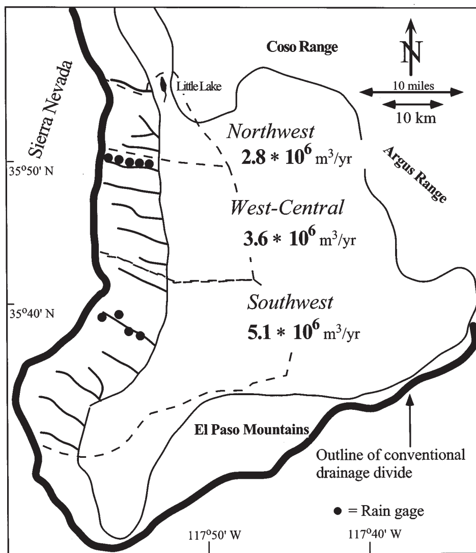
Figure 4. Results of recharge calculated by the precipitation-based method. The three sections of the study area and locations of the rain gages are also shown. The value for the northwest section includes the contribution from the Little Lake stream outflow ( 1.6 \times 10^6 \text{ m}^3/\text{yr} ).
