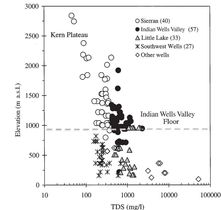
Figure 9. Plot of elevation (meters above sea level, m a.s.l.) versus total dissolved solids (TDS) for the hydrochemical facies and the deep wells (other wells) influenced by geothermal brine.
