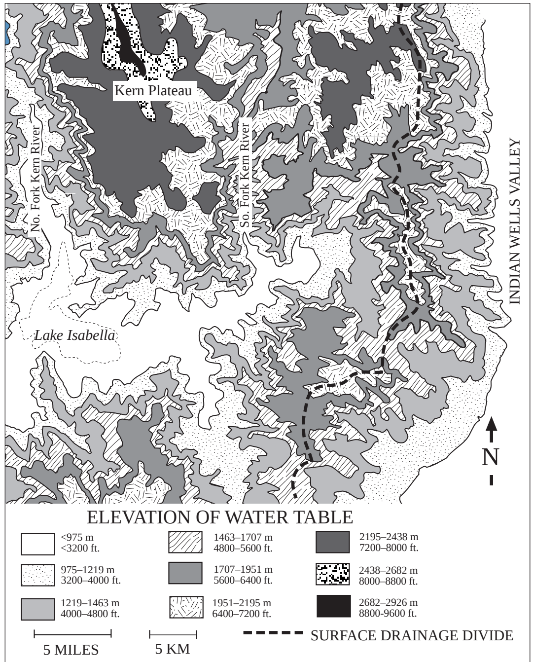
Figure 11. Map of potentiometric surface contours in the eastern Sierra and Kern Plateau areas. Map is modified from Howard et al. (1997a).
