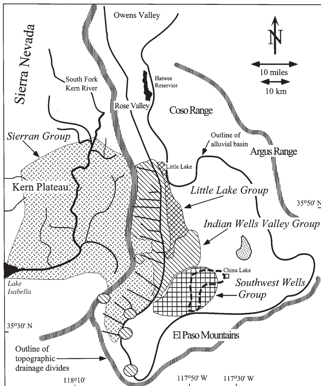
Figure 8. Map view of the hydrochemical facies ( italics ) in the study area. The heavy dashed line shows the location of wells where the tritium data show that a significant fraction of the ground water is post-1952 in age.
