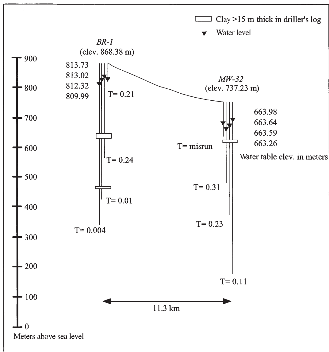
Figure 6. Schematic cross section of the multipiezometer wells and slug test hydraulic transmissivity values for the southwest section wells BR1 and MW32 used for the flux calculations.
