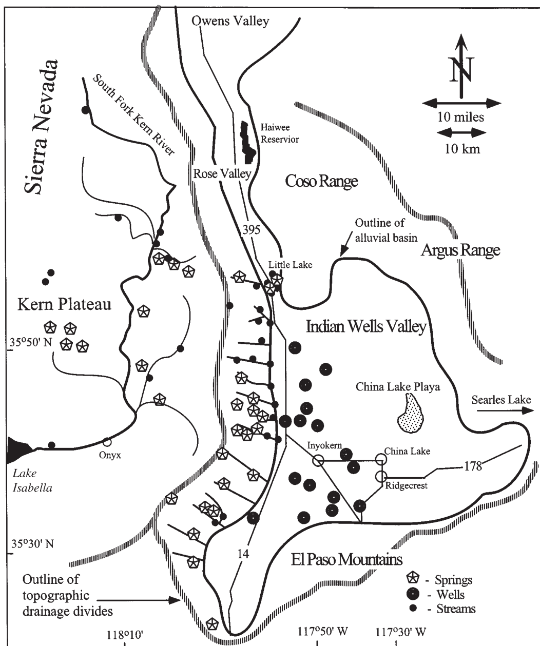
Figure 3. Schematic map view of study area showing the location of wells, springs, and streams sampled in this study. Chemical and isotopic data for the samples are in the Data Repository (see text footnote 1).
