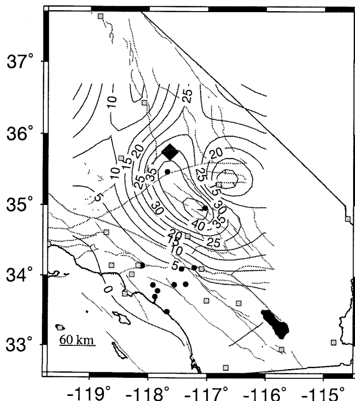
▲ Figure 4 (A) Vertical and (B) horizontal peak accelerations in \text{cm/sec}^2 from the M 5.8 earthquake (epicenter indicated by solid diamond). The ground motions are affected by distance from the epicenter and local site effects. The open squares are TERRAScope stations while the filled circles are analog SCSN stations and digital AMOES/CalREN stations with strong motion sensors.
