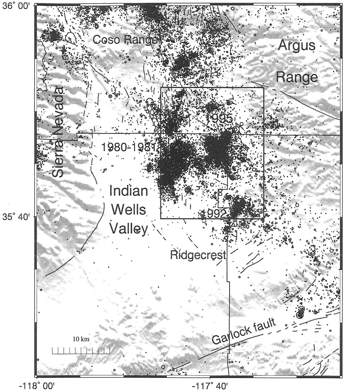
▲ Figure 1 Overview of seismicity in Indian Wells Valley recorded by the Southern California Seismic Network from 1980 to 1995. Symbol size is scaled with magnitude. The swarms of 1980–1981, 1992, and the 1995 sequence are labeled with the year. The box indicates the location of Figures 2 and 3. The straight lines are the county boundaries.
