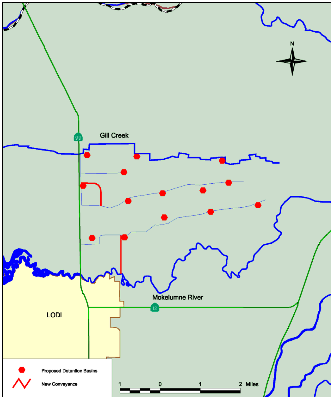
Figure 8-17 Gill Creek and Woodbridge Road Flood Control Improvements
