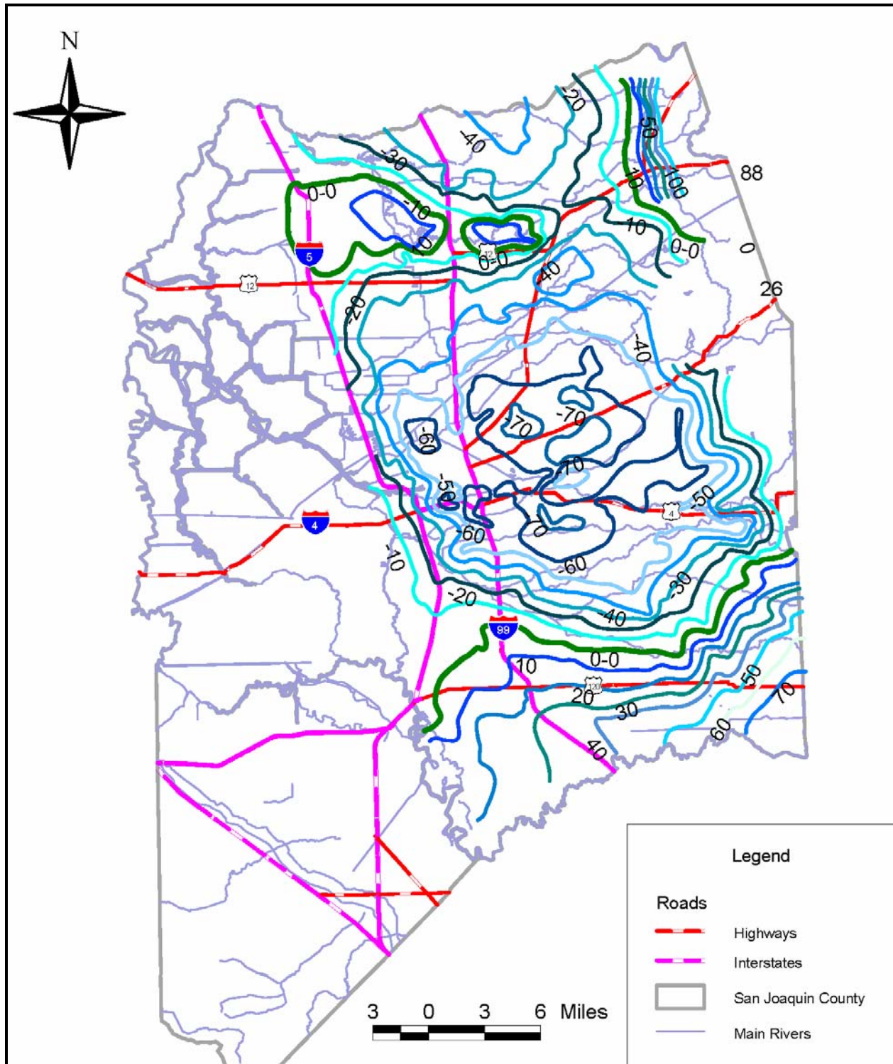
Figure 2-4 Fall 1993 Groundwater Contours
