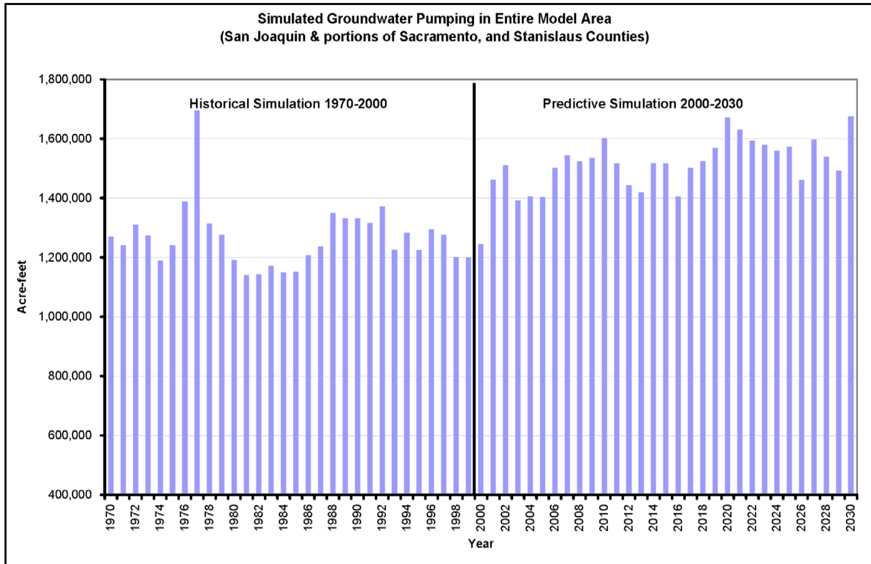
Figure 2-23 Simulated Groundwater Pumping
