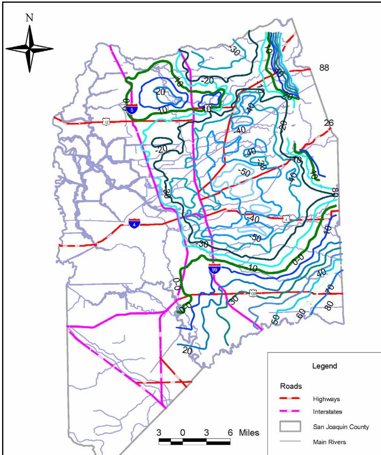
Figure 2-6 Fall 1998 Groundwater Contours
