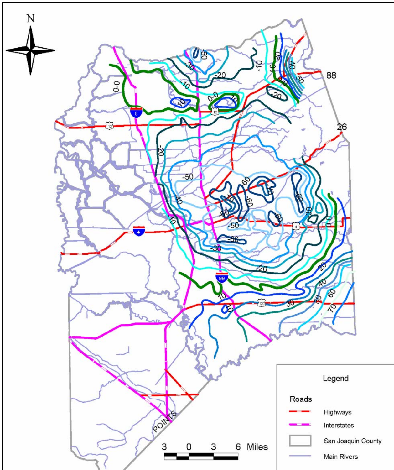
Figure 2-3 Spring 1993 Groundwater Contours
