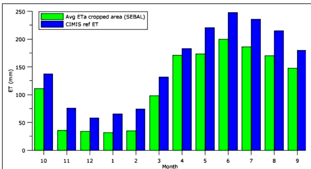
Figure 4. Average ET_a for Cropped Area in IID Compared with Average ET_0 .
