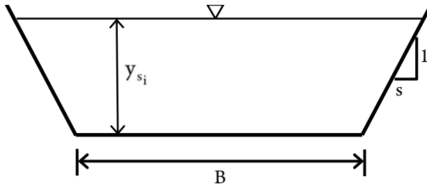
Figure 2.8 A trapezoidal channel cross-section and relevant parameters
