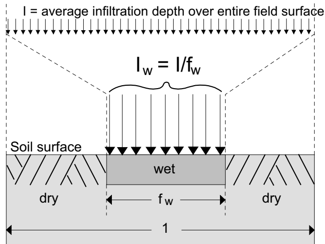
FIGURE 31 Partial wetting by irrigation
