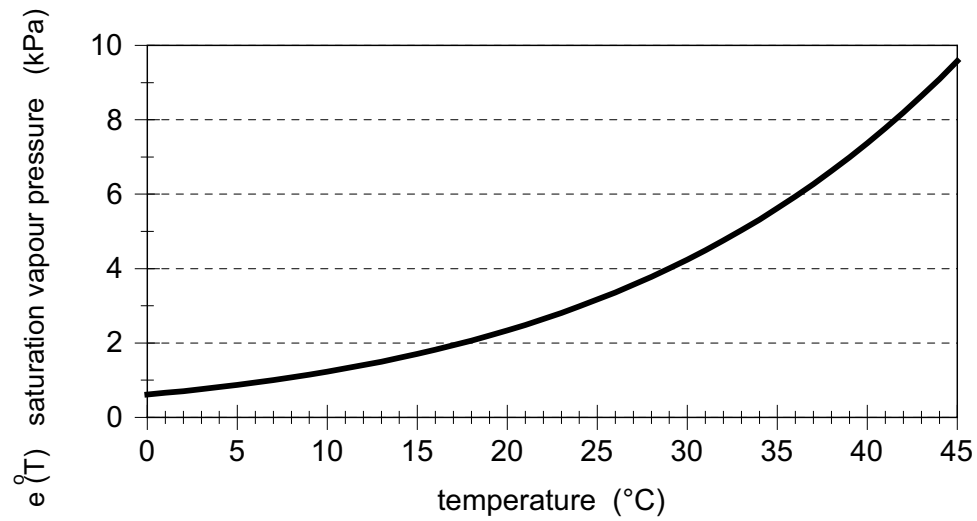
FIGURE 11 Saturation vapour pressure shown as a function of temperature: e^s(T) curve
