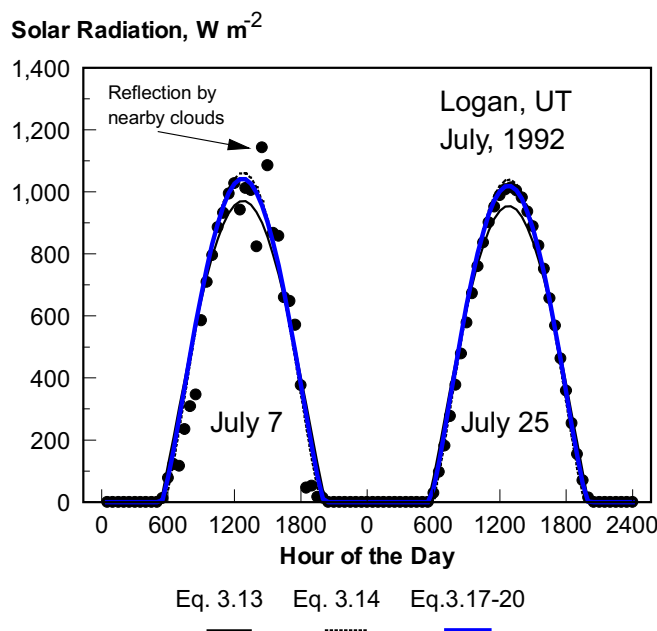
FIGURE 5.2 30-minute average R_s and estimated R_{so} envelopes at Logan, UT during July 7 and July 25, 1992
