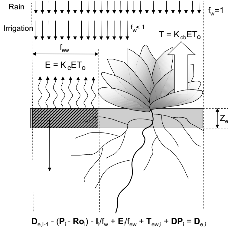
FIGURE 40 Water balance of the topsoil layer
