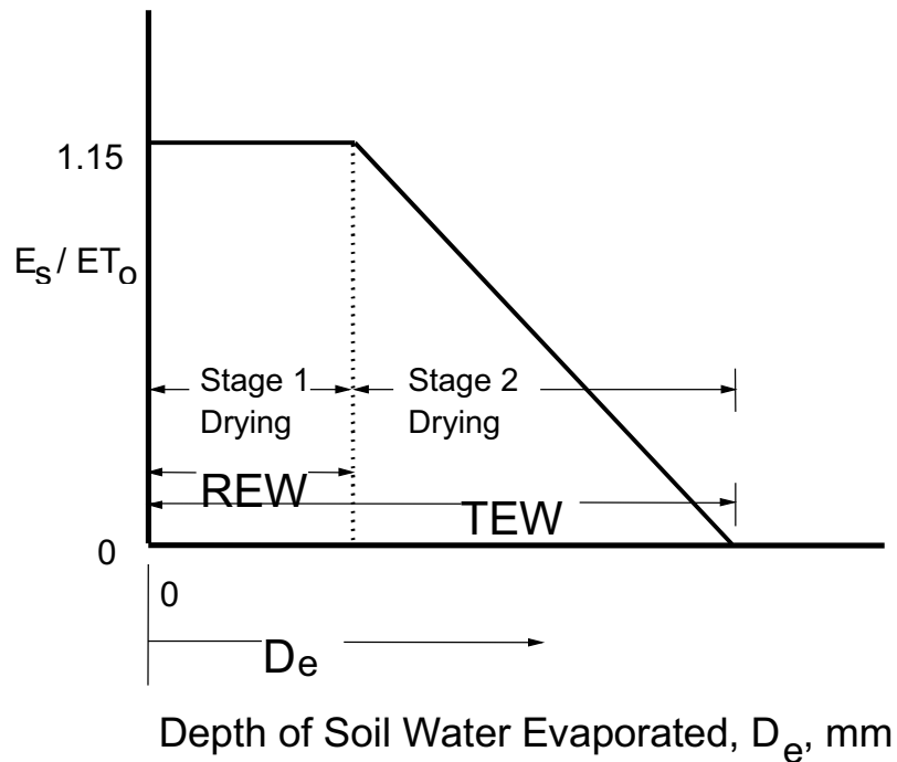
FIGURE 7.1 Two stage model for soil evaporation during the initial period
