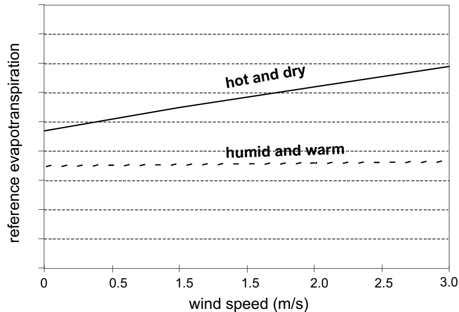
FIGURE 10 Illustration of the effect of wind speed on evapotranspiration in hot-dry and humid-warm weather conditions
