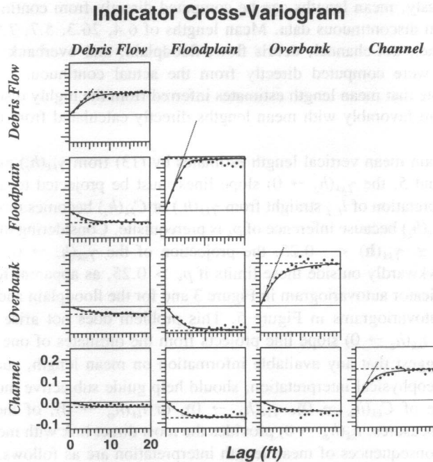
Figure 5. Corresponding to all four lithofacies shown in Figure 1: vertical indicator cross-variogram measurements (circles), sills (dashed lines), and estimated slope lines (dotted lines); autovariogram models (solid curves, on diagonal) fitted by sum of spherical and exponential models and, corresponding to (16), random cross-variogram models (solid curves, on off-diagonal).
