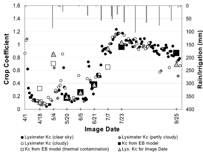
Fig. 4. Comparison of ET_r ( K_c ) by METRIC (EB model) and by lysimeter for sugar beets near Kimberly, Id. during 1989 (unpublished lysimeter data from Wright 2000, USDA-ARS, Kimberly, Id.) (adapted from Tasumi et al. 2005a)
