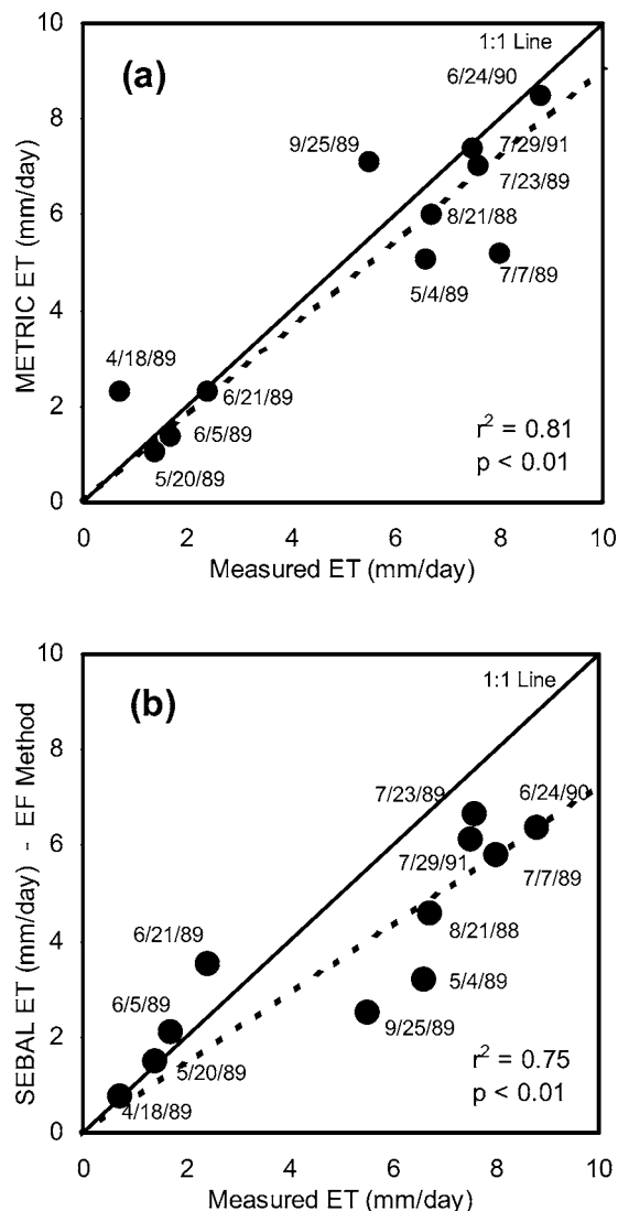
Fig. 3. Comparison of daily ET from METRIC using ET r F (a); from SEBAL (version 2000) using EF (b) on satellite image dates for sugar beets (1989), potatoes (1988), peas (1990), and alfalfa (1991) compared against lysimeter measurements at Kimberly, Id. (measurement data from Dr. J. L. Wright, USDA-ARS) (graphed data from Trezza 2002)
