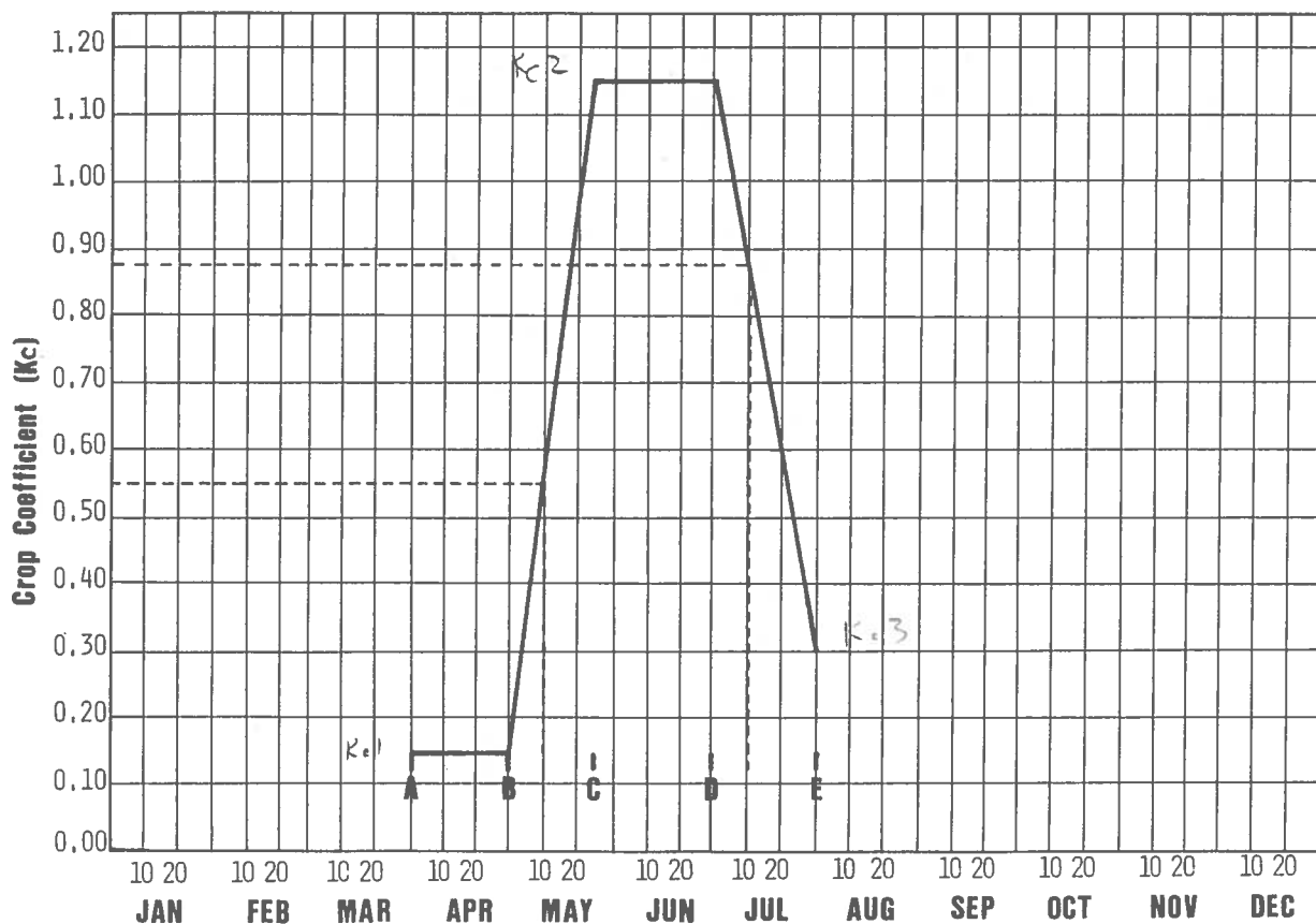
Fig. 2. Crop coefficient ( Kc ) curve for beans grown in the San Joaquin Valley with planting on April 1, 10 percent ground shading on April 30, 75 percent ground shading on May 25, and maturity on July 31.
