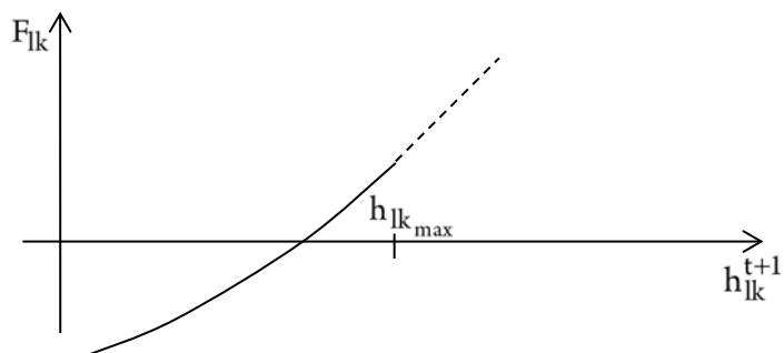
Figure 3.5 Plots of possible lake storage functions and the modified function when lake elevation exceeds the maximum elevation
