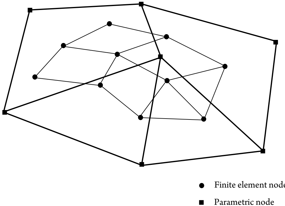
Figure 3.7 An example of parametric and finite element mesh systems
