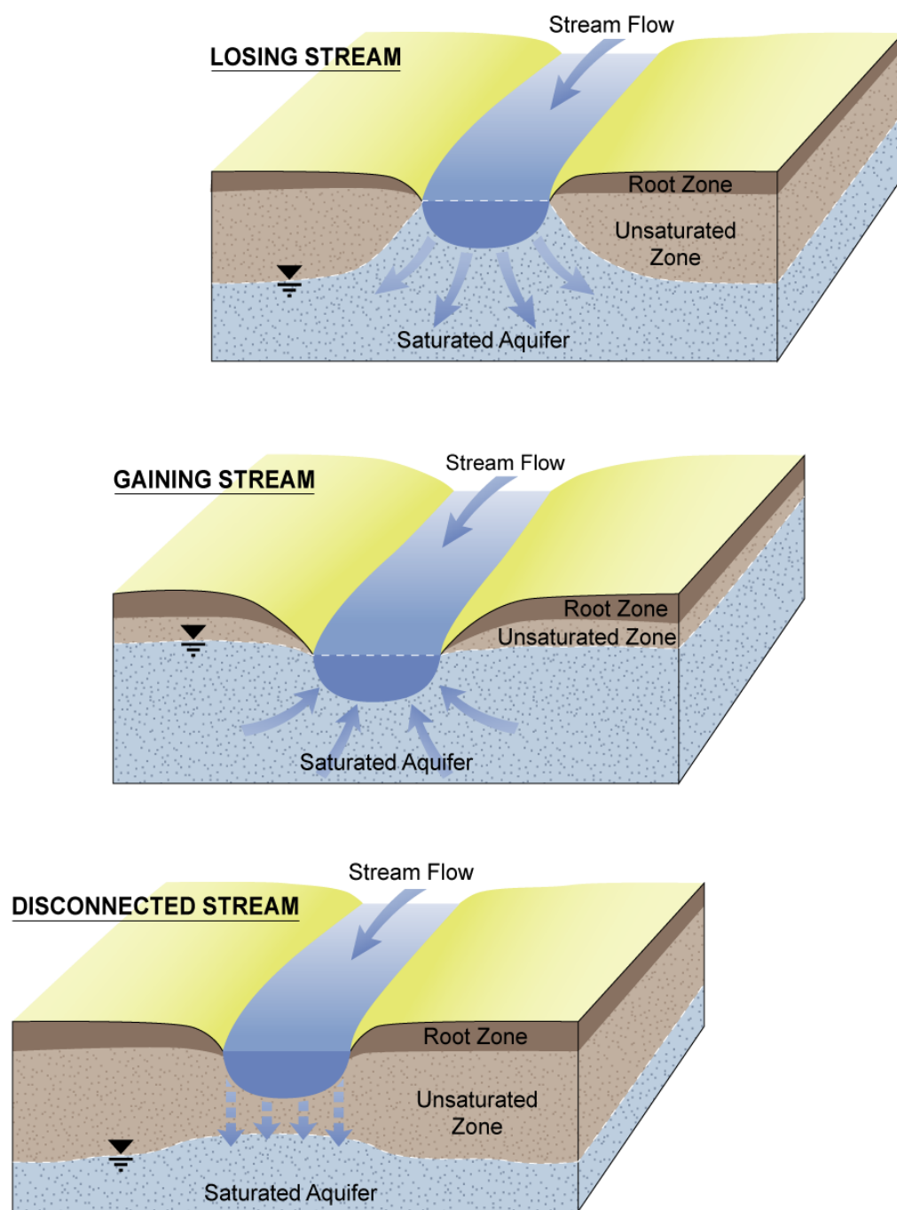
Figure 2.6 Stream-groundwater interaction scenarios
