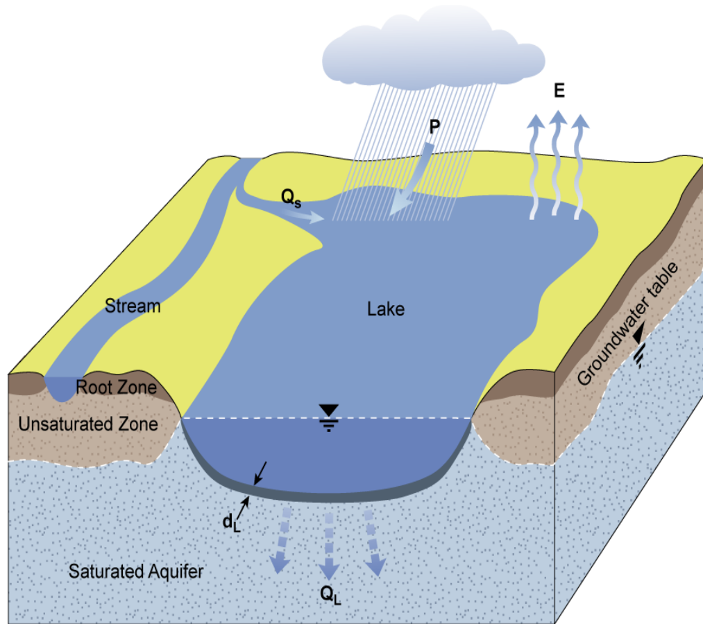
Figure 2.9 Hydrological components that affect lake storage
