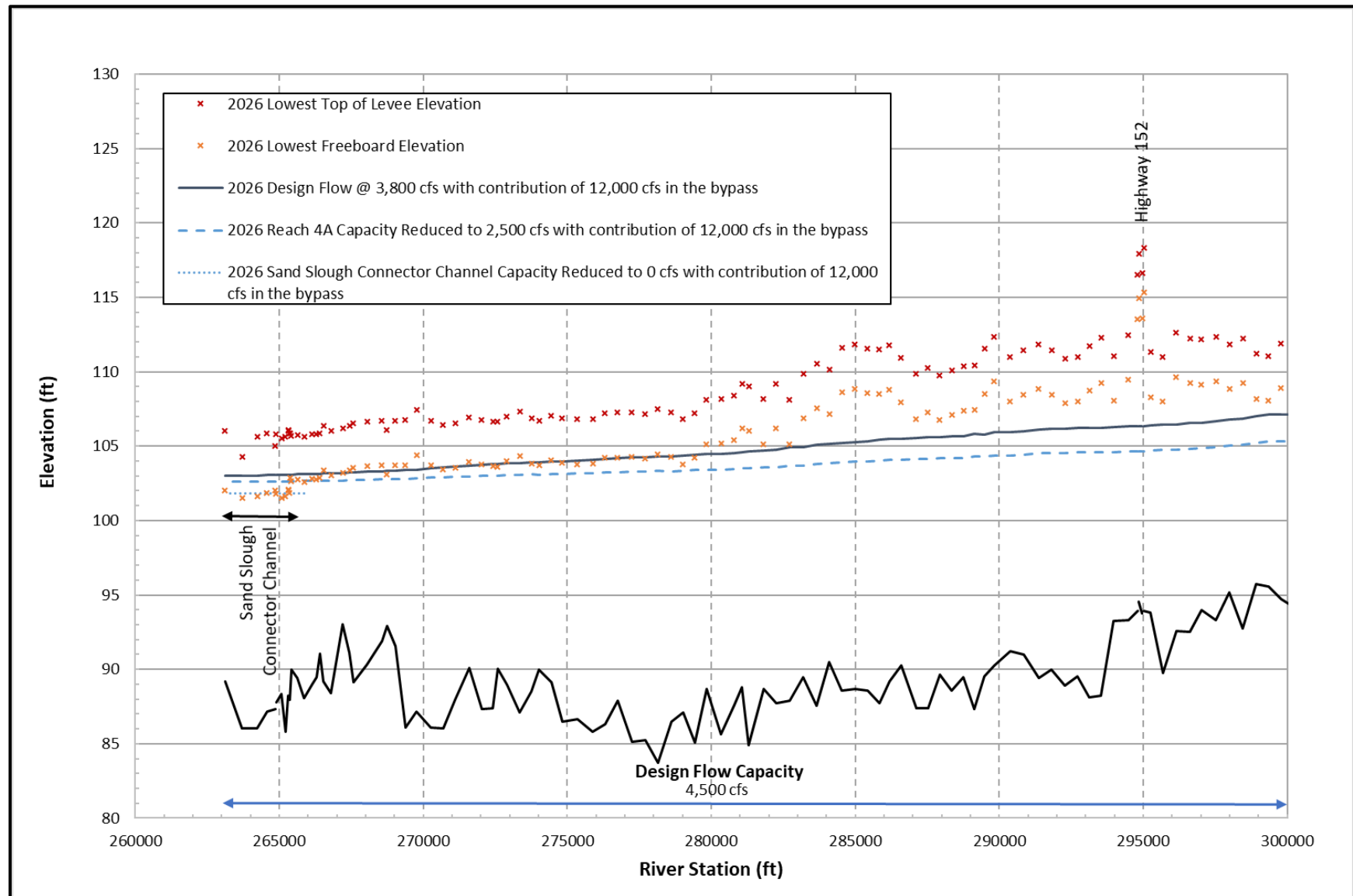
Figure 21 Water Surface Profile for 2026 Backwater Condition for Reach 4A from Highway 152 to Sand Slough
