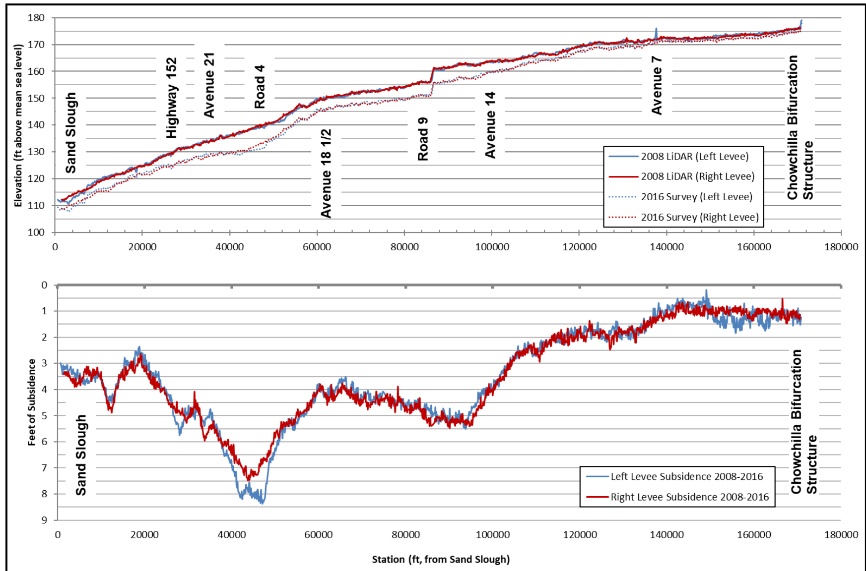
Figure 3 Ground Subsidence along the Chowchilla and Eastside Bypasses from the Chowchilla Bifurcation Structure to Sand Slough (2008–2016)
