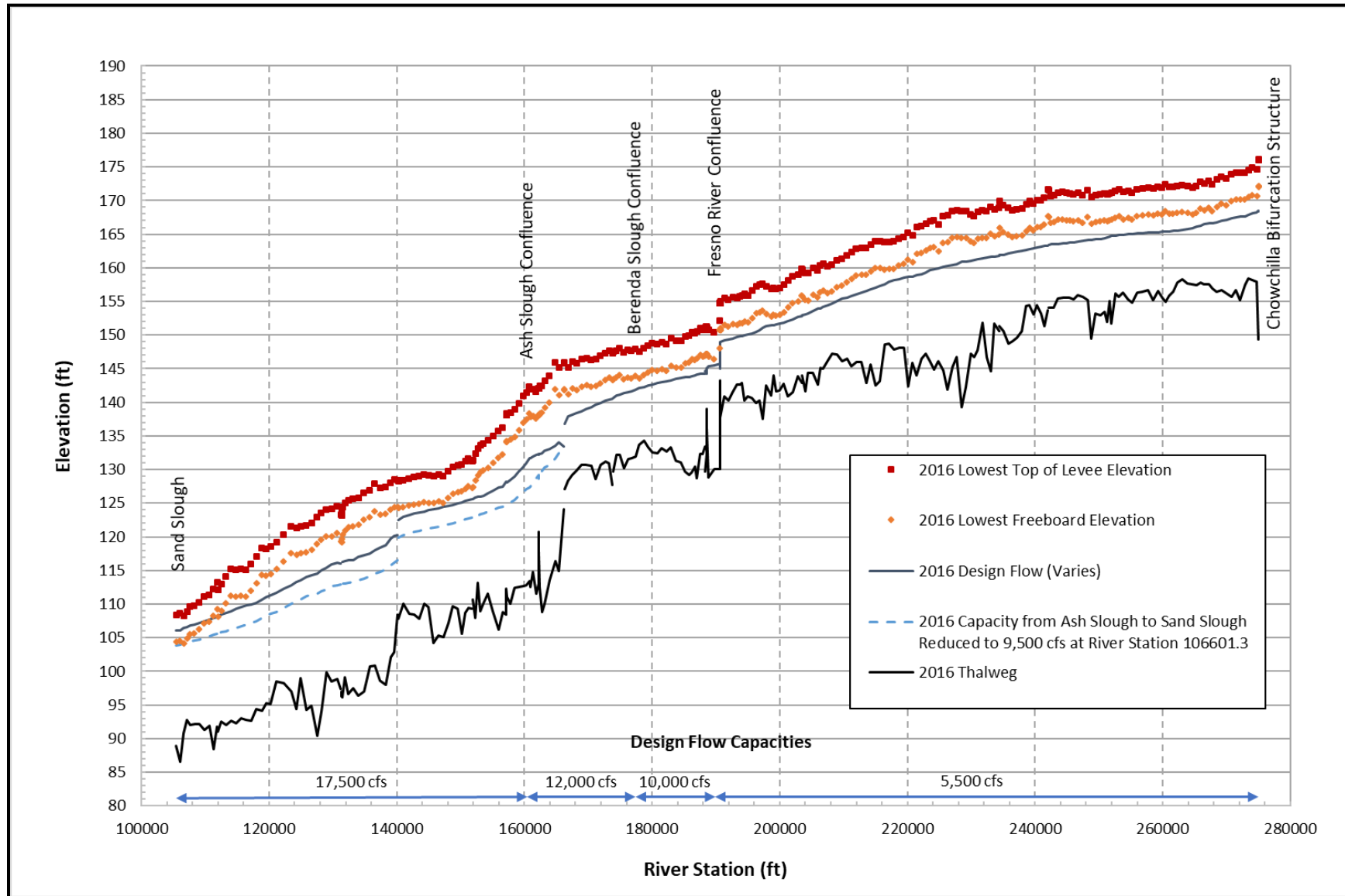
Figure 12 Water Surface Profile for 2016 Run-of-the-River Condition for the Chowchilla and Eastside Bypasses from the Chowchilla Bifurcation Structure to Sand Slough
