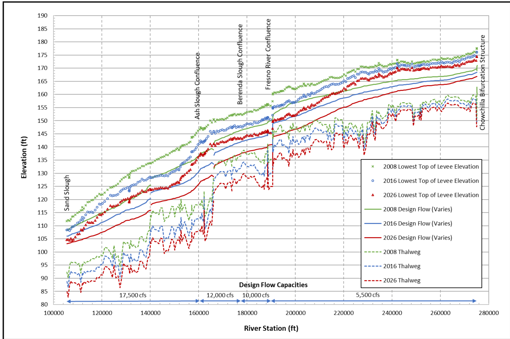
Figure 6 Design Flow Profile under 2008, 2016, and 2026 Run-of-the-River Conditions in the Chowchilla and Eastside Bypasses from the Chowchilla Bifurcation Structure to Sand Slough
