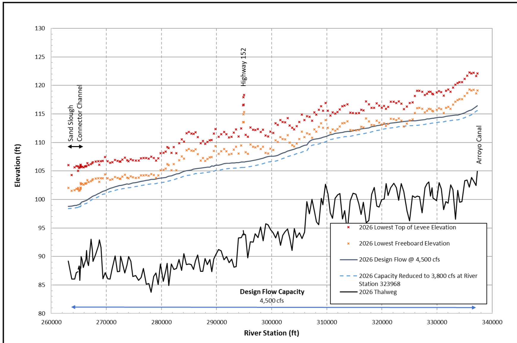
Figure 20 Water Surface Profile for 2026 Run-of-the-River Condition for Reach 4A from Arroyo Canal to Sand Slough
