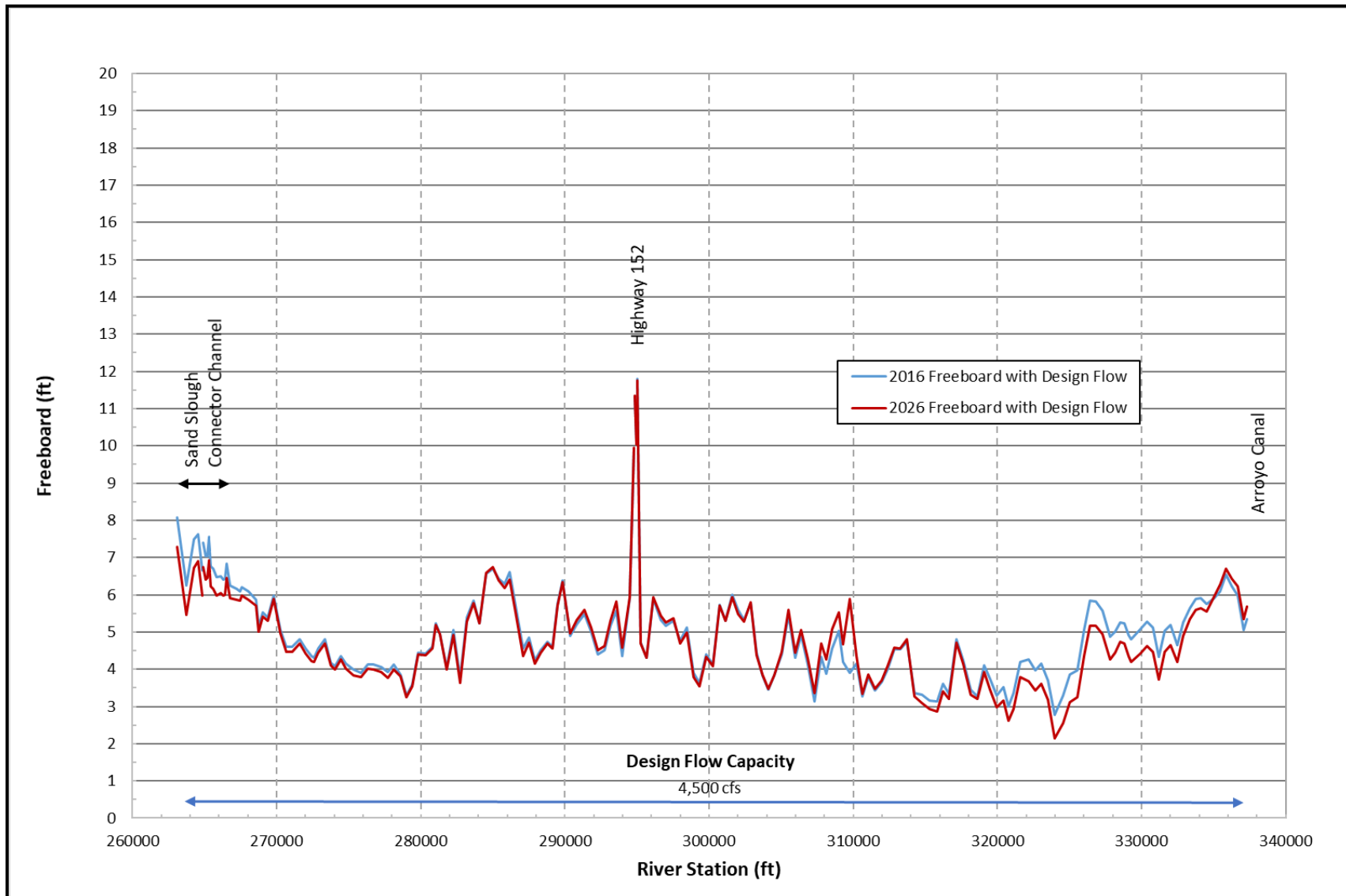
Figure 11 Freeboard Conditions for 2016 and 2026 Run-of-the-River Conditions for Reach 4A of the San Joaquin River based on Design Flow Capacities
