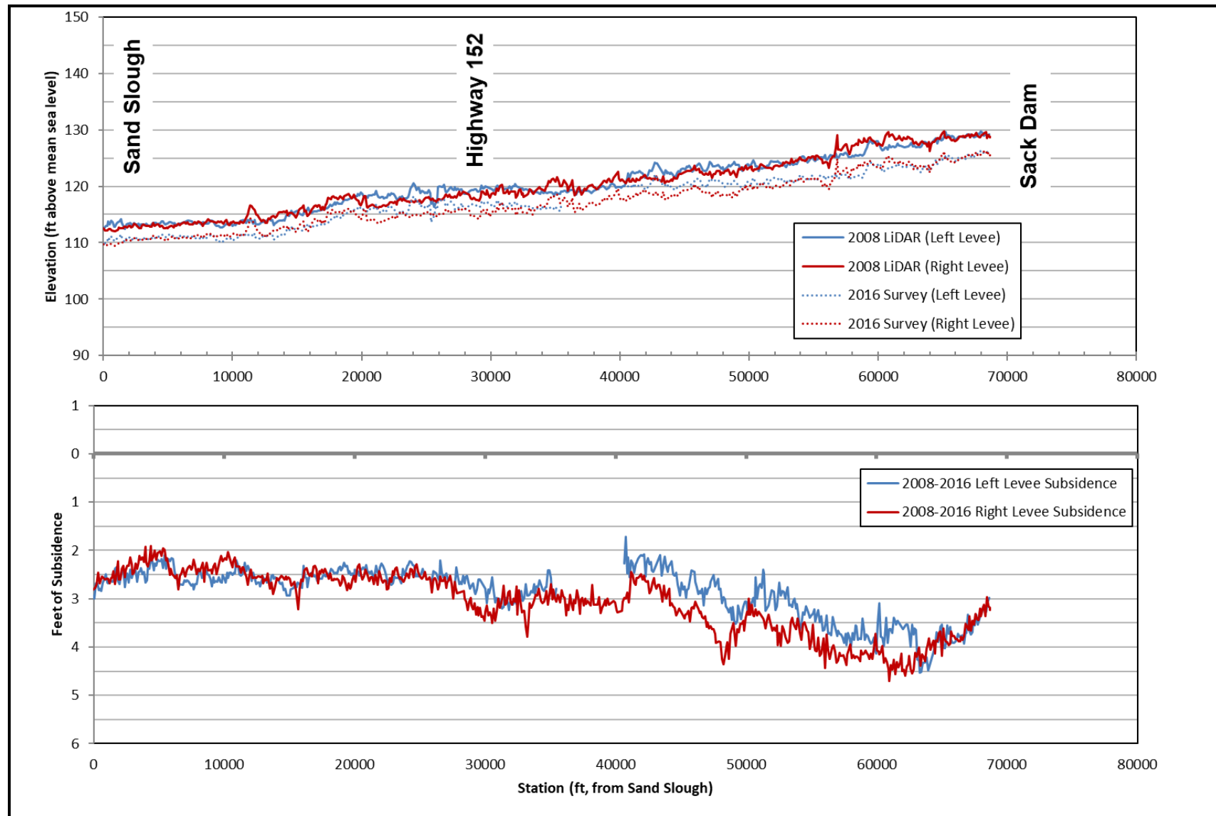
Figure 5 Ground Subsidence along Reach 4A of the San Joaquin River (2008–2016)
