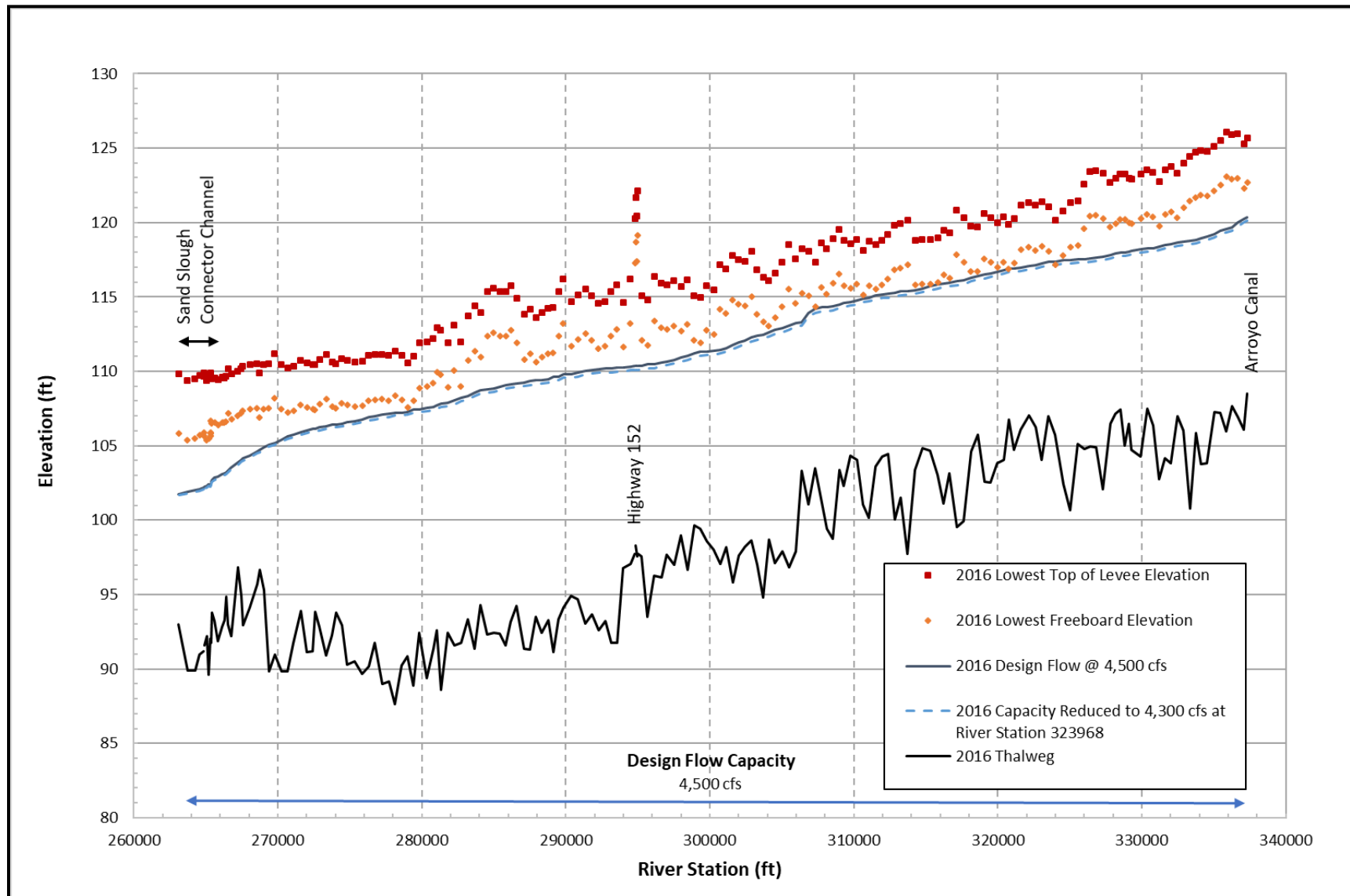
Figure 18 Water Surface Profile for 2016 Run-of-the-River Condition for Reach 4A from Arroyo Canal to Sand Slough
