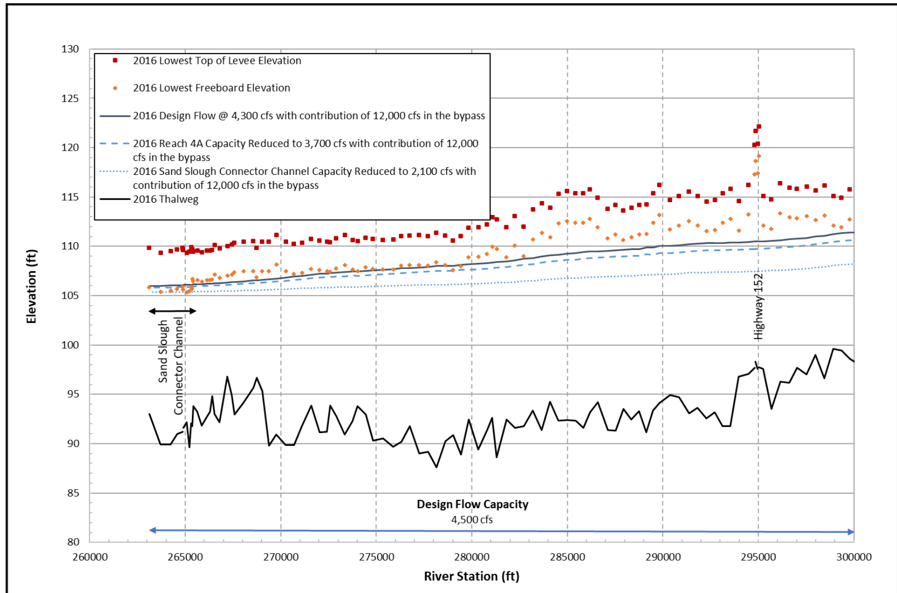
Figure 19 Water Surface Profile for 2016 Backwater Condition for Reach 4A from Highway 152 to Sand Slough
