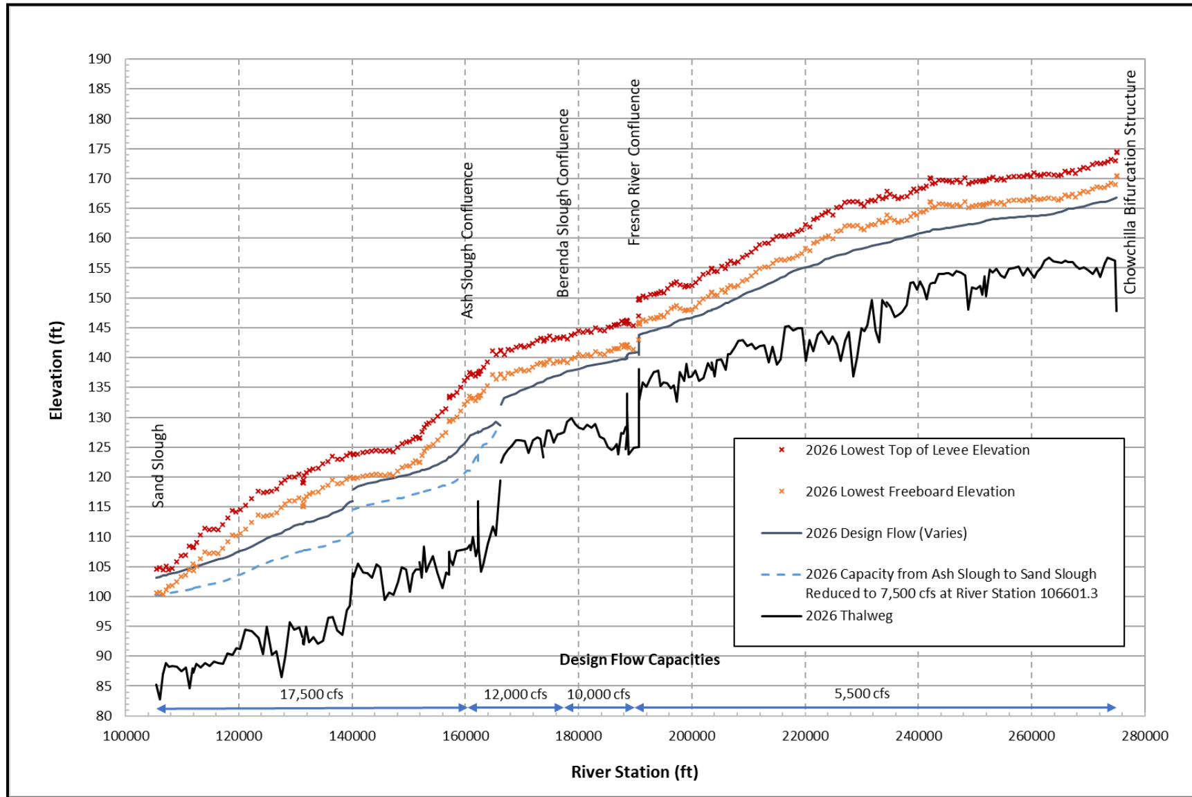
Figure 14 Water Surface Profile for 2026 Run-of-the-River Condition for the Chowchilla and Eastside Bypasses from Chowchilla Bifurcation Structure to Sand Slough
