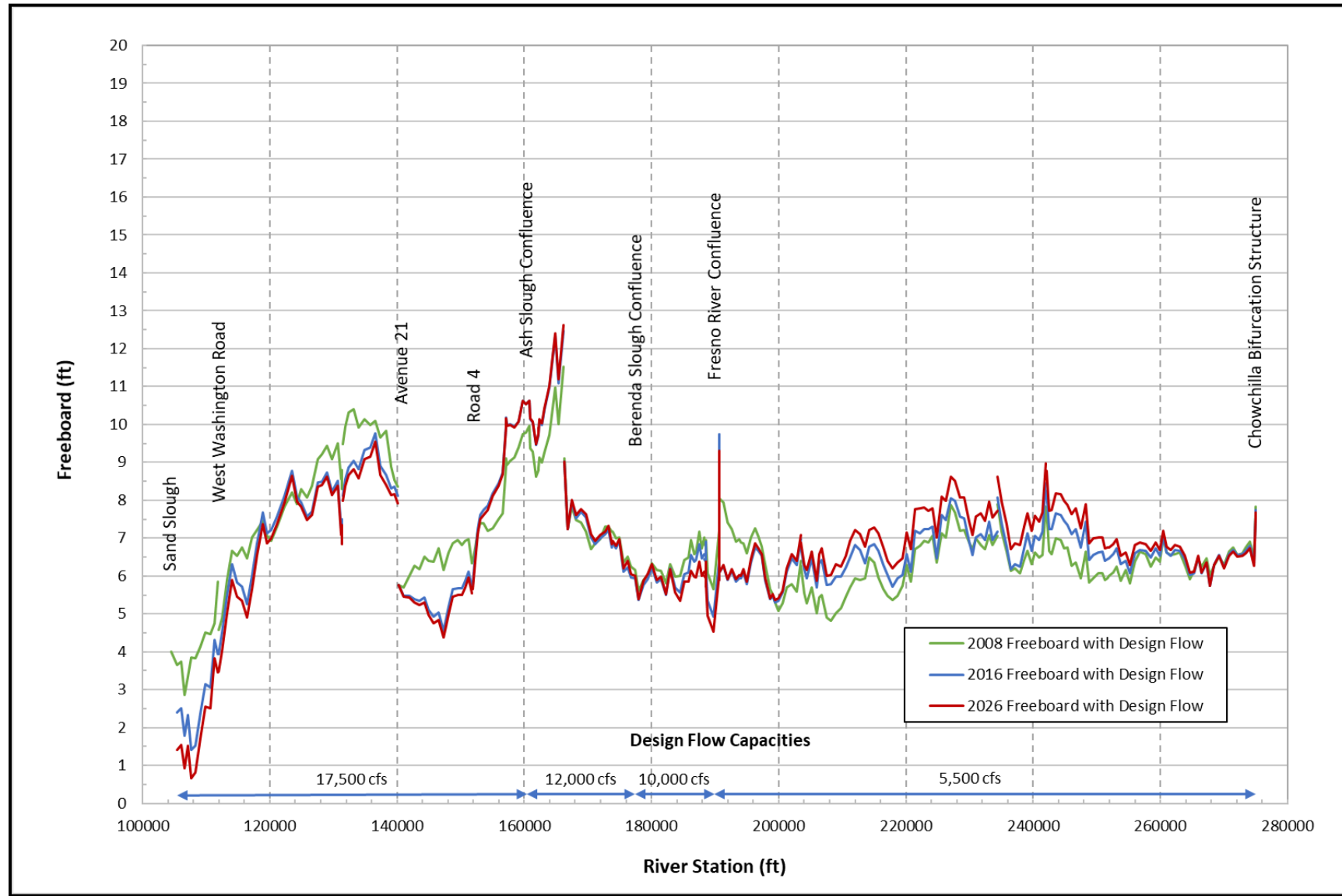
Figure 7 Freeboard Conditions under 2008, 2016, and 2026 Run-of-the-River Conditions in Chowchilla and Eastside Bypasses from the Chowchilla Bifurcation Structure to Sand Slough, based on Design Flow Capacities
