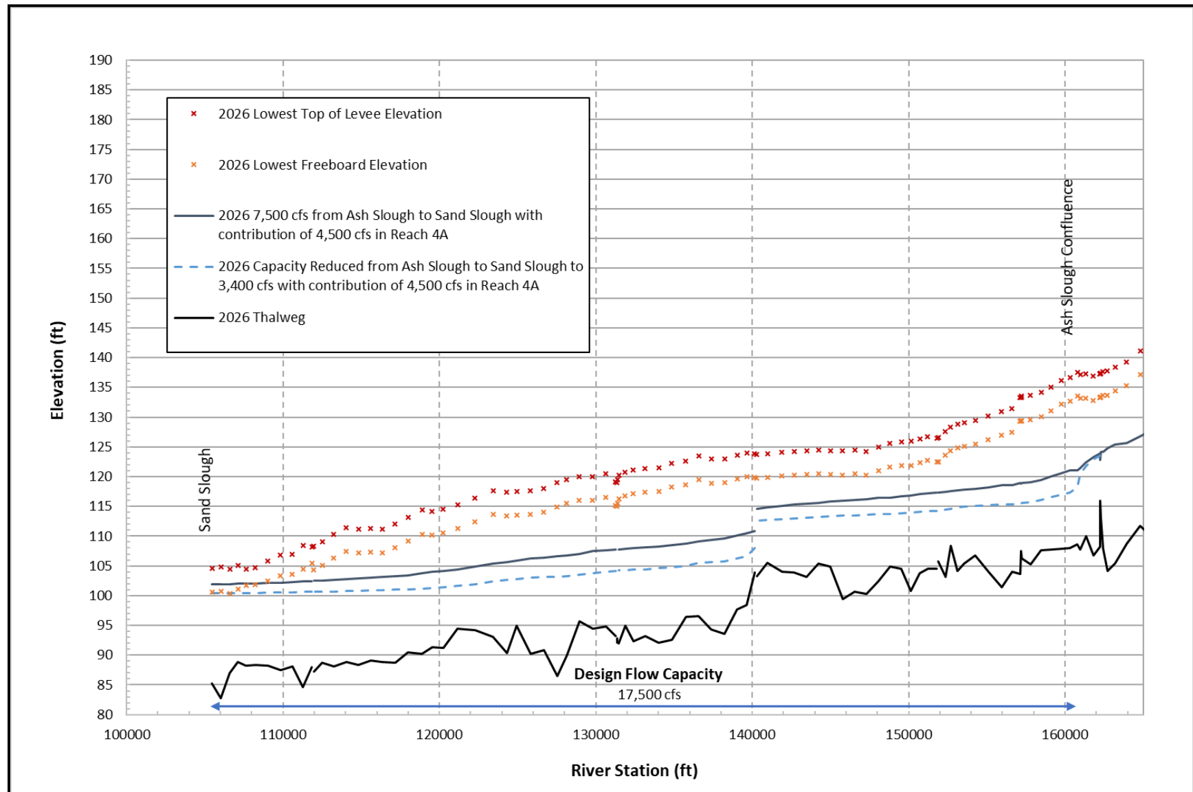
Figure 15 Water Surface Profile for 2026 Backwater Condition for the Eastside Bypass from the Ash Slough Confluence to Sand Slough
