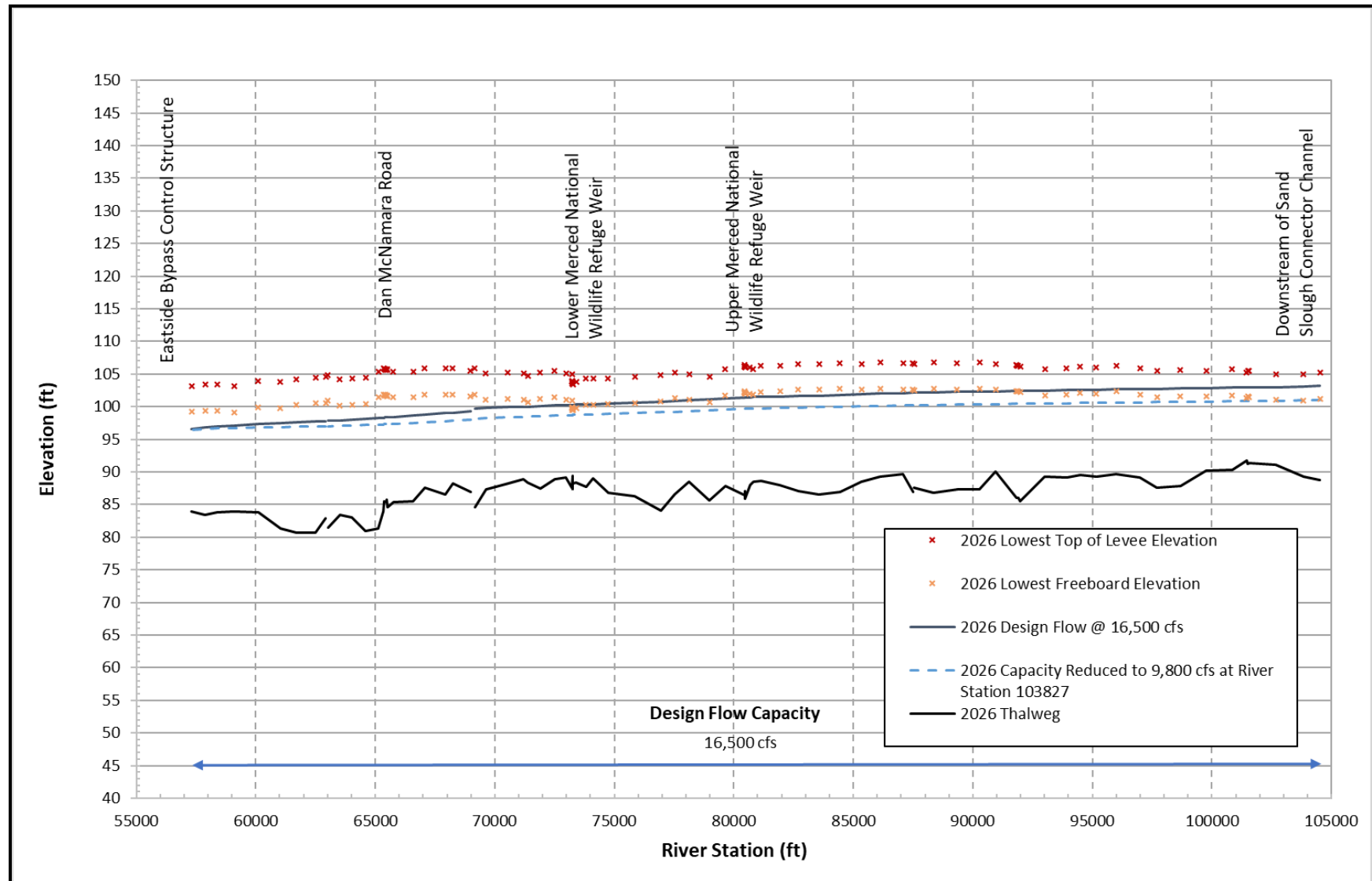
Figure 17 Water Surface Profile for 2026 Run-of-the-River Condition for the Eastside Bypass from Sand Slough to the Eastside Bypass Control Structure
