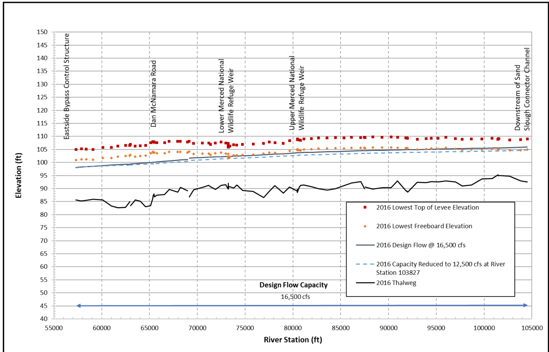
Figure 16 Water Surface Profile for 2016 Run-of-the-River Condition for the Eastside Bypass from Sand Slough to the Eastside Bypass Control Structure
