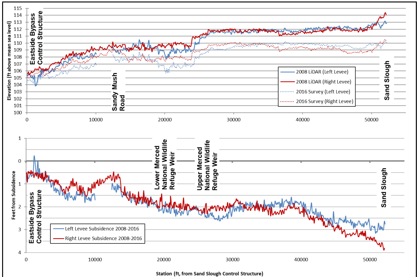
Figure 4 Ground Subsidence along the Eastside Bypass from Sand Slough to the Eastside Bypass Control Structure (2008–2016)
