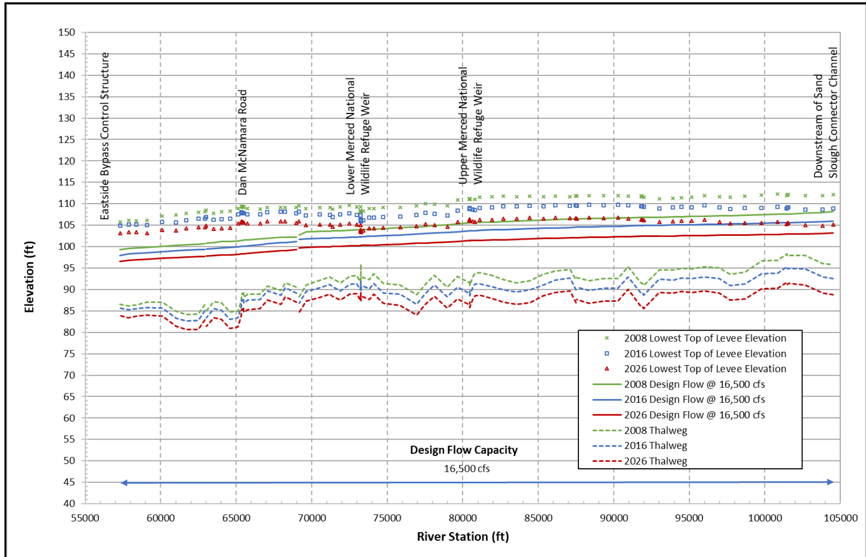
Figure 8 Design Flow Profile under 2008, 2016, and 2026 Run-of-the-River Conditions in the Eastside Bypass from Sand Slough to the Eastside Bypass Control Structure
