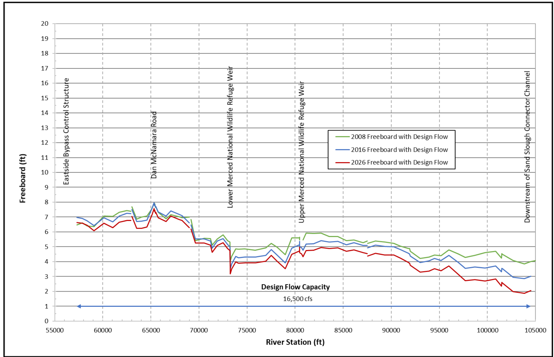
Figure 9 Freeboard Conditions for 2008, 2016 and 2026 Run-of-the-River Conditions for Eastside Bypass from Sand Slough to the Eastside Bypass Control Structure, based on Design Flow Capacities
