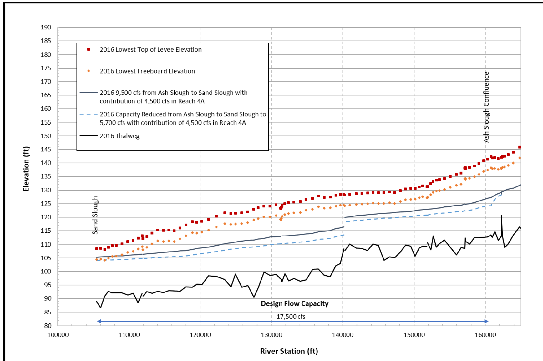
Figure 13 Water Surface Profile for 2016 Backwater Condition for the Eastside Bypass from the Ash Slough Confluence to Sand Slough
