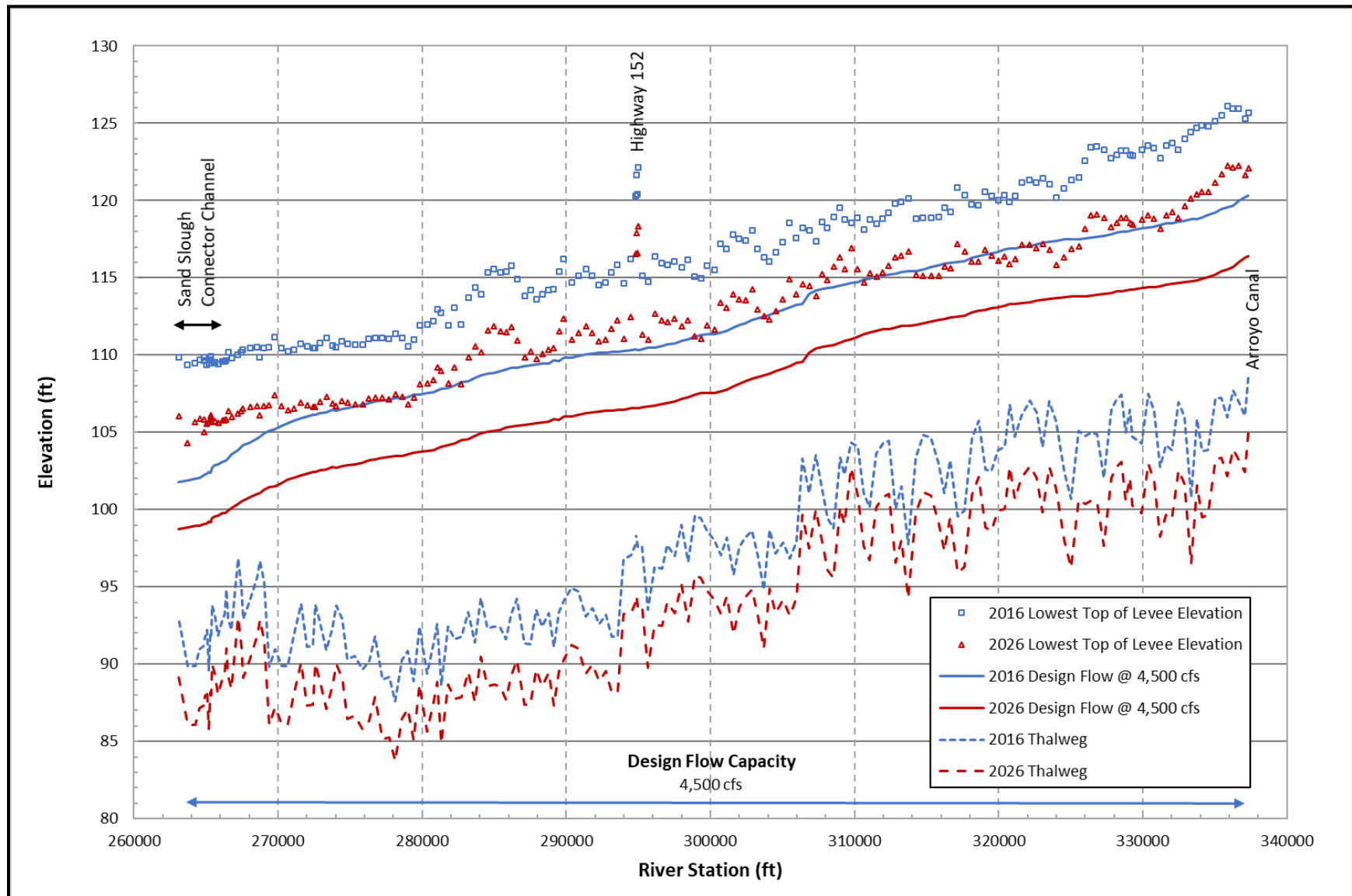
Figure 10 Design Flow Profile under 2016 and 2026 Run-of-the-River Conditions in Reach 4A of the San Joaquin River
