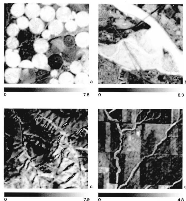
Fig. 1. Surface Energy Balance Algorithm for Land estimates of evapotranspiration (ET) (mm) for different ecosystems in the Columbia River basin (Washington State) on June 25, 2000. Part A consist of irrigated pivots (119°35'51" W;46°03'13" N). Part B is riparian vegetation at the confluence of the Yakima and the Colombia (119°14'14" W,46°15'07" N). Part C is the forests near Pendleton (118°53'30" W,45°20'39" N), and Part D consists of rangeland (119°33'25" W,46°13'48" N). The range in actual ET varies (mm·d -1 for every subimage and is specified underneath every panel.
