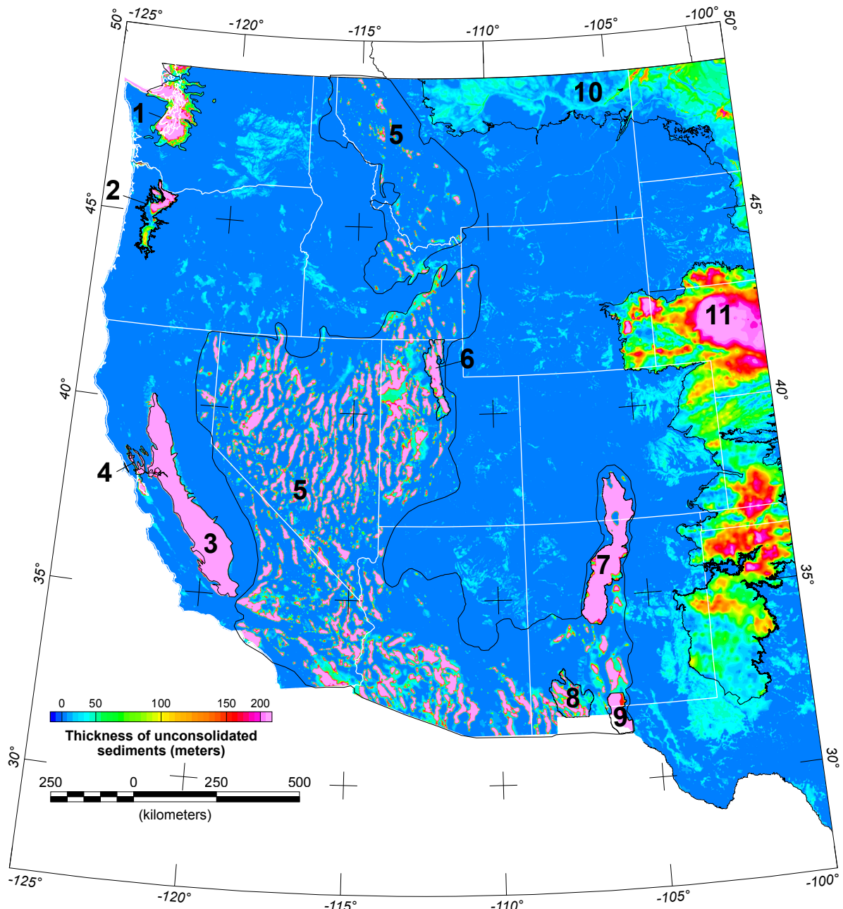
Figure 2. Thickness of unconsolidated sediments combined from Pelletier and others (2016) and regional models. Note that the color scale is different than that used in figure 1. Polygons show bounds of regional models—1, Puget Sound; 2, Portland and Willamette Basins; 3, Central Valley of California; 4, northern San Francisco Bay; 5, Basin and Range; 6, Salt Lake Valley; 7, San Luis and Albuquerque Basins; 8, Mimbres Basin; 9, Hueco Bolson; 10, glacial deposits east of the Rocky Mountains; 11, High Plains. White lines represent State boundaries.
