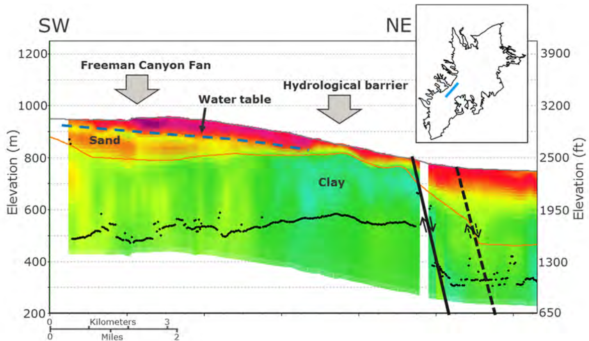
Figure 6-15. Cross-section showing the SkyTEM data, where the resistivity shows fine materials nearly reaching the surface
