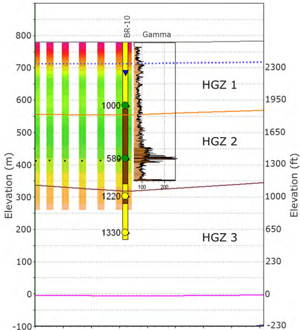
Figure 4-7. Illustration of the interpretation of available data sources in GeoScene3D software
