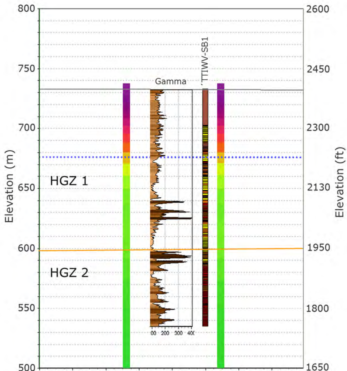
Figure 4-6. Example of well log from well TTIWV-SB1 in GeoScene3D used for the interpretation of the HCF. The gamma signal is filled, with the darker the fill the higher the clay content. The colored bars show the SkyTEM resistivity and the dotted blue line shows the interpolated water table from the SkyTEM data. The bottom of HGZ 1 is the orange line and the bottom of HGZ 2 is the brown line.
