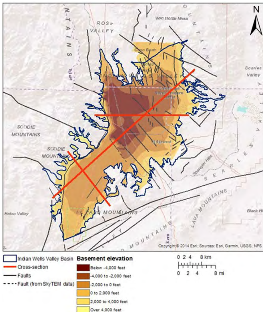
Figure 5-2. Elevation of the basement (granite/bedrock) for the Indian Wells Valley groundwater basin The black lines show the location of the faults mapped out by the USGS. The dashed black lines show an extension of two mapped faults, based upon SkyTEM data. These two faults define the boundary to the El Paso area, which encompasses the southwest portion of the Indian Wells Valley groundwater basin. The red lines show the location of the three cross-sections cutting across the basin. Elevations are with respect to mean sea level.
