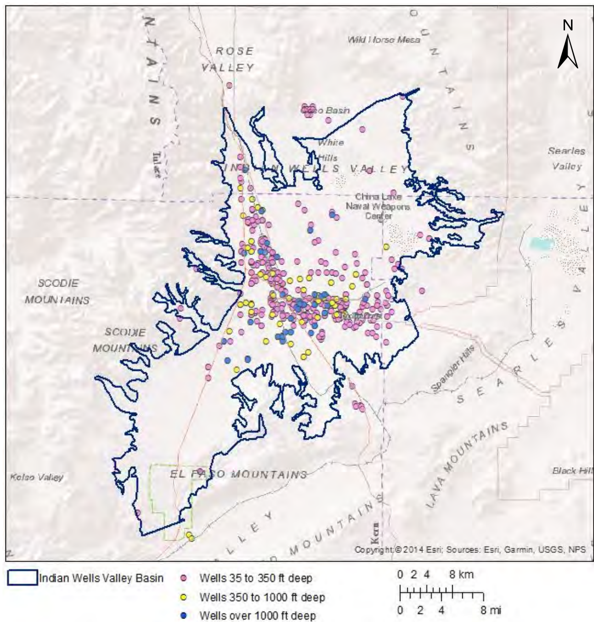
Figure 3-1. Map showing the location of the wells that were used in the interpretation of the HCF Each dot represents locations of wells within a specified depth range. There may be several wells with the same coordinates.
