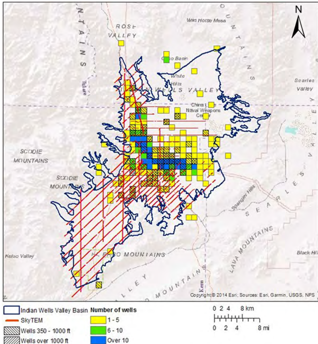
Figure 7-1. Map showing the number of wells per square mile and SkyTEM data within the Indian Wells Valley groundwater basin
