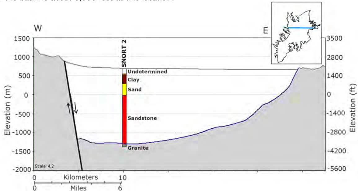
Figure 5-3. Cross-section from west to east showing the structure of the China Lake area The Sierra Nevada frontal fault defines the western boundary of the basin. The SNORT 2 well is one of the few wells in the basin that reaches the granite in the basin floor.
