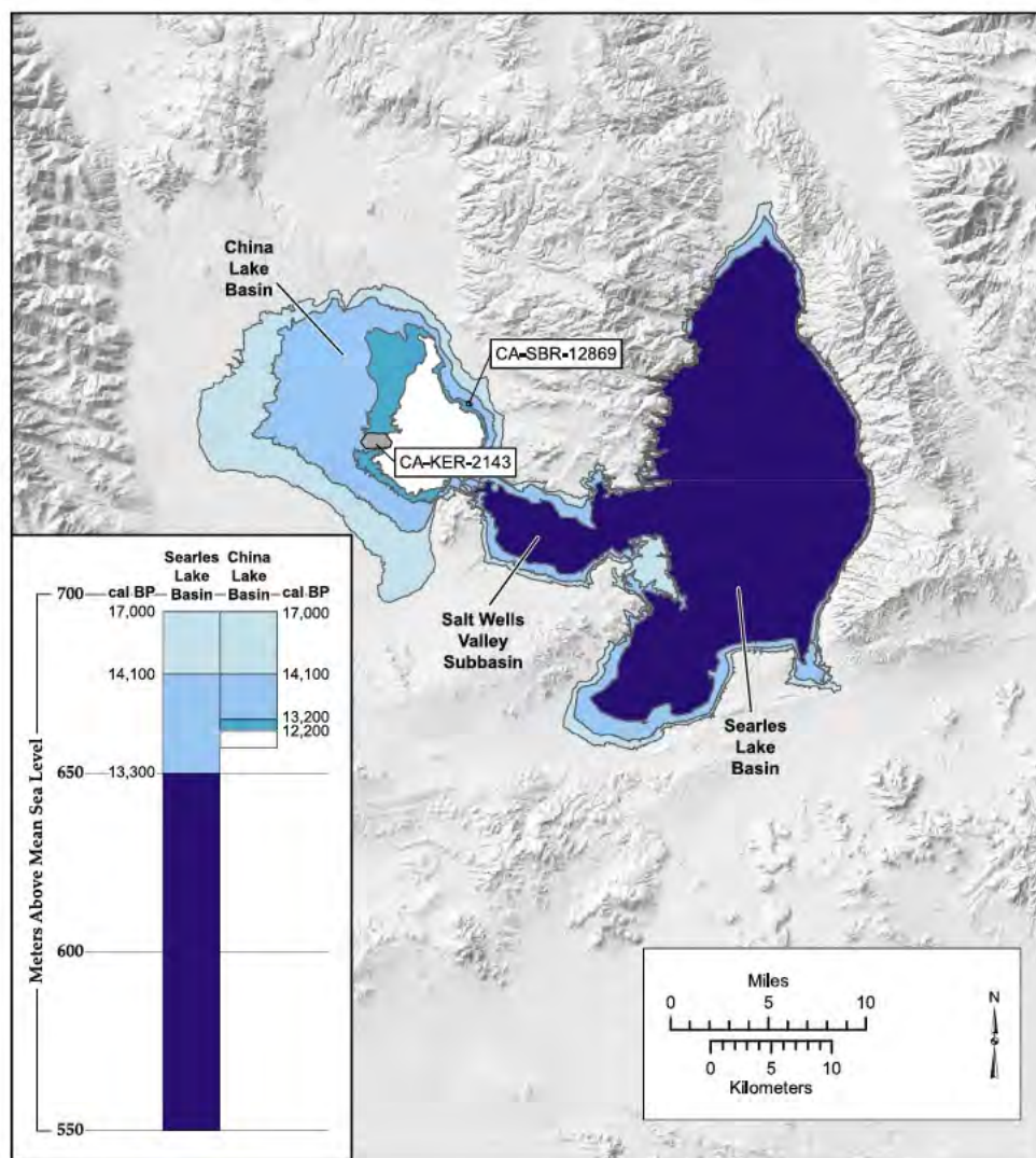
Figure 2-6. High stands of China, Salt Wells and Searles pluvial lakes
