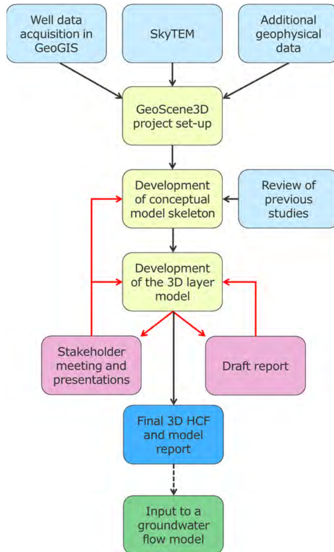
Figure 4-1. Diagram illustrating the workflow in the development of the HCF
