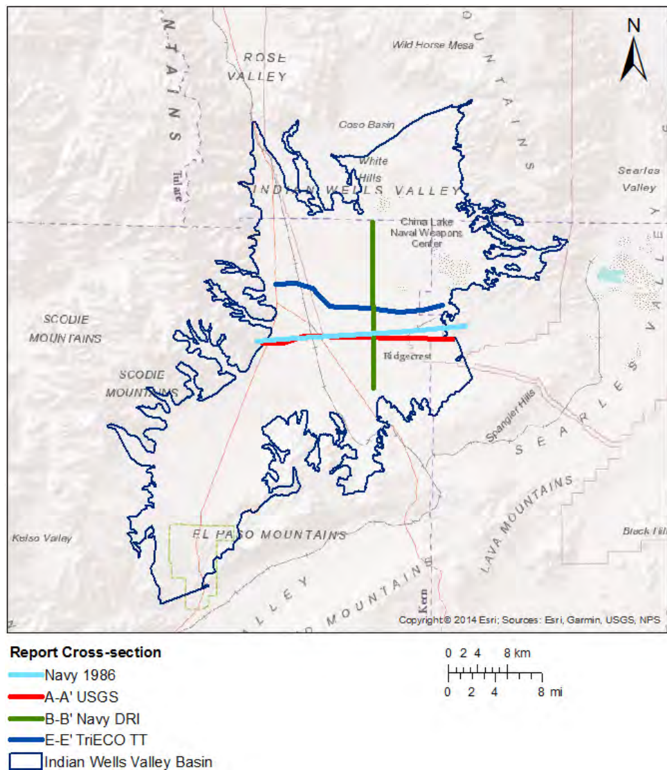
Figure A2.1 Location of the four cross-sections shown in Appendix 2 figures.
