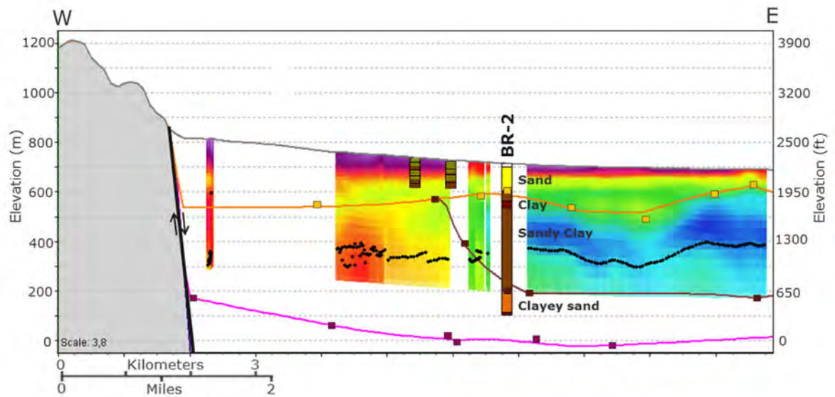
Figure 4-3. Cross-section showing SkyTEM resistivity measurements combined with the lithology from the three different wells The squares show where the interpretation points were placed in relation to the data. The small black dots show the depth of investigation (DOI) for the SkyTEM data. The lithology for well BR-2 is provided. The colored lines show the interpreted hydrogeologic zones, which will be discussed later in the report.
