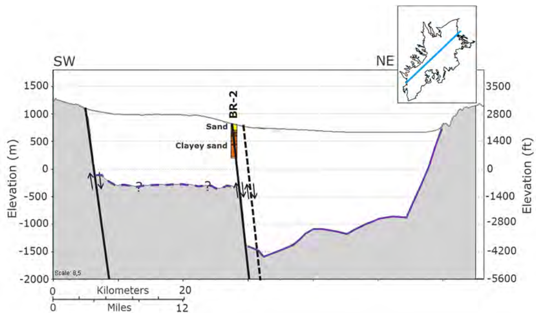
Figure 5-5. Cross-section across the entire Indian Wells Valley groundwater basin, from southwest to northeast The Sierra Nevada frontal fault is shown in the southwestern part of the cross-section. The fault dividing the China Lake area to the north and the El Paso area to the southwest is shown in the middle of the cross-sections. The dashed line shows an inferred extension of a second fault based upon SkyTEM data. Well BR-2, shown on the cross-section, is one of the deepest wells in the area. The bottom of the basin southwest of the mid-basin fault is estimated.
