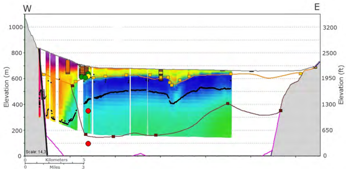
Figure 4-5. Cross-section showing SkyTEM resistivity measurements combined with lithology and measured TDS (large circles)
