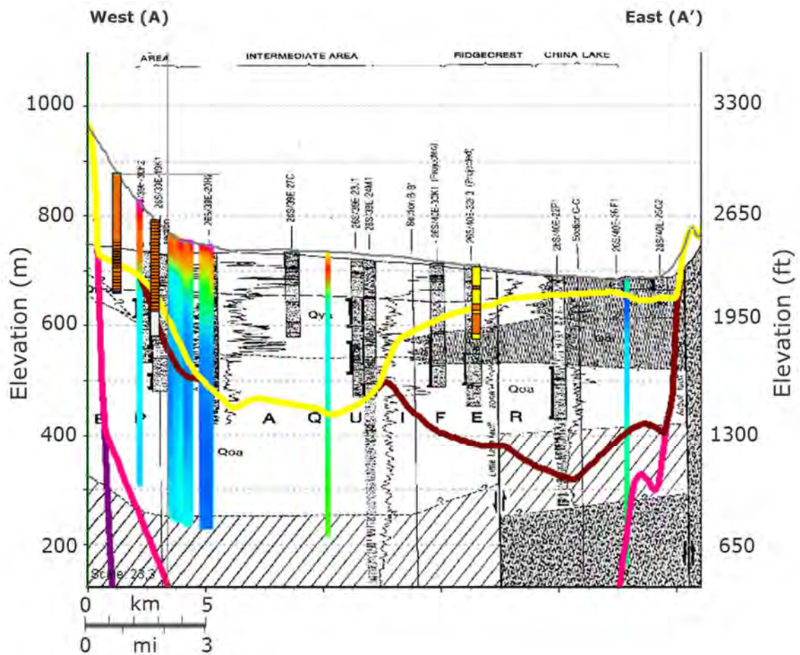
Figure A2.3 Cross-section A-A' from the USGS Water-Resources Investigations Report 89-4191, from 1989 (Brenbrock and Martin, 1989).
