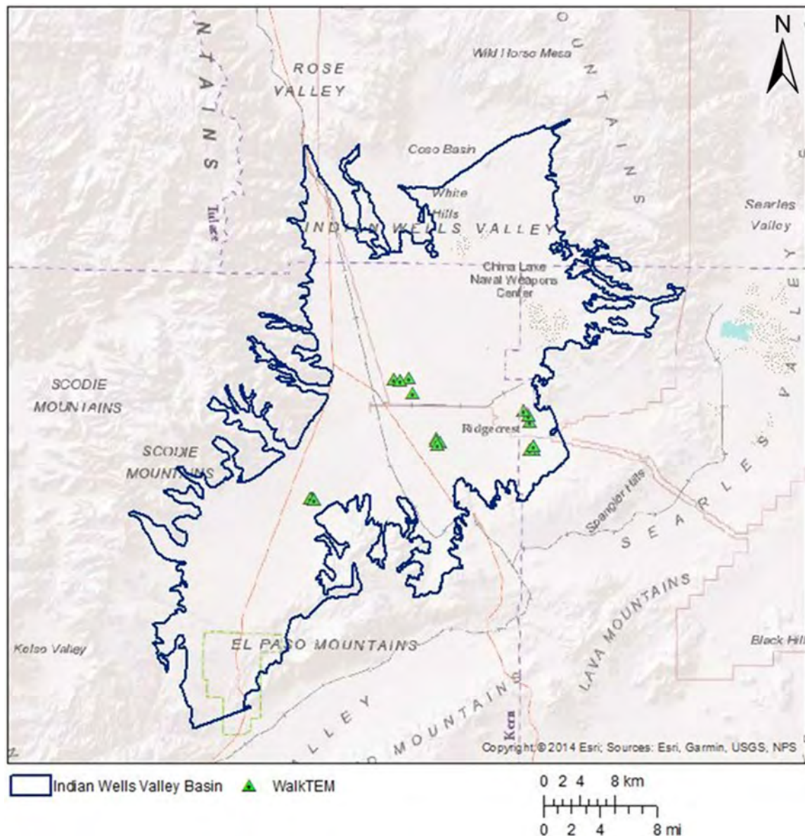
Figure 3-6. Location of the WalkTEM soundings.
