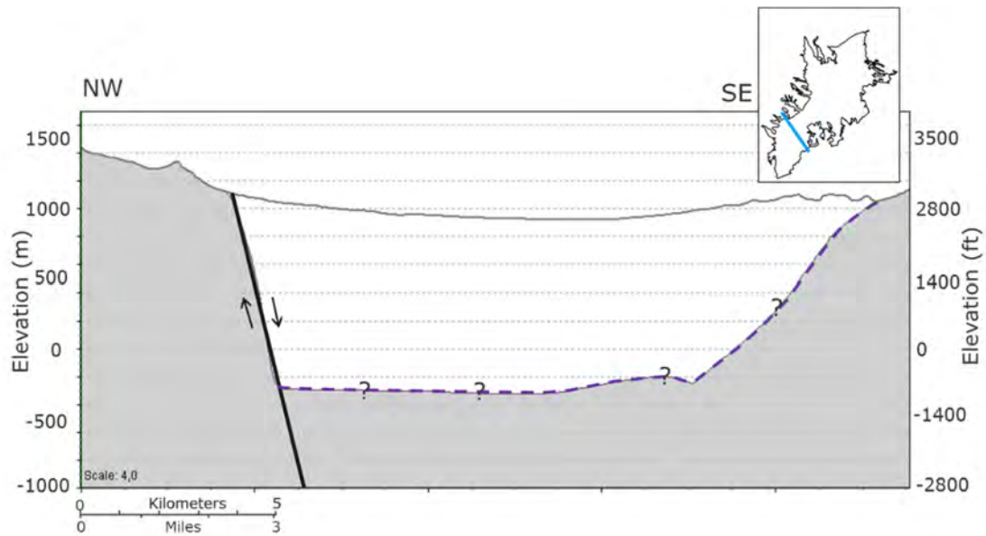
Figure 5-4. Cross-section from northwest to southeast showing the structure in the El Paso area The Sierra Nevada frontal fault defines the northwestern boundary of the area. The bottom of the basin is only estimated as there are no wells or geophysical surveys that can be used to determine the basin bottom.
