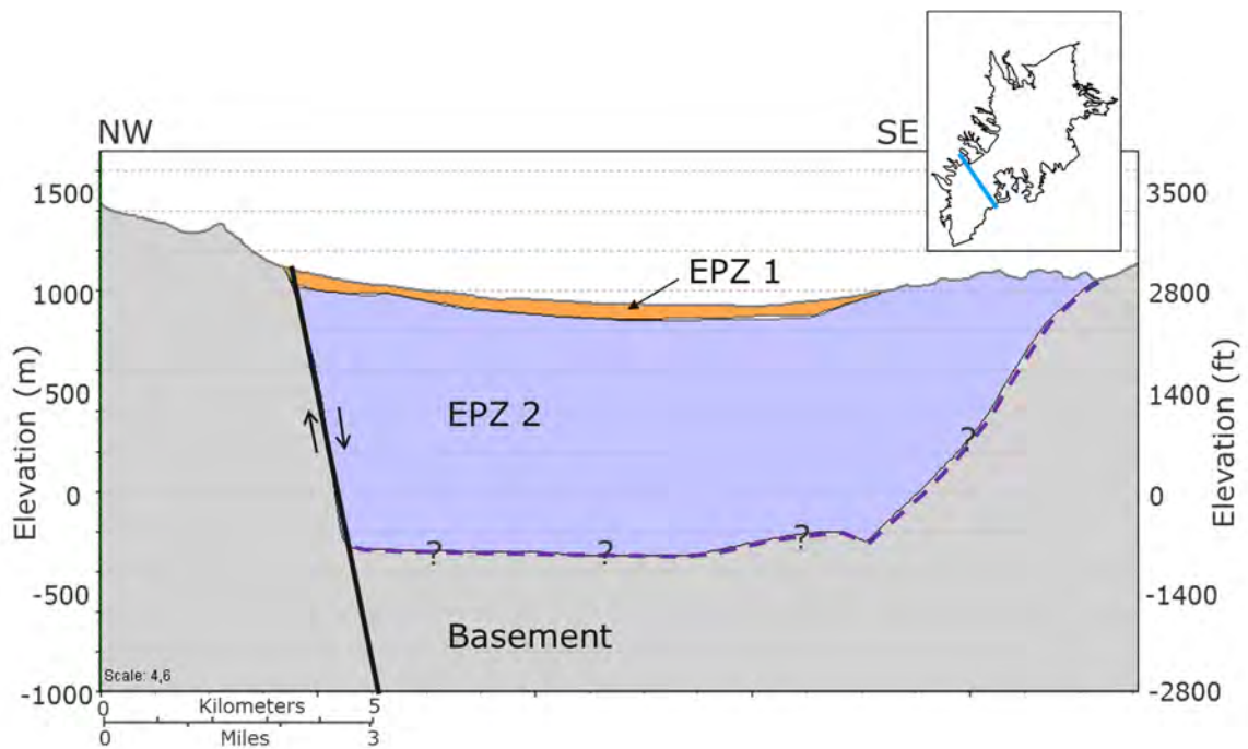
Figure 6-2. Cross-section showing the three different hydrogeologic zones mapped in the El Paso area.
