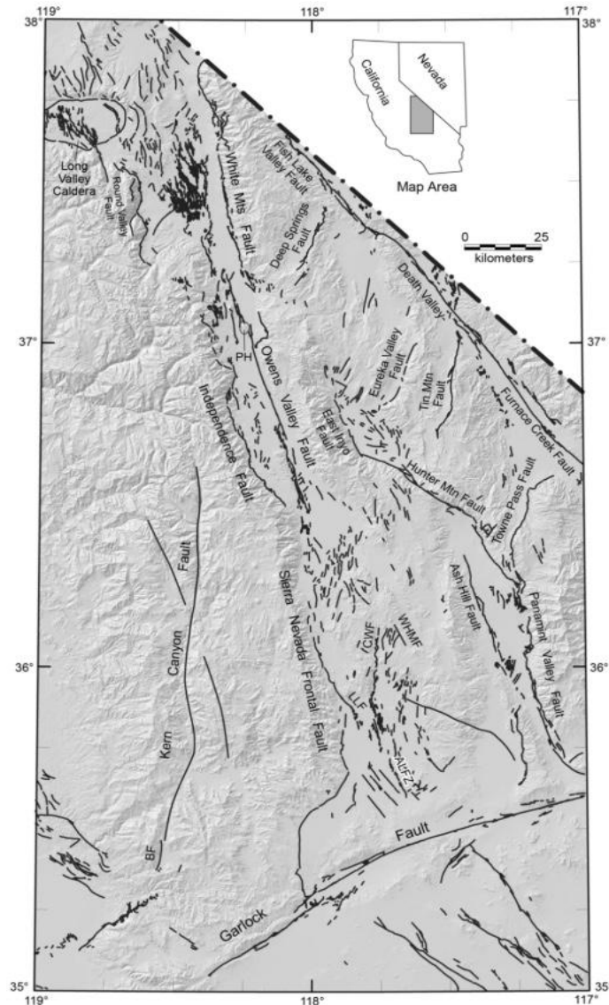
Figure 2-3. Map showing Quaternary faults in east-central California
