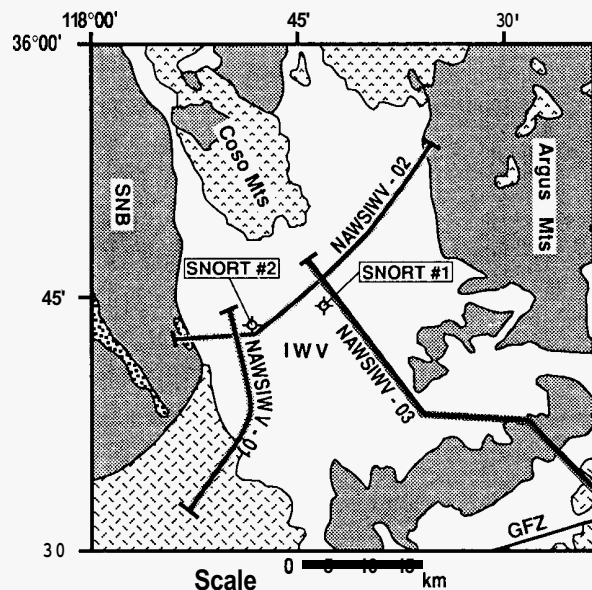
Figure 2. Map showing Indian Wells Valley and surrounding area. Also shown are the locations of the SNORT #1, SNORT #2, and reflection seismic lines designated NAWSIWV-92-01, 02, or 03.
