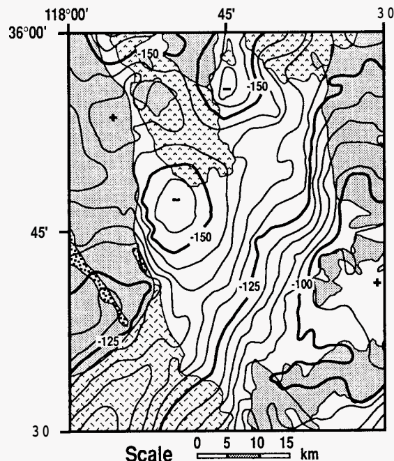
Figure 3. Gravity data for the Indian Wells Valley. Contour interval is 5 milligals. The deep gravity low is located directly beneath the western IWV. Adapted from Nilsen and Chapman, 1971.
