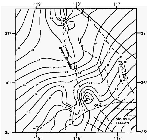
Figure 5. A preliminary Moho depth (km) contour map of east-central California based on forward modeling of PmP travel times from both explosions and earthquake data. The center of the Indian Wells Valley is located beneath 117° 45' W and 35° 45' N (from Malin and Shalev, in prep., data are from the Southern Sierra Crustal Dynamics Project). The outline of the Sierra Nevada and other key physiographic features are shown by the dashed lines; refer to Figure 1 for specific locations. GFZ = Garlock Fault Zone, IWV = Indian Wells Valley.
