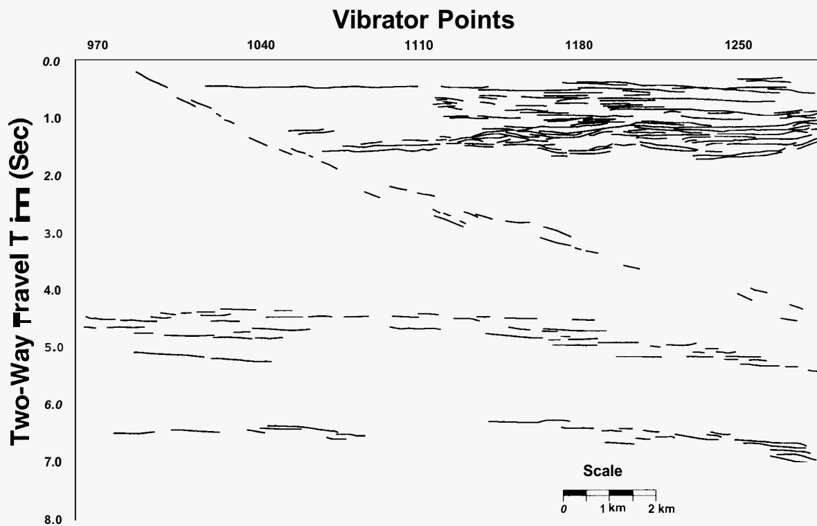
Figure 4. A portion of the western end of NAWSIWV-92-02 reflection seismic line with a line drawing of major reflectors. Vibrator points (V.P.) are 50 meters apart. See text for discussions.
