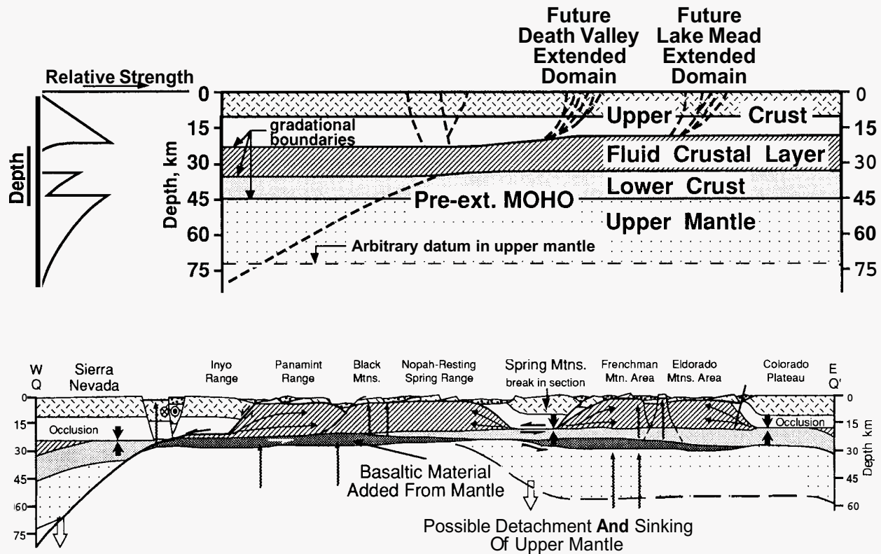
Figure 7. Fluid layer model of Wernicke (1992) as applied to the southwest basin and range. Diagram is an east-west section at approximately 36°N latitude. The model shows flow from within the fluid layer located between the upper and lower crust. Note that flow is predicted from beneath the Sierra Nevada eastward under the mountains to the east with heat passing upward along the strike slip faults. The equivalent position of Coso, if this section were to the south of this location, would be where the Inyo Range is. The datum in the upper mantle is not intended to be either a thermal or mechanical boundary.
