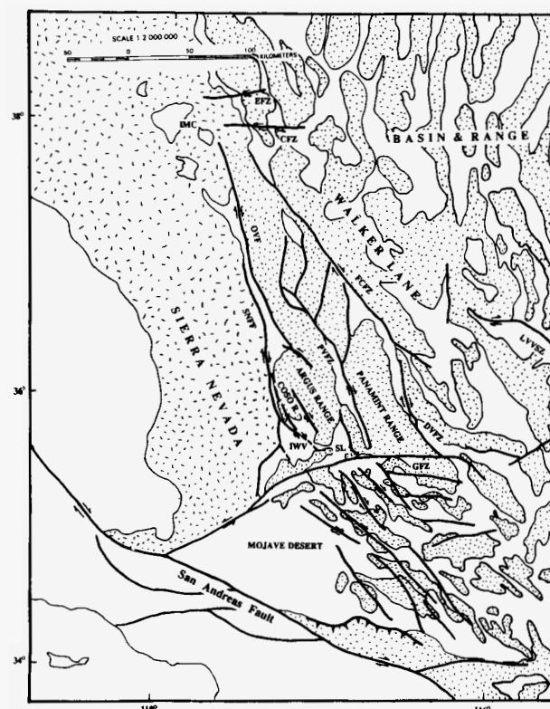
Figure 1. Physiographic map of the western Basin and Range, U.S.A. Significant features discussed in the text include: DVFZ-Death Valley Fault Zone, GFZ-Garlock Fault Zone, IWV-Indian Wells Valley, PVFZ-Panamint Valley Fault Zone (from Monastero, 1992). The Panamint Valley proper lies immediately west of the PVFZ.
