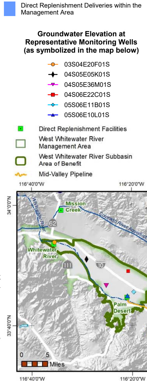
Hydrographs and Direct Replenishment, for the West Whitewater River Subbasin Management Area 2009-2019
