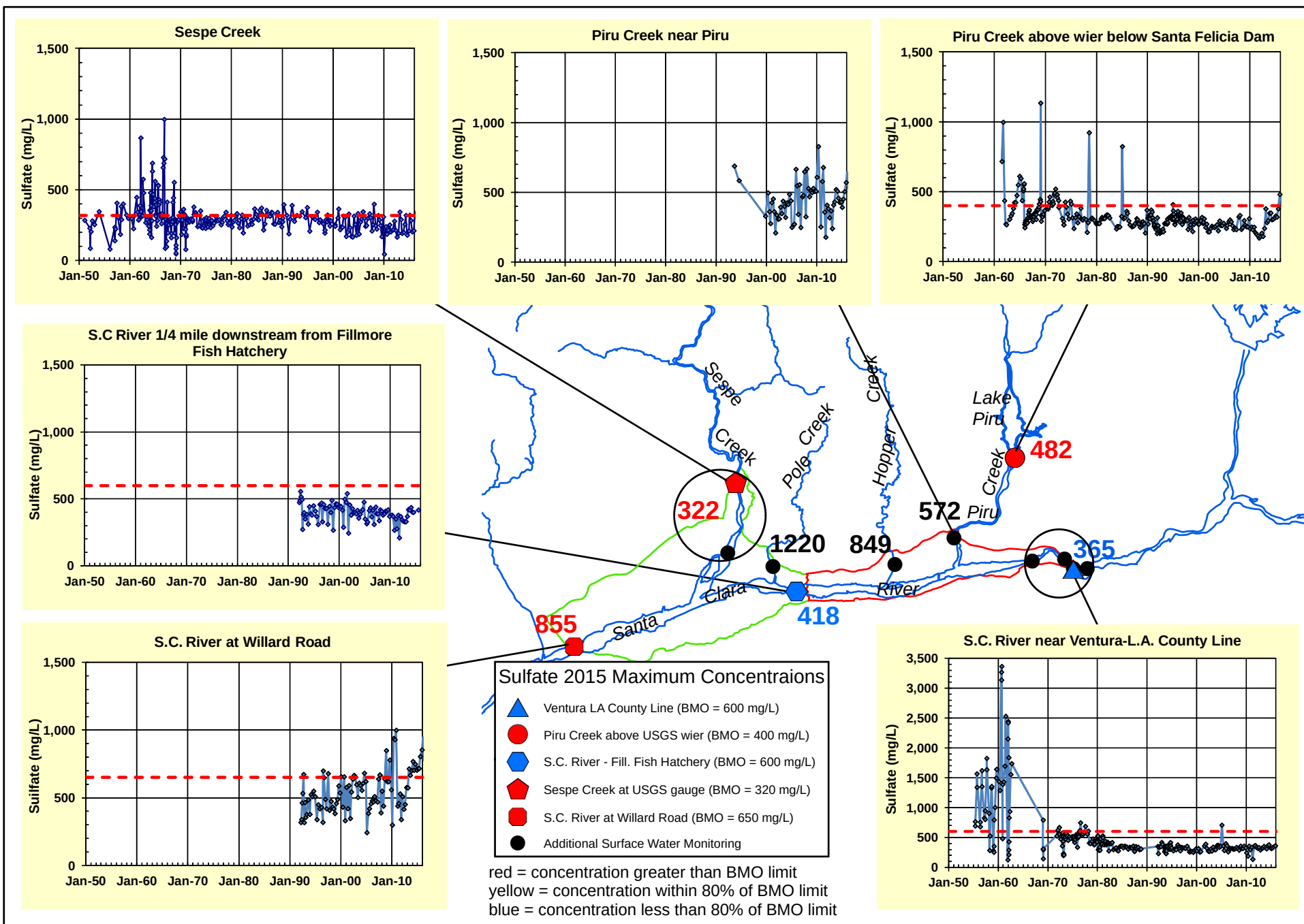
Figure 27. Sulfate surface water quality time series graphs with map of 2015 maximum concentrations in mg/L (black circles denote alternate sample sites); dashed red line is the BMO based on surface water quality objectives from the LRWQCB-LA Basin Plan, 1994.
