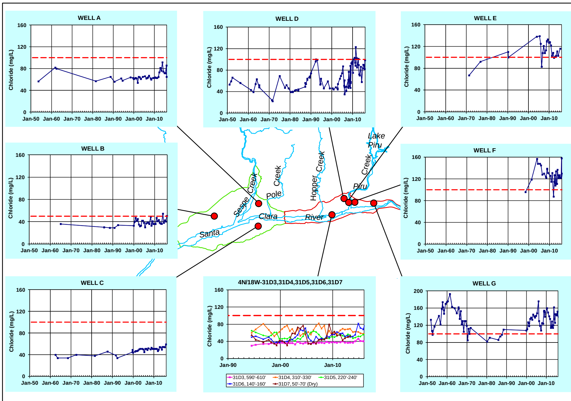
Figure 38. Chloride groundwater quality time series graphs (mg/L); dashed red line is the BMO.
