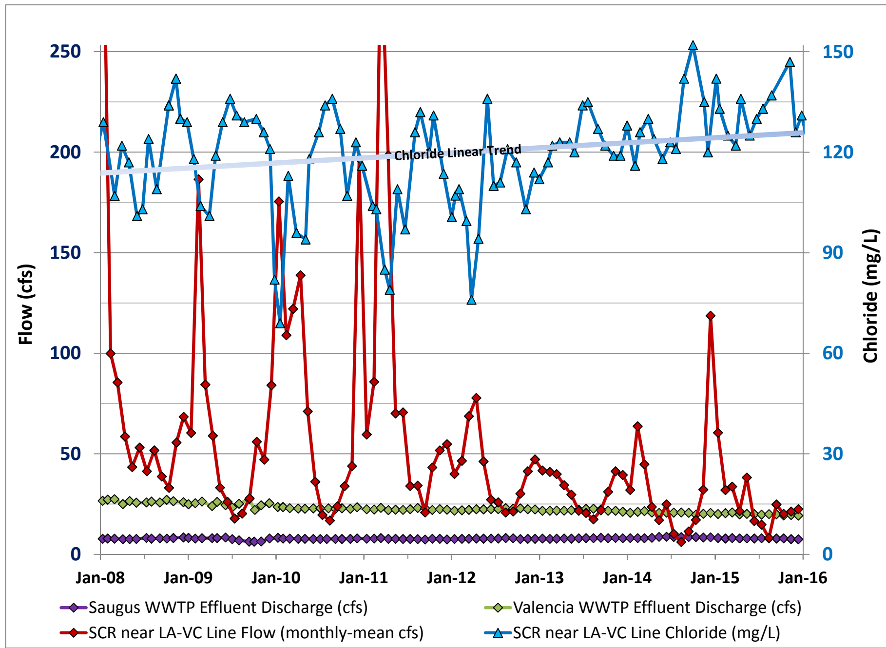
Figure 43. Saugus and Valencia WWTPs effluent (NPDES); Santa Clara River flow and chloride concentration near the Ventura/ Los Angeles County Line.
