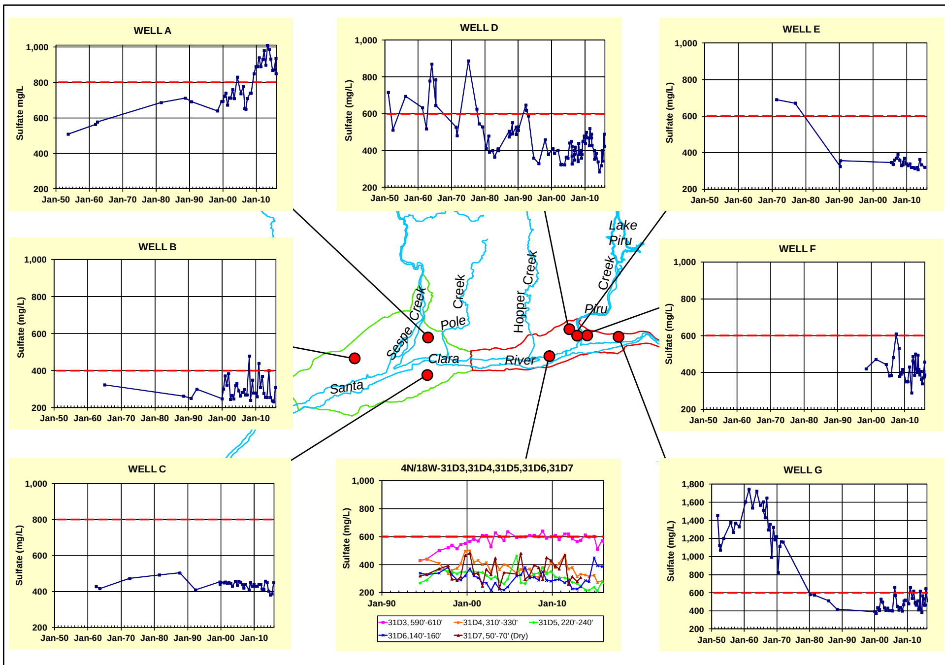
Figure 37. Sulfate groundwater quality time series graphs (mg/L); dashed red line is the BMO.
