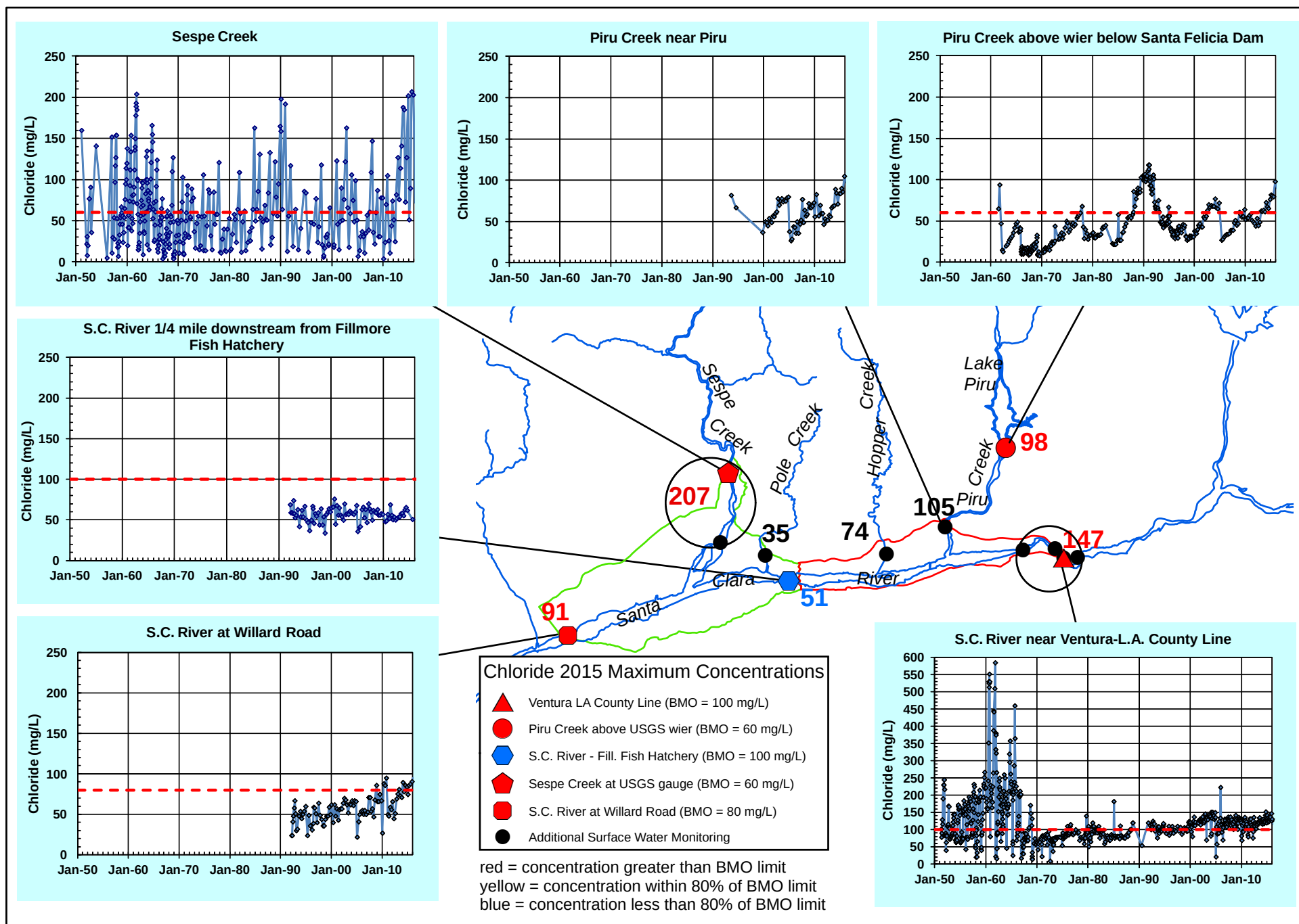
Figure 28. Chloride surface water quality time series graphs with map of 2015 maximum concentrations in mg/L (black circles denote alternate sample sites); dashed red line is the BMO based on surface water quality objectives from the RWQCB-LA Basin Plan, 1994.
