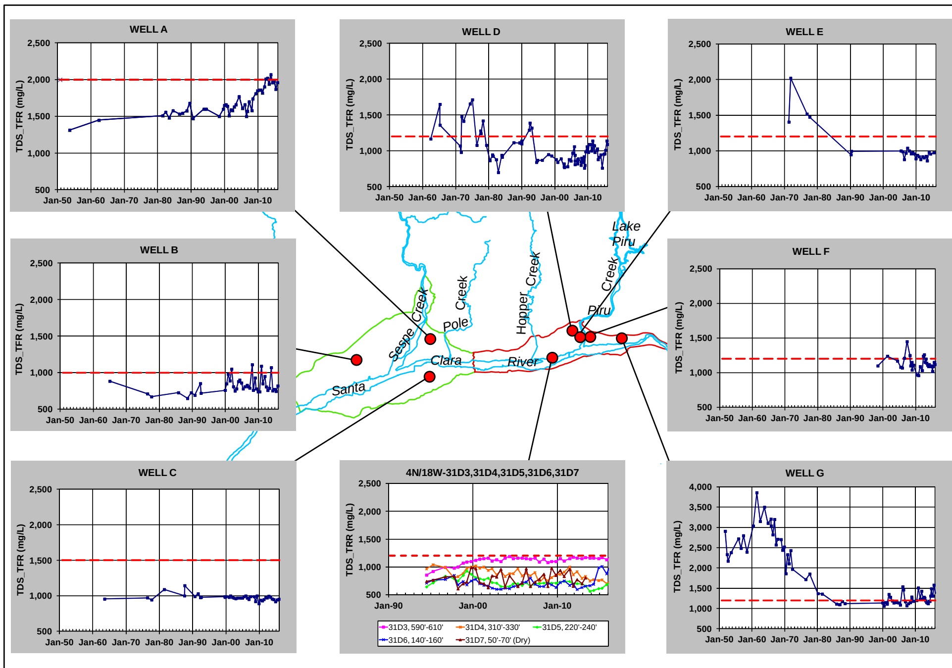
Figure 36. TDS groundwater quality time series graphs (mg/L); dashed red line is the BMO.
