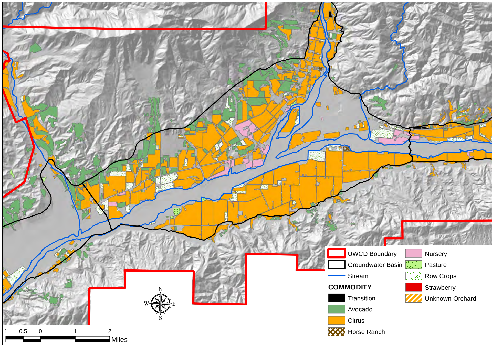
Figure 47. Fillmore basin agricultural land use map for 1997 with hillshade base.
