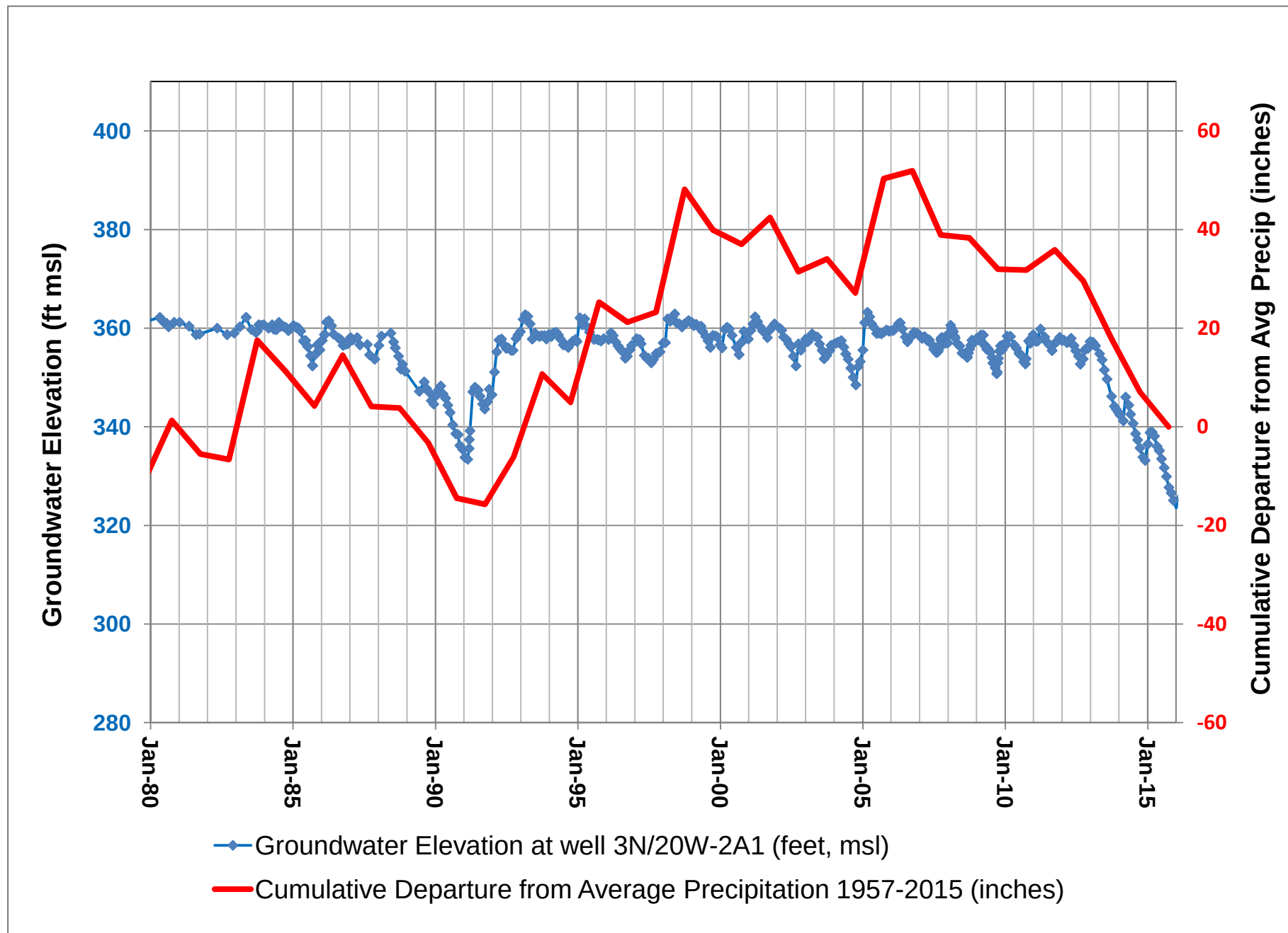
Figure 20. Groundwater elevations and cumulative departure from average precipitation for the Fillmore basin.
