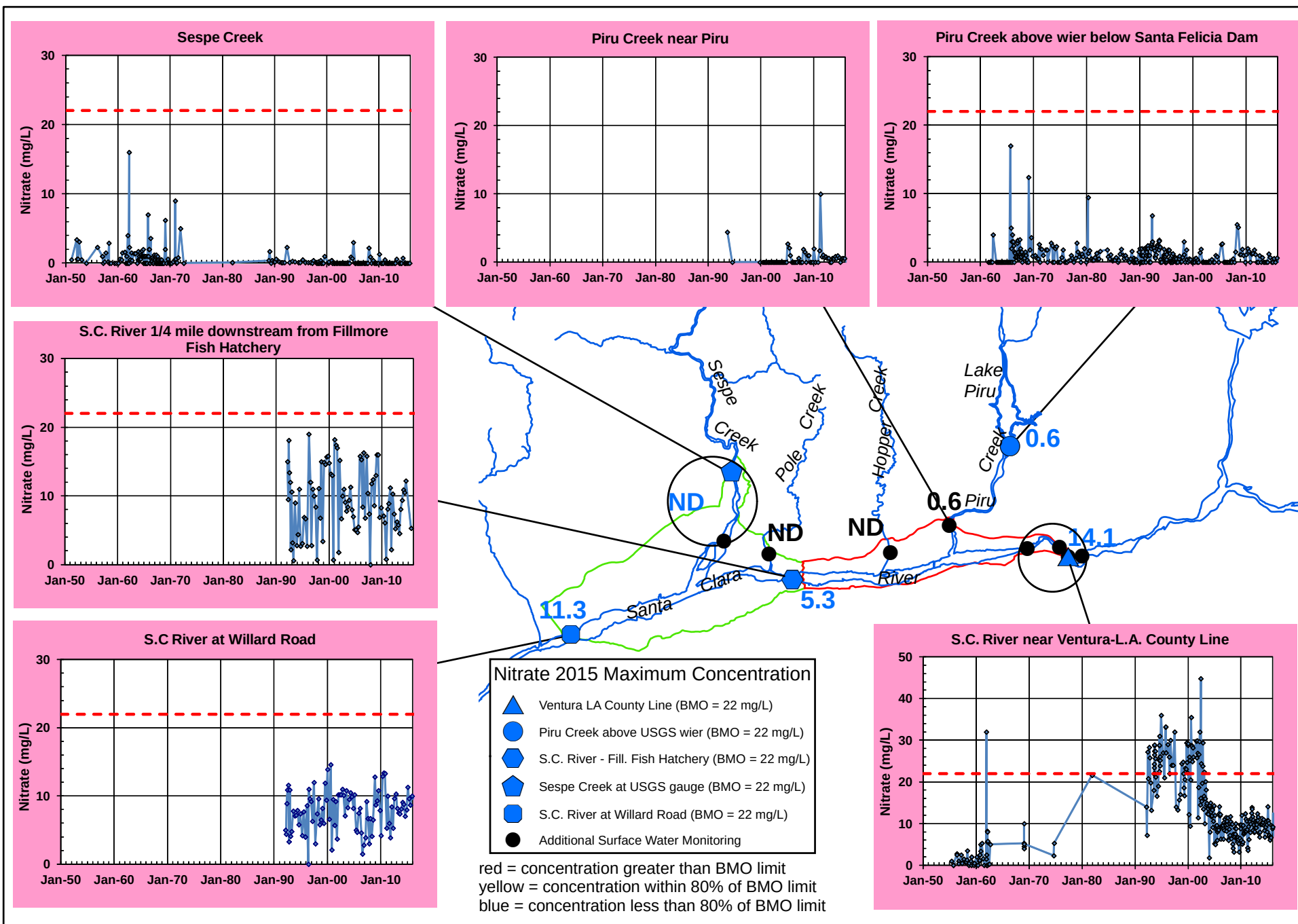
Figure 29. Nitrate surface water quality time series graphs with map of 2015 maximum concentrations in mg/L (black circles denote alternate sample sites); dashed red line is the BMO based on surface water quality objectives from the RWQCB-LA Basin Plan, 1994.
