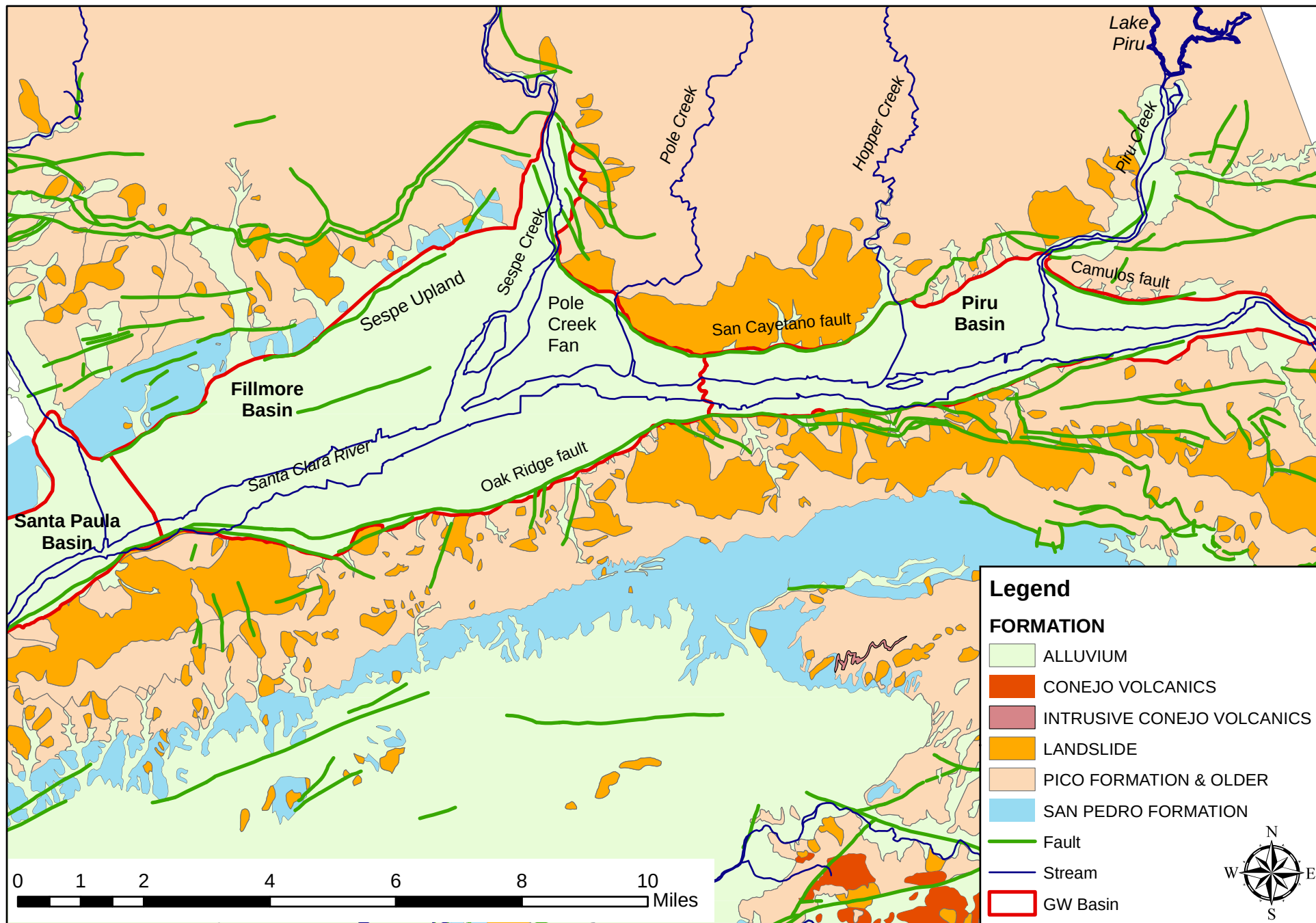
Figure 2. Surface geology map.
