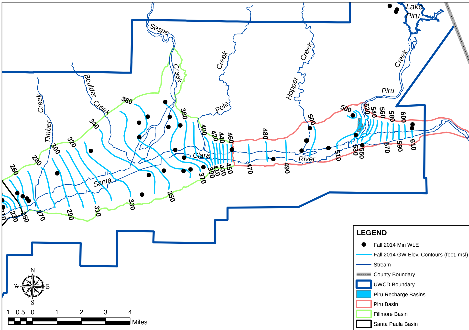
Figure 4. Fall 2014 groundwater elevation contours.
