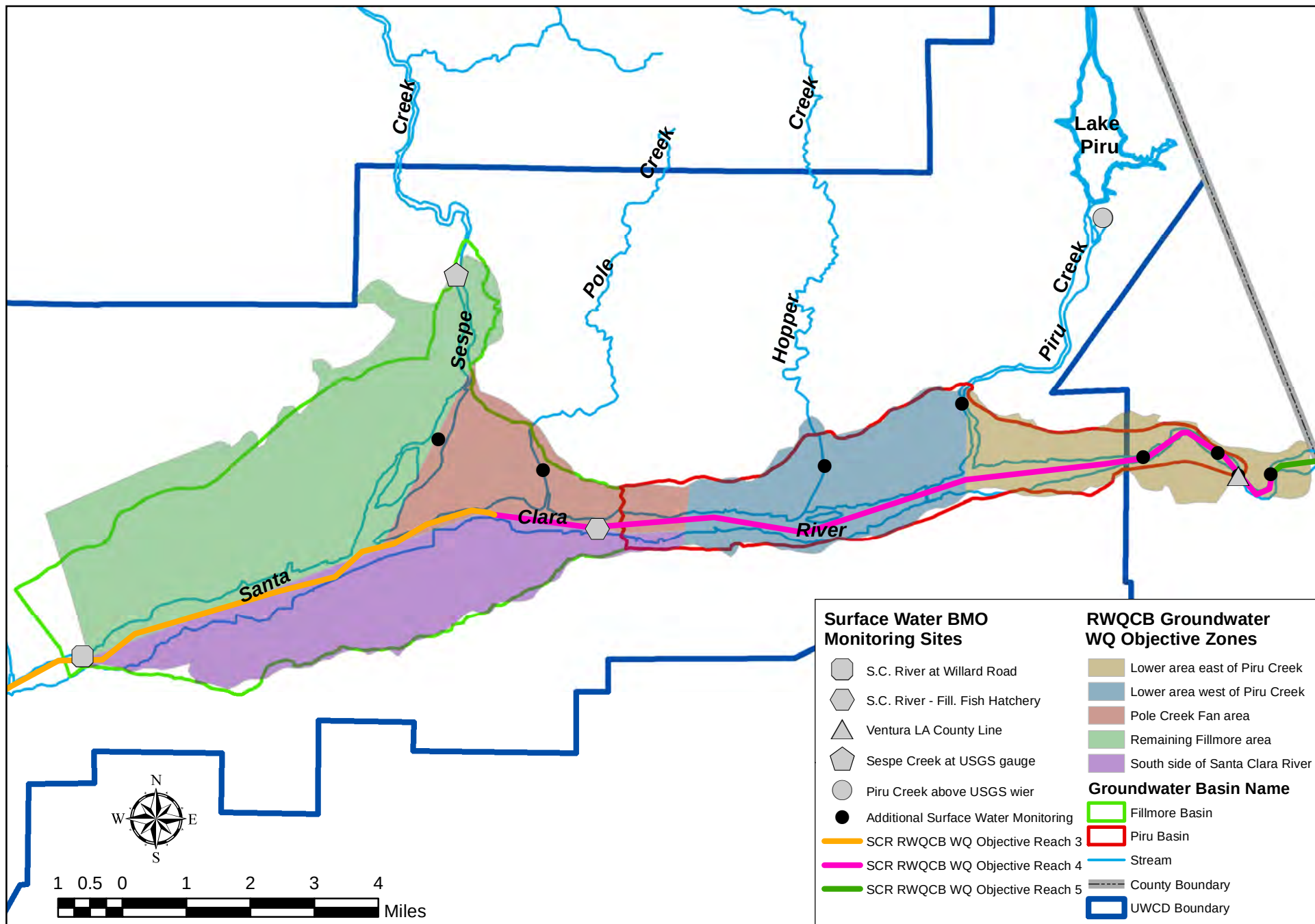
Figure 25. Surface water quality monitoring locations and Regional Water Quality Control Board Santa Clara River reaches; and Regional Water Quality Control Board groundwater quality objective zones map.
