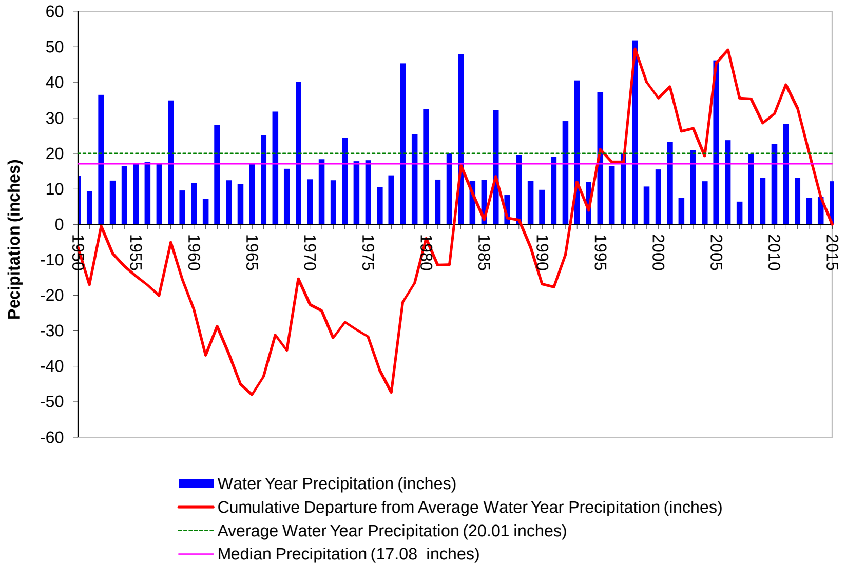
Figure 8. Piru basin historical annual precipitation (Piru-Temescal gauge; Data from Ventura County Watershed Protection District and United Water Conservation District).
