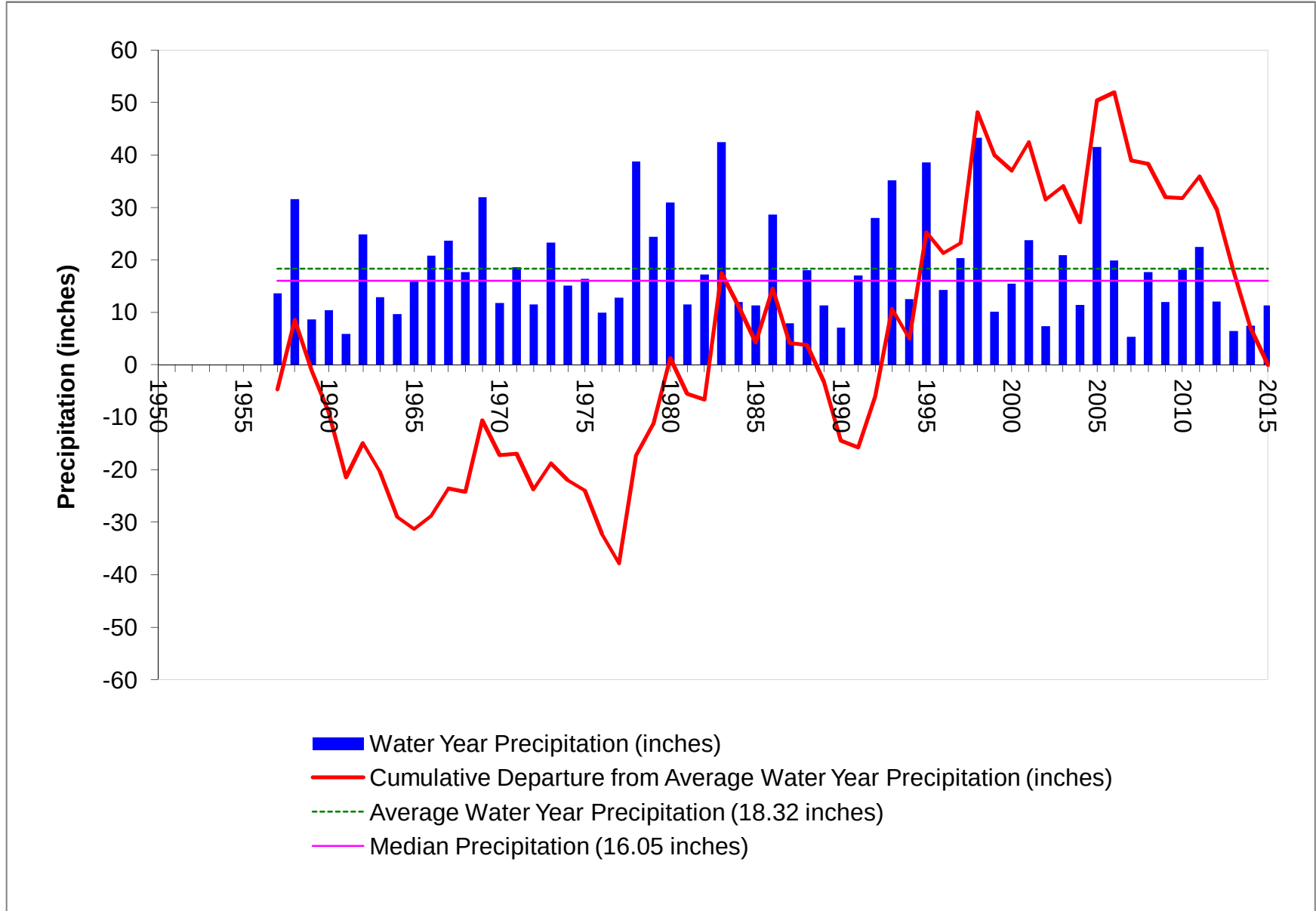
Figure 9. Fillmore basin historical annual precipitation (Fillmore Fish Hatchery Gauge; Data from Ventura County Watershed Protection District).
