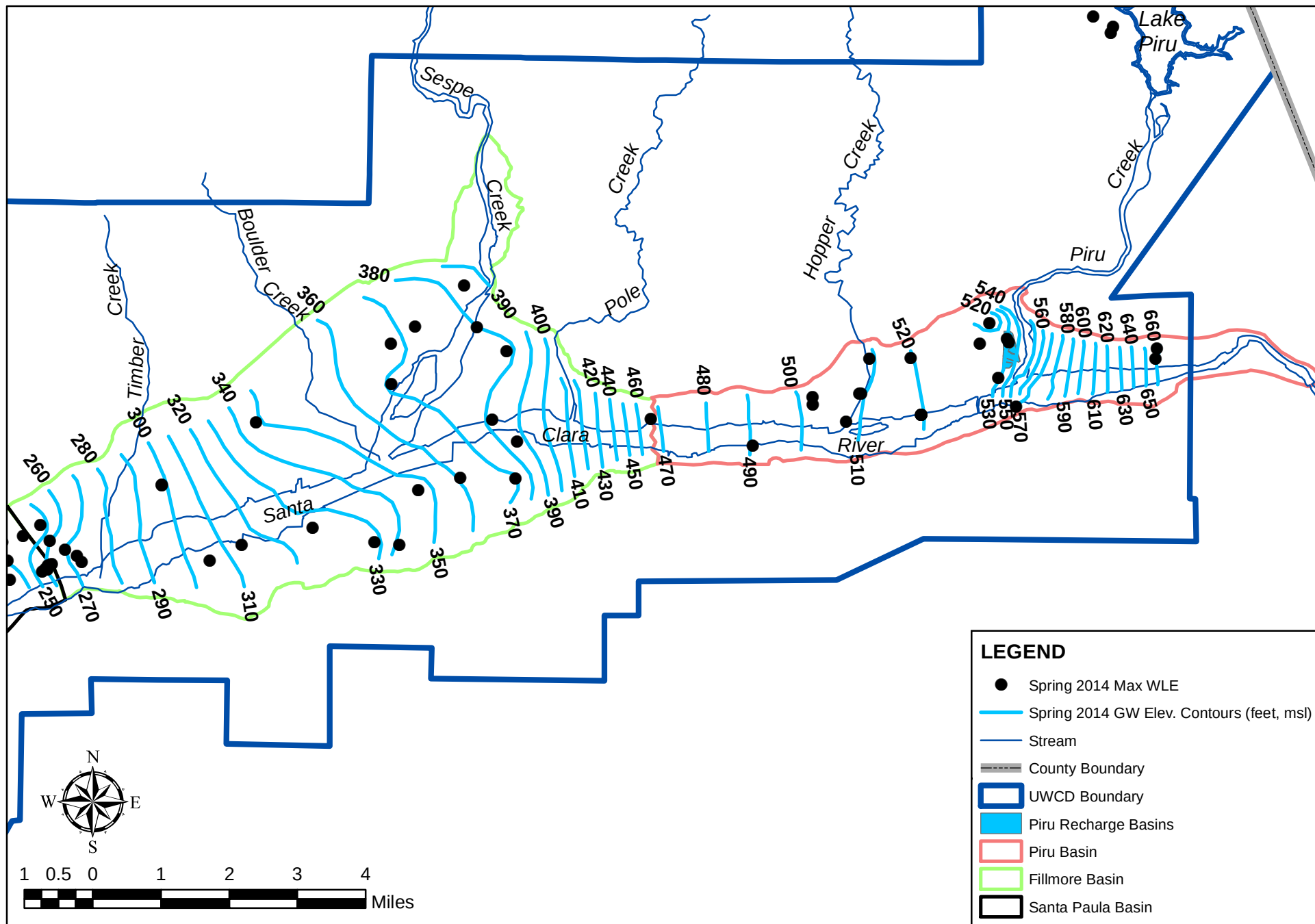
Figure 3. Spring 2014 groundwater elevation contours.
