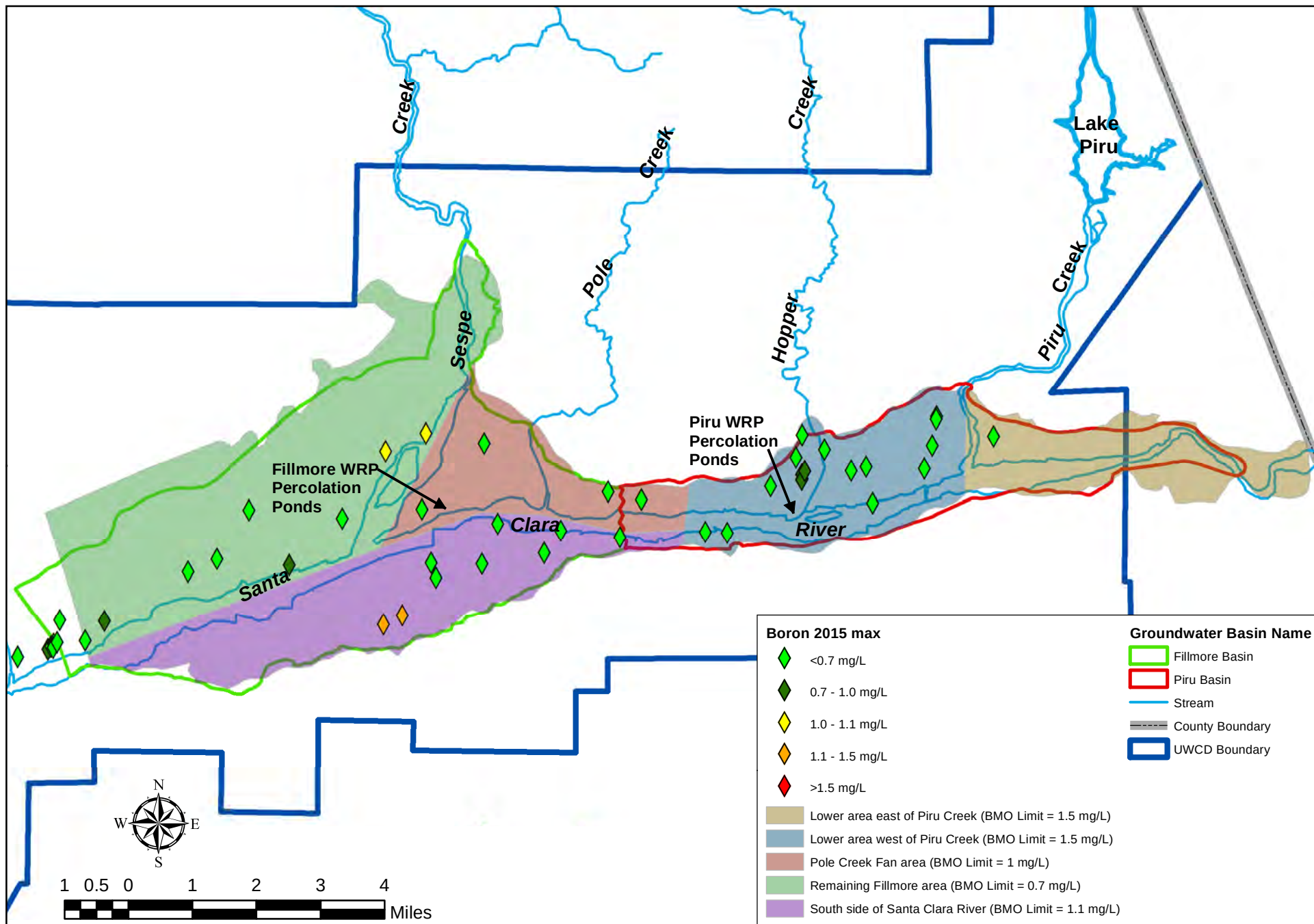
Figure 35. Boron groundwater quality map of 2015 maximum concentrations (mg/L). BMOs are generally based on the groundwater quality objectives identified by the Los Angeles Regional Water Quality Control Board Basin Plan, 1994 (except for in the Piru basin east of Piru Creek).
