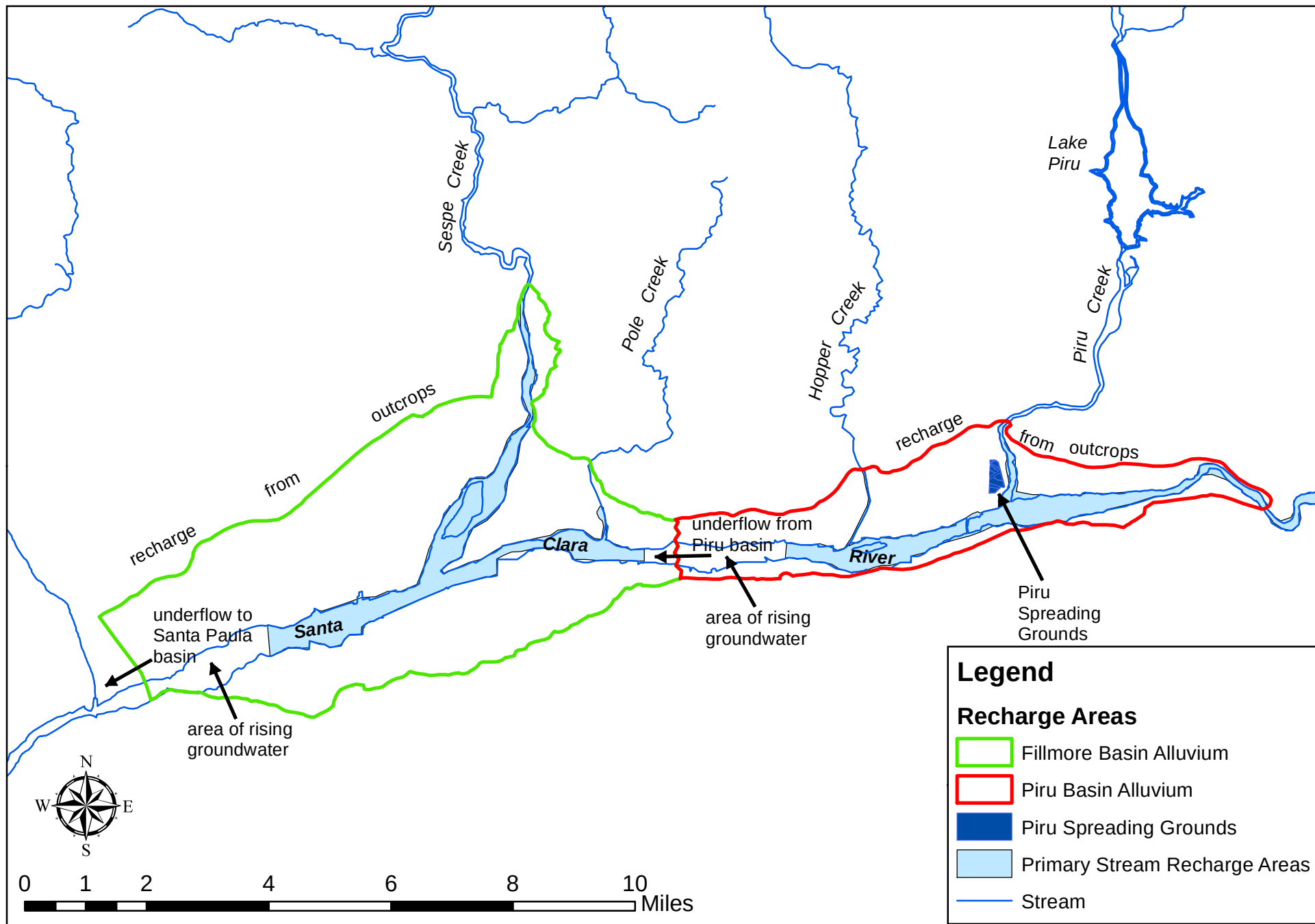
Figure 7. Groundwater recharge areas.
