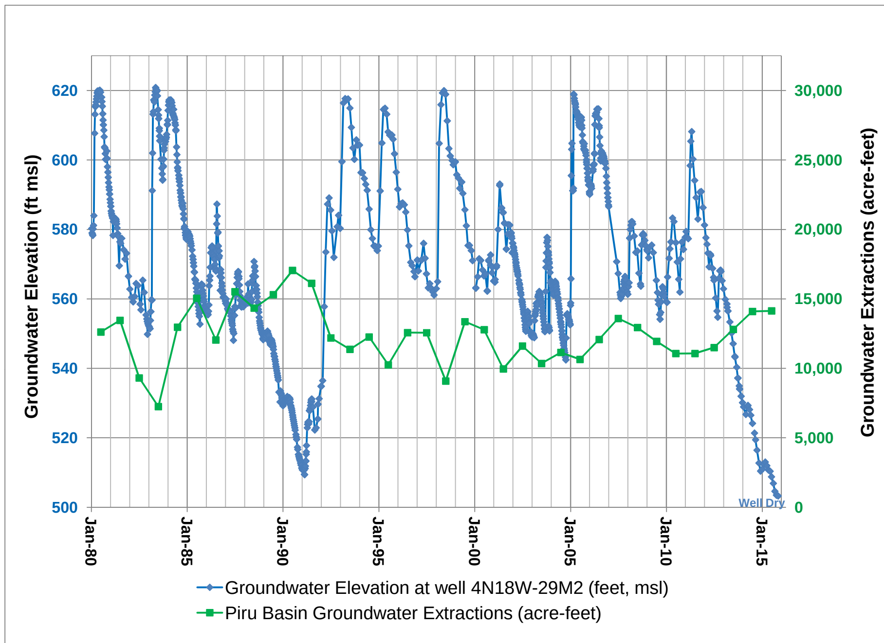
Figure 21. Historical annual groundwater elevations and extractions for the Piru basin.
