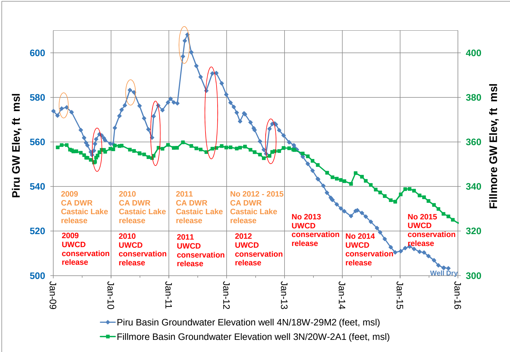
Figure 12. Piru basin and Fillmore basin groundwater levels response to United Water conservation releases and CA DWR Castaic Lake releases.
