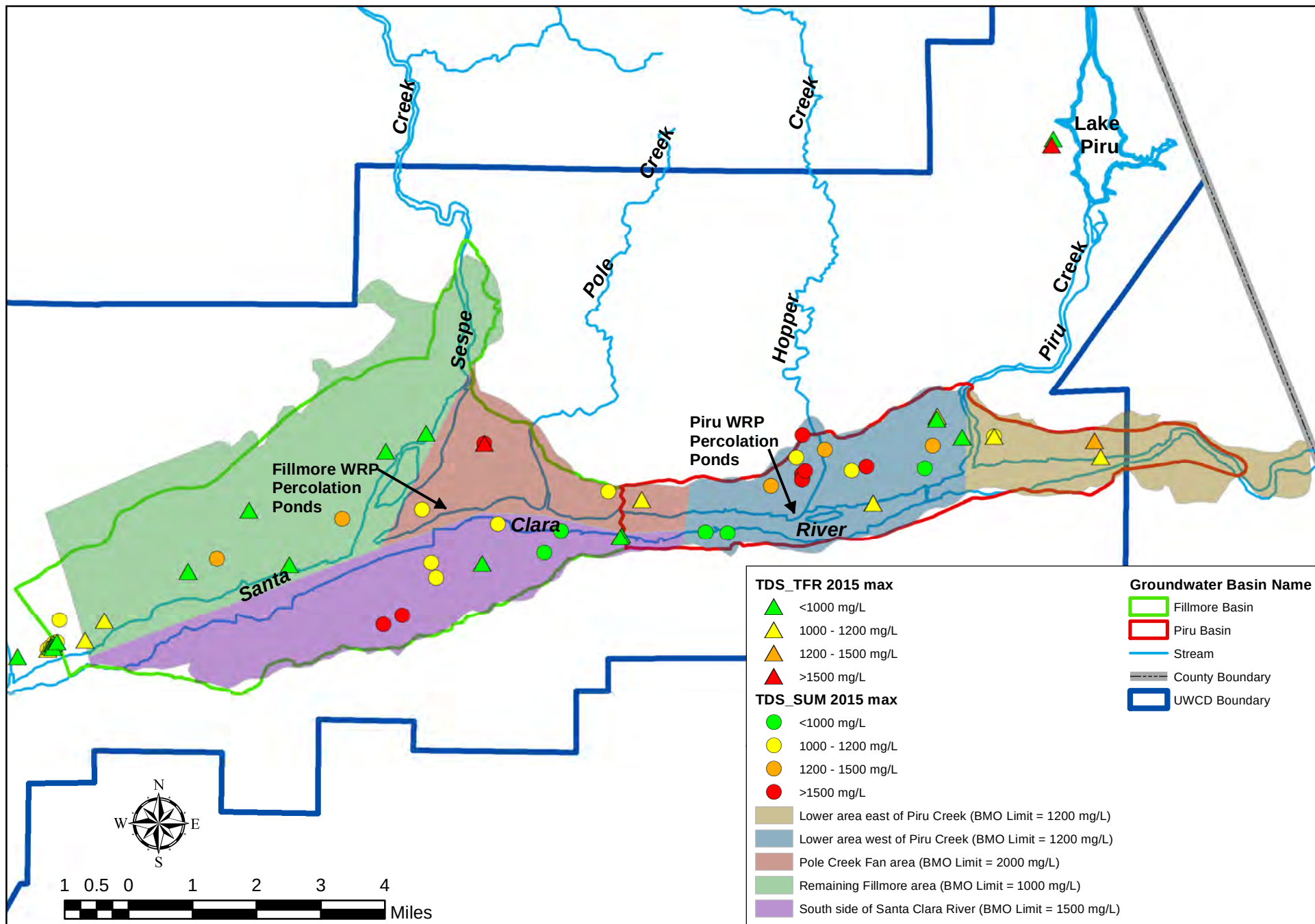
Figure 31. TDS groundwater quality map of 2015 maximum concentrations (mg/L). BMOs are generally based on the groundwater quality objectives identified by the Los Angeles Regional Water Quality Control Board Basin Plan, 1994 (except for in the Piru basin east of Piru Creek).
