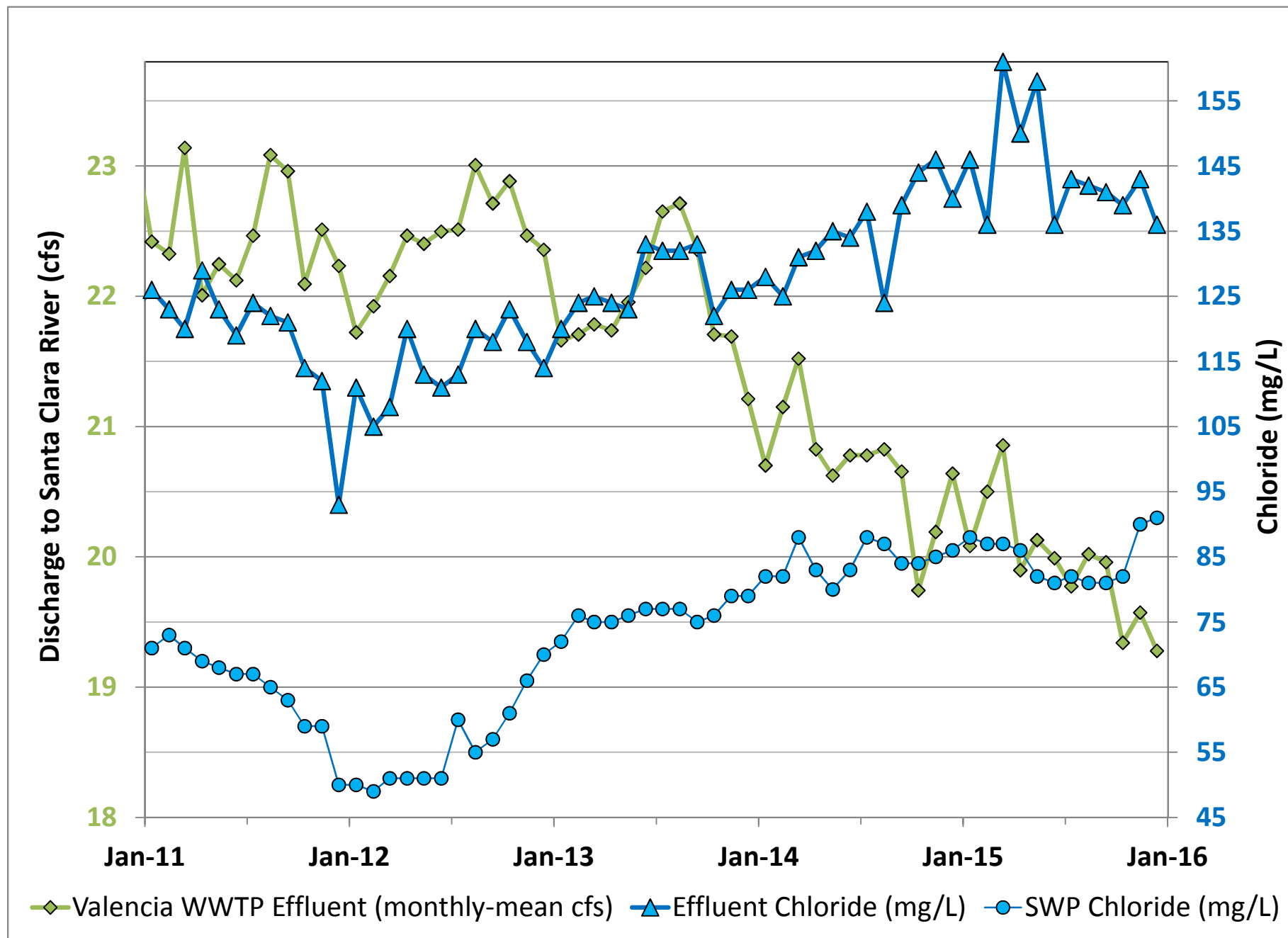
Figure 42. Valencia Wastewater Treatment Plant effluent (NPDES) and chloride concentration discharge to Santa Clara River; State Water Project chloride concentration.
