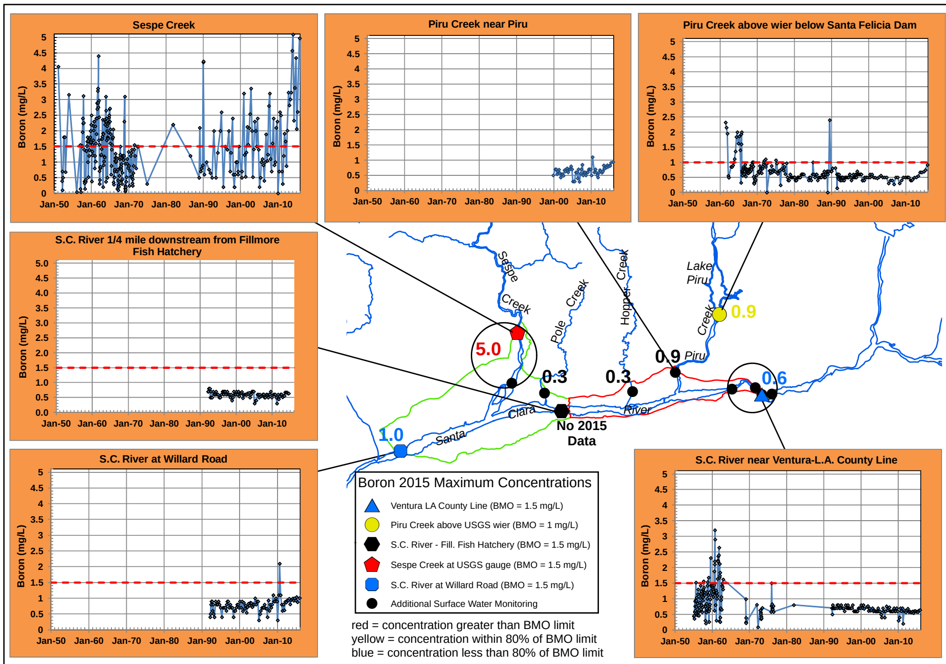
Figure 30. Boron surface water quality time series graphs with map of 2015 maximum concentrations in mg/L (black circles denote alternate sample sites); dashed red line is the BMO based on surface water quality objectives from the RWQCB-LA Basin Plan, 1994.
