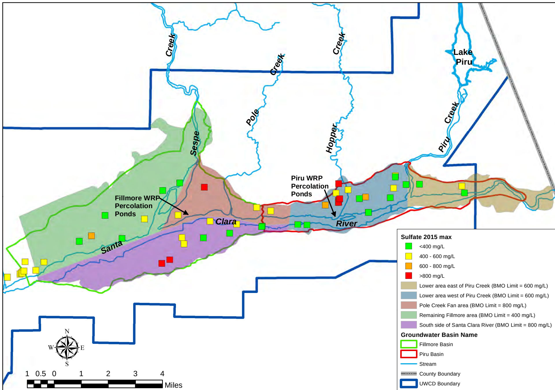
Figure 32. Sulfate groundwater quality map of 2015 maximum concentrations (mg/L). BMOs are generally based on the groundwater quality objectives identified by the Los Angeles Regional Water Quality Control Board Basin Plan, 1994 (except for in the Piru basin east of Piru Creek).
