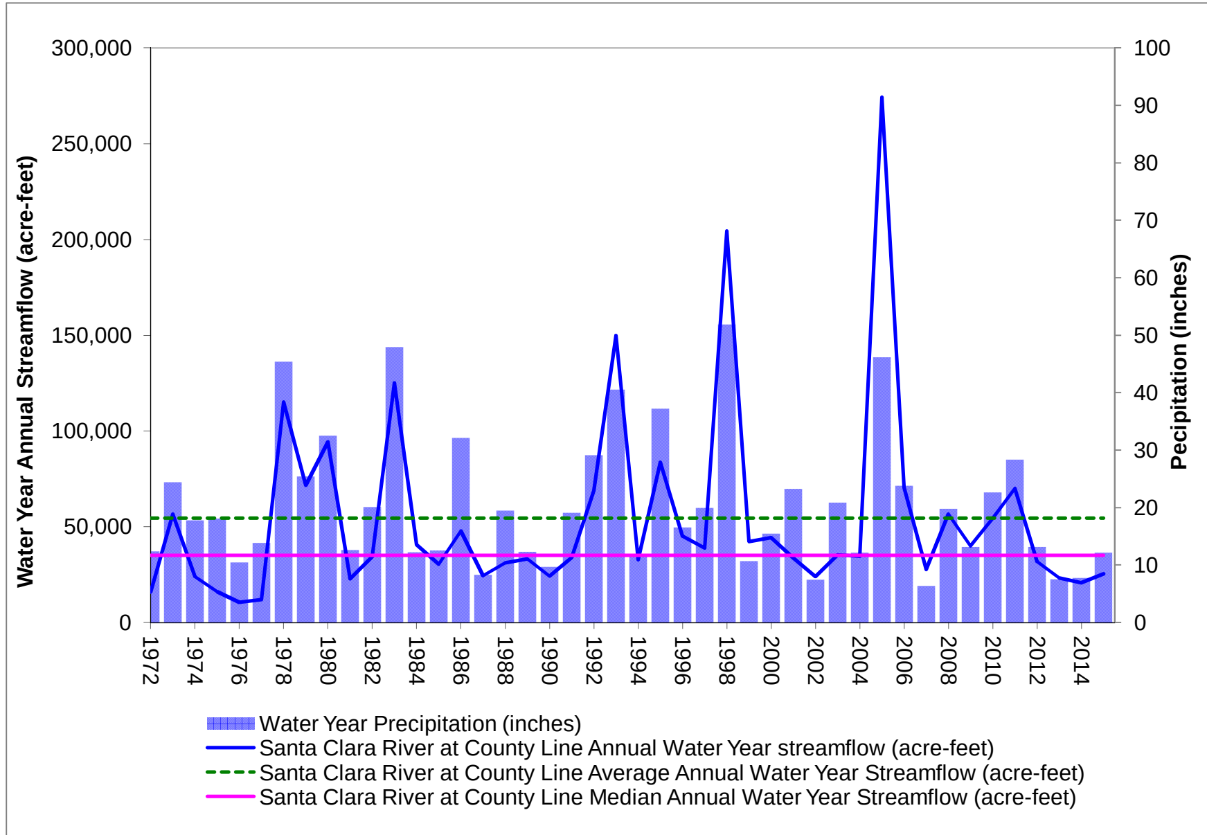
Figure 10. Santa Clara River historical annual streamflow near Ventura/L.A County Line and Piru basin precipitation (streamflow data from USGS).
