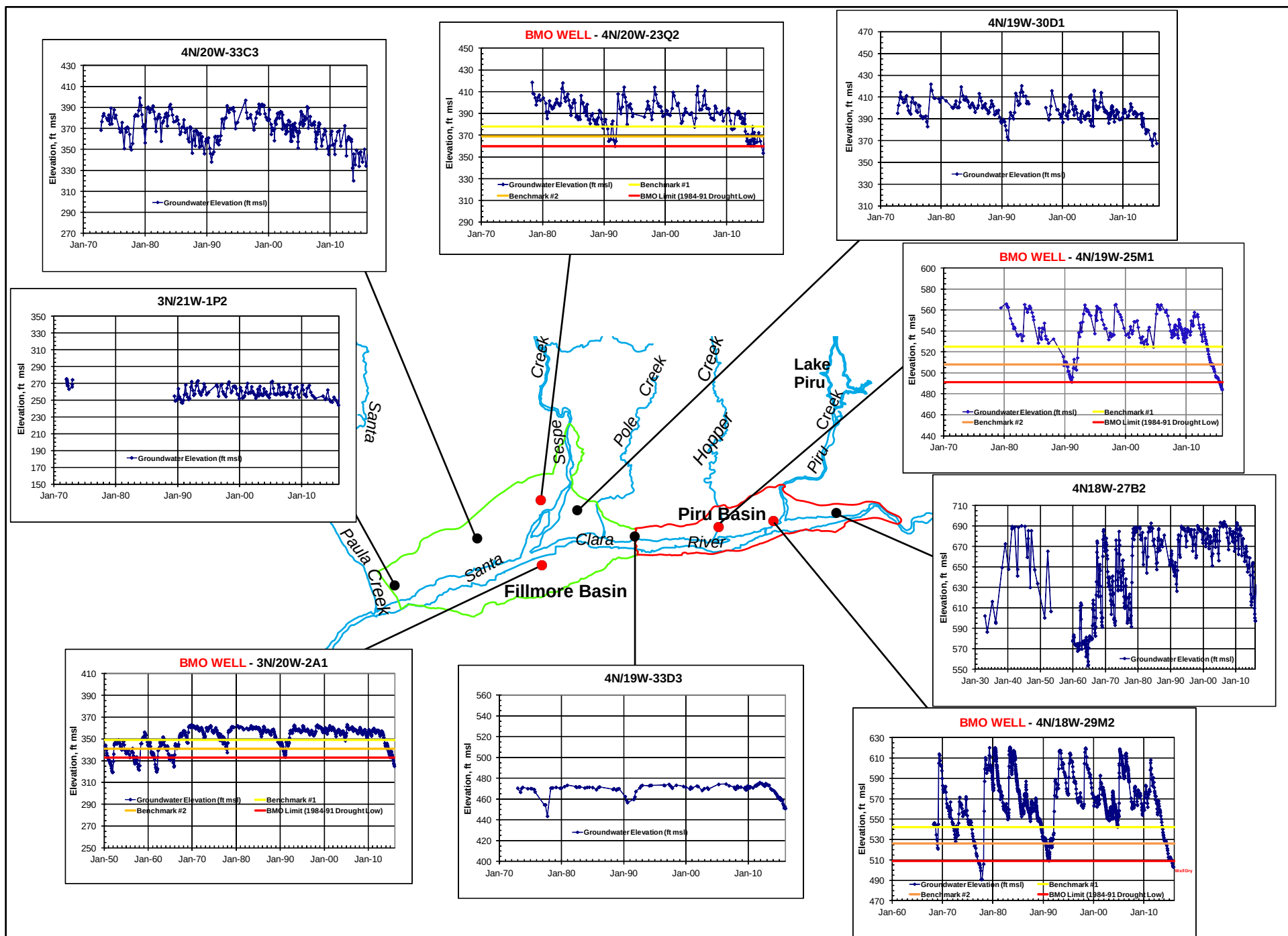
Figure 18. Groundwater elevation hydrographs.
