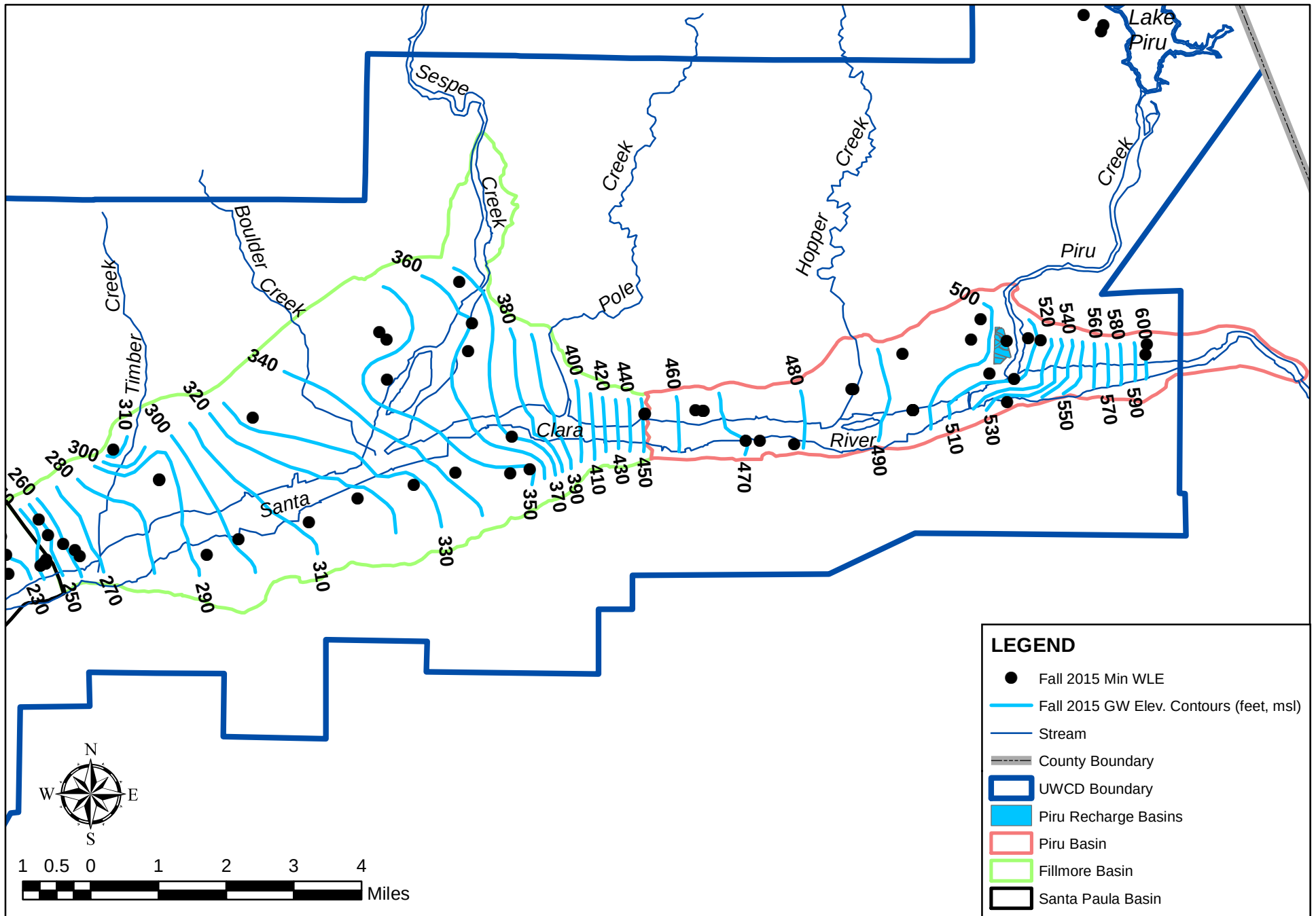
Figure 6. Fall 2015 groundwater elevation contours.
