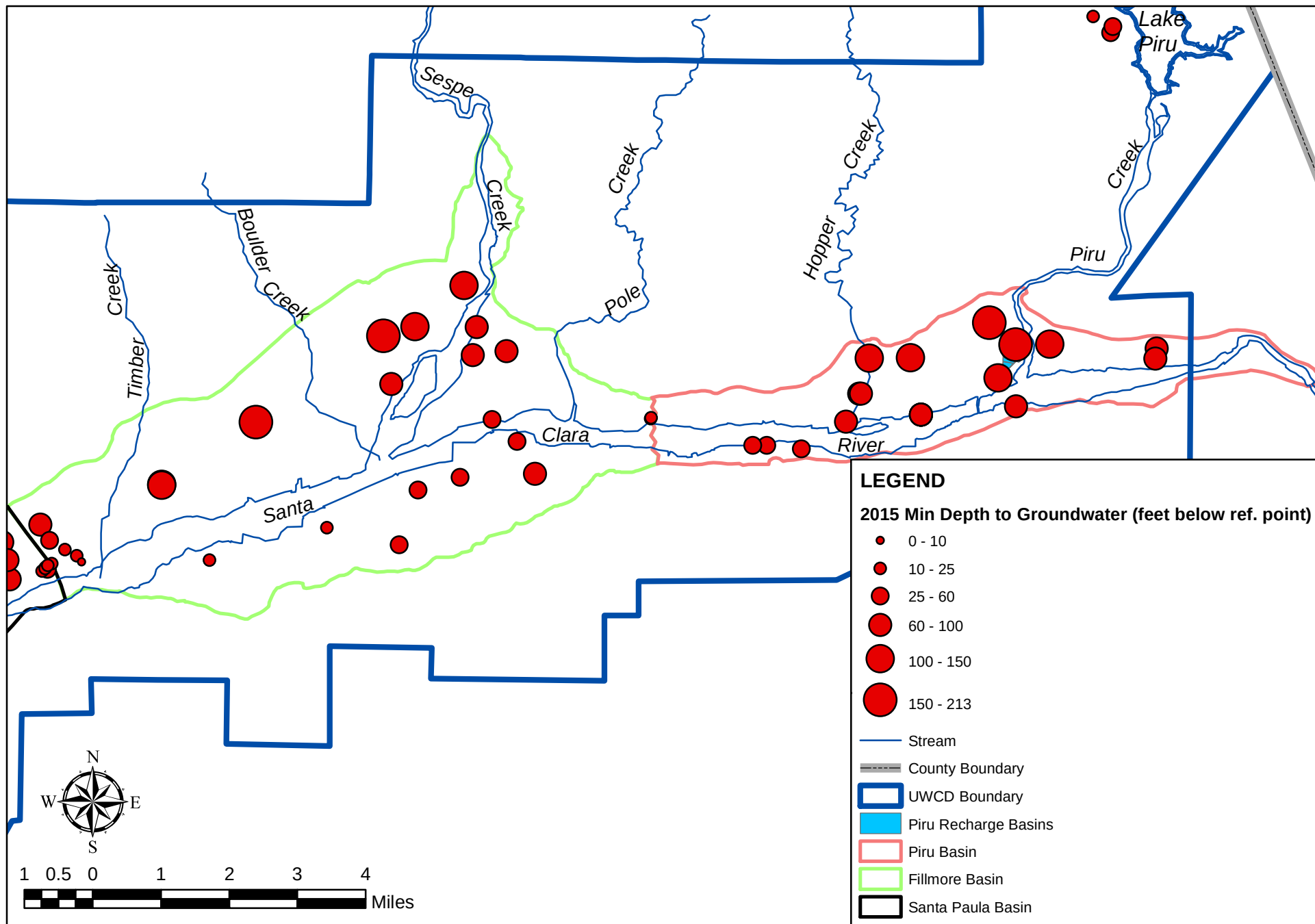
Figure 24. Spring 2015 depth to groundwater.
