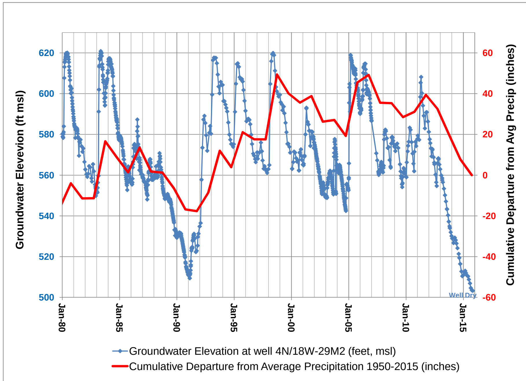
Figure 19. Groundwater elevations and cumulative departure from average precipitation for the Piru basin.
