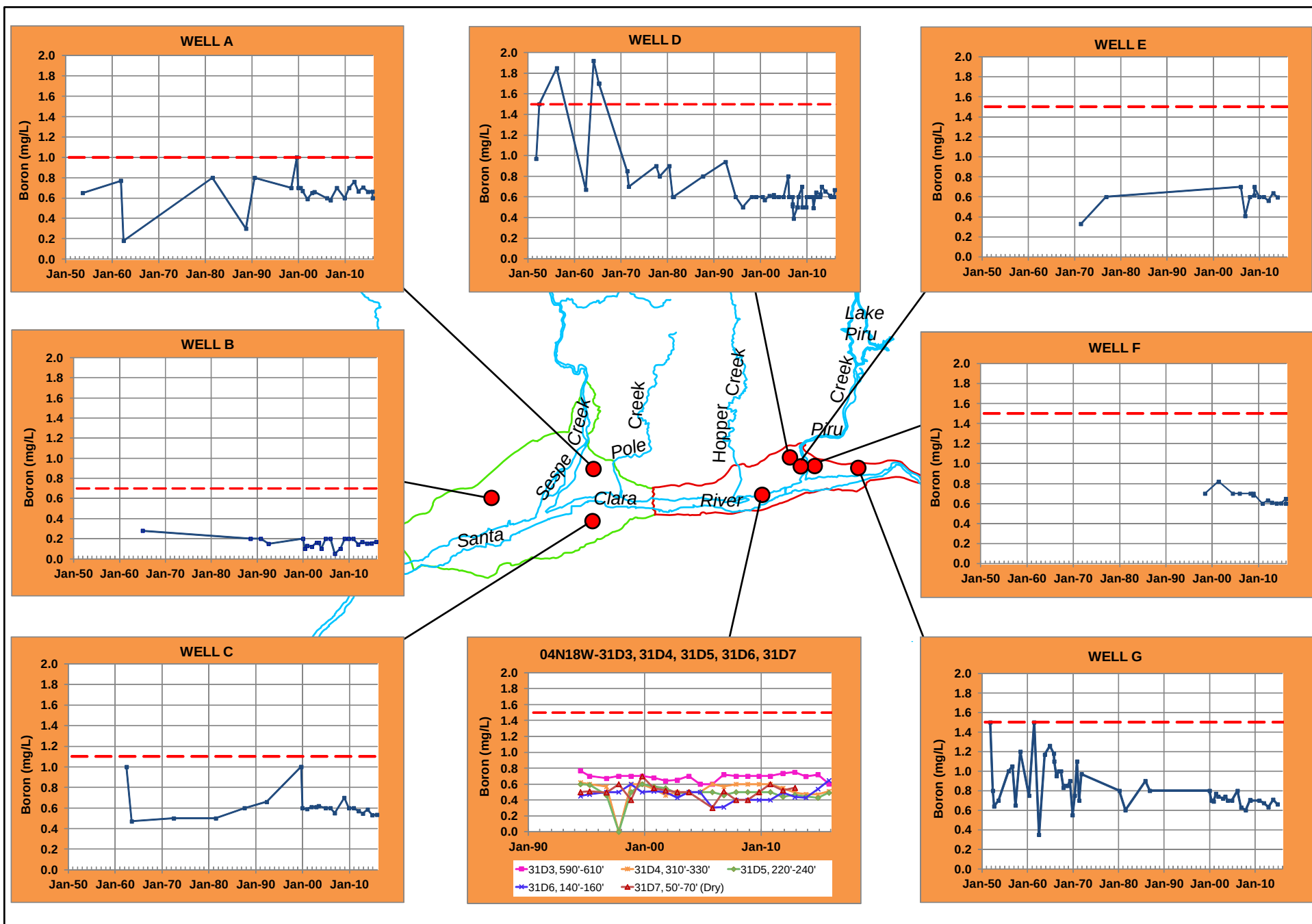
Figure 40. Boron groundwater quality time series graphs (mg/L); dashed red line is the BMO.
