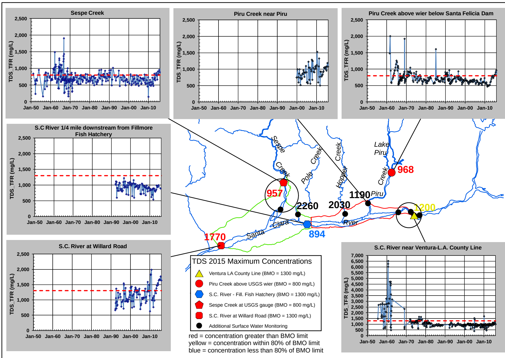
Figure 26. TDS surface water quality time series graphs with map of 2015 maximum concentrations in mg/L (black circles denote alternate sample sites); dashed red line is the BMO based on surface water quality objectives from the RWQCB-LA Basin Plan, 1994.
