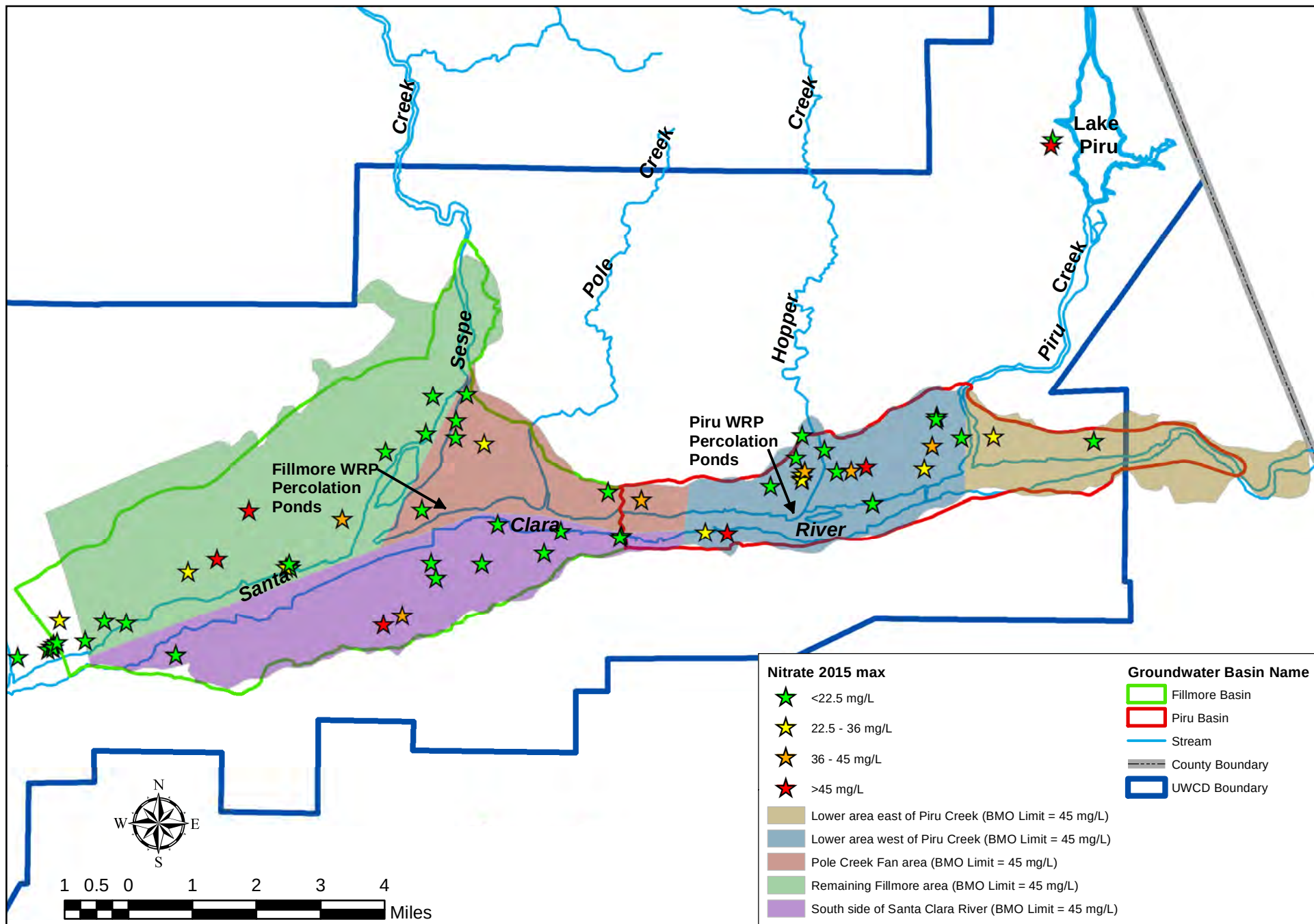
Figure 34. Nitrate groundwater quality map of 2015 maximum concentrations (mg/L). BMOs are generally based on the groundwater quality objectives identified by the Los Angeles Regional Water Quality Control Board Basin Plan, 1994 (except for in the Piru basin east of Piru Creek).
