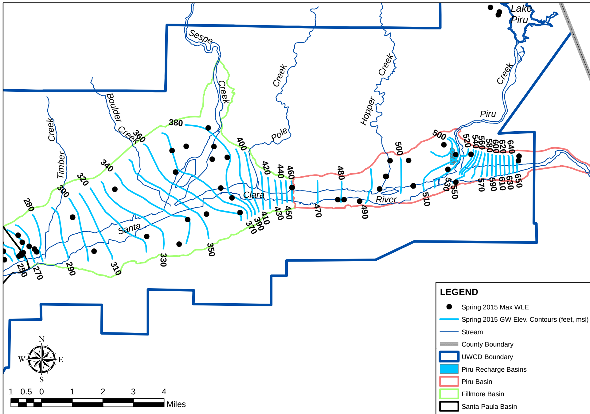
Figure 5. Spring 2015 groundwater elevation contours.
