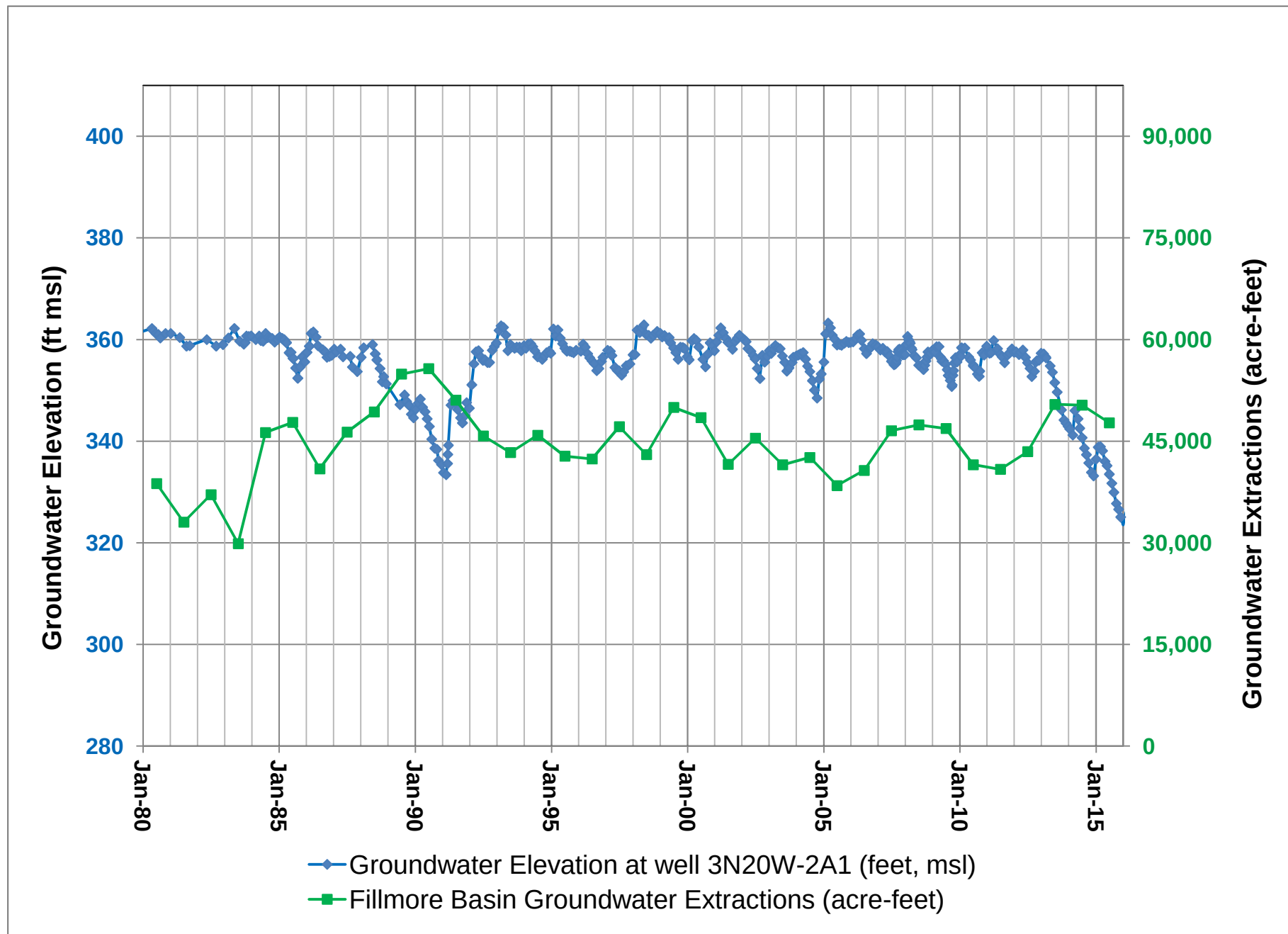
Figure 22. Historical annual groundwater elevations and extractions for the Fillmore basin.
