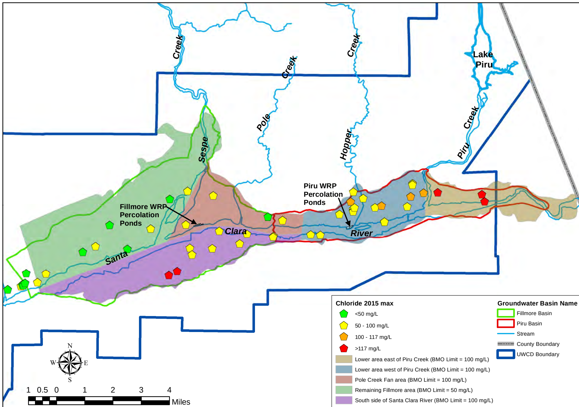
Figure 33. Chloride groundwater quality map of 2015 maximum concentrations (mg/L). BMOs are generally based on the groundwater quality objectives identified by the Los Angeles Regional Water Quality Control Board Basin Plan, 1994 (except for in the Piru basin east of Piru Creek).
