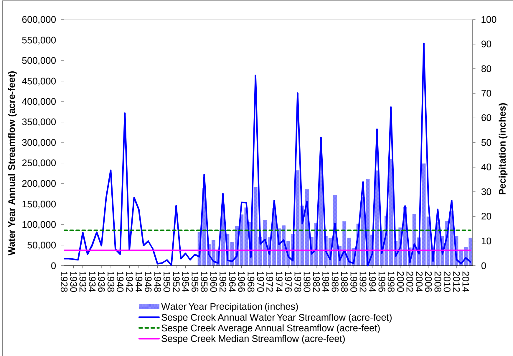
Figure 11. Sespe Creek historical annual streamflow and Fillmore basin precipitation (streamflow data from USGS and VCWPD).
