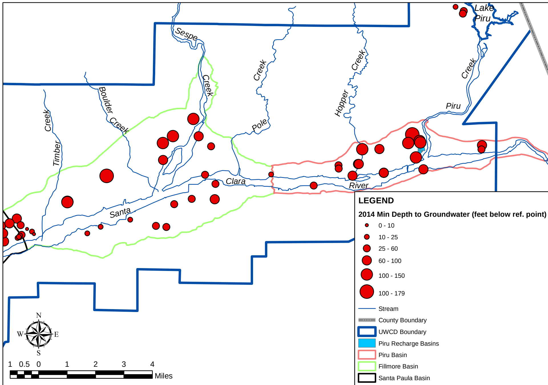
Figure 23. Spring 2014 depth to groundwater.
