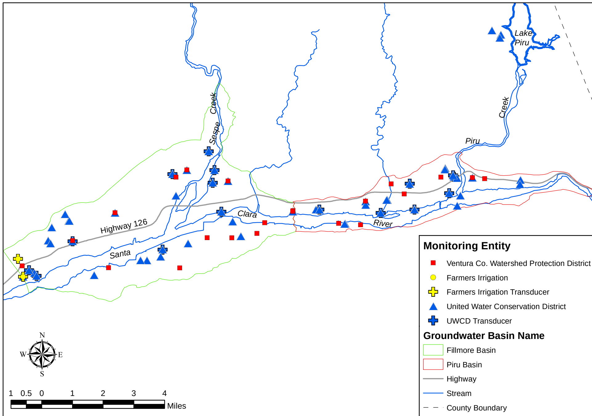
Figure 17. Locations of wells monitored for groundwater elevations in 2014 and/or 2015 within Piru basin and Fillmore basin.
