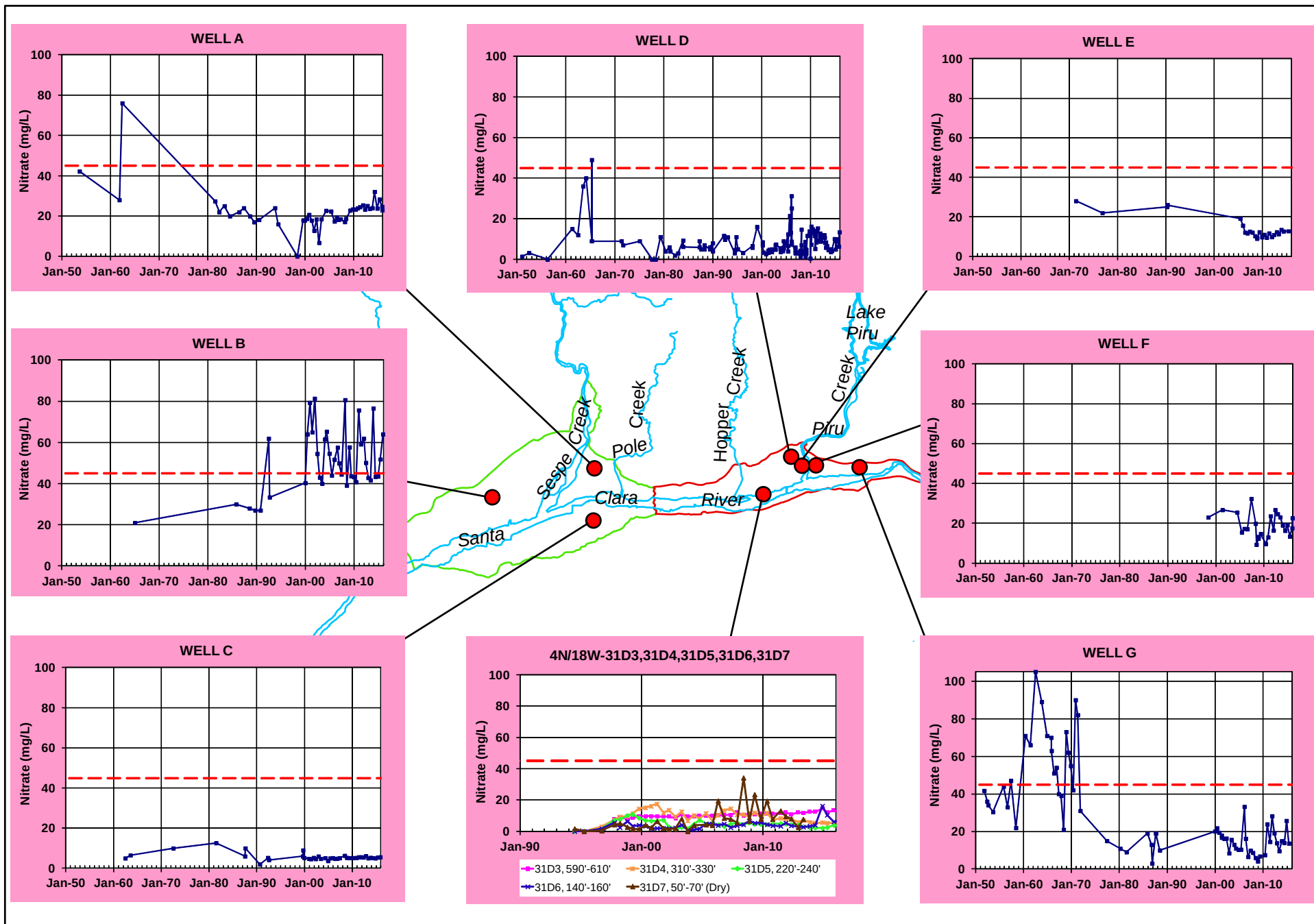
Figure 39. Nitrate groundwater quality time series graphs (mg/L); dashed red line is the BMO.
