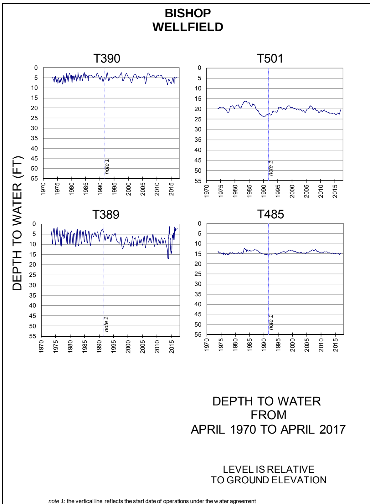
Figure 2. 3. Depth to Water Hydrographs for Bishop Wellfield
